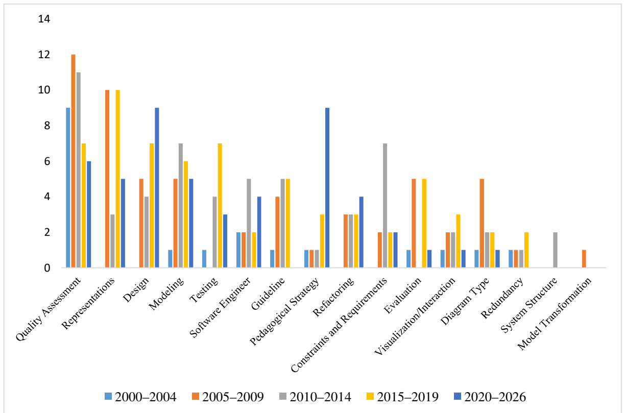
Figure 3: Topic Trends.
