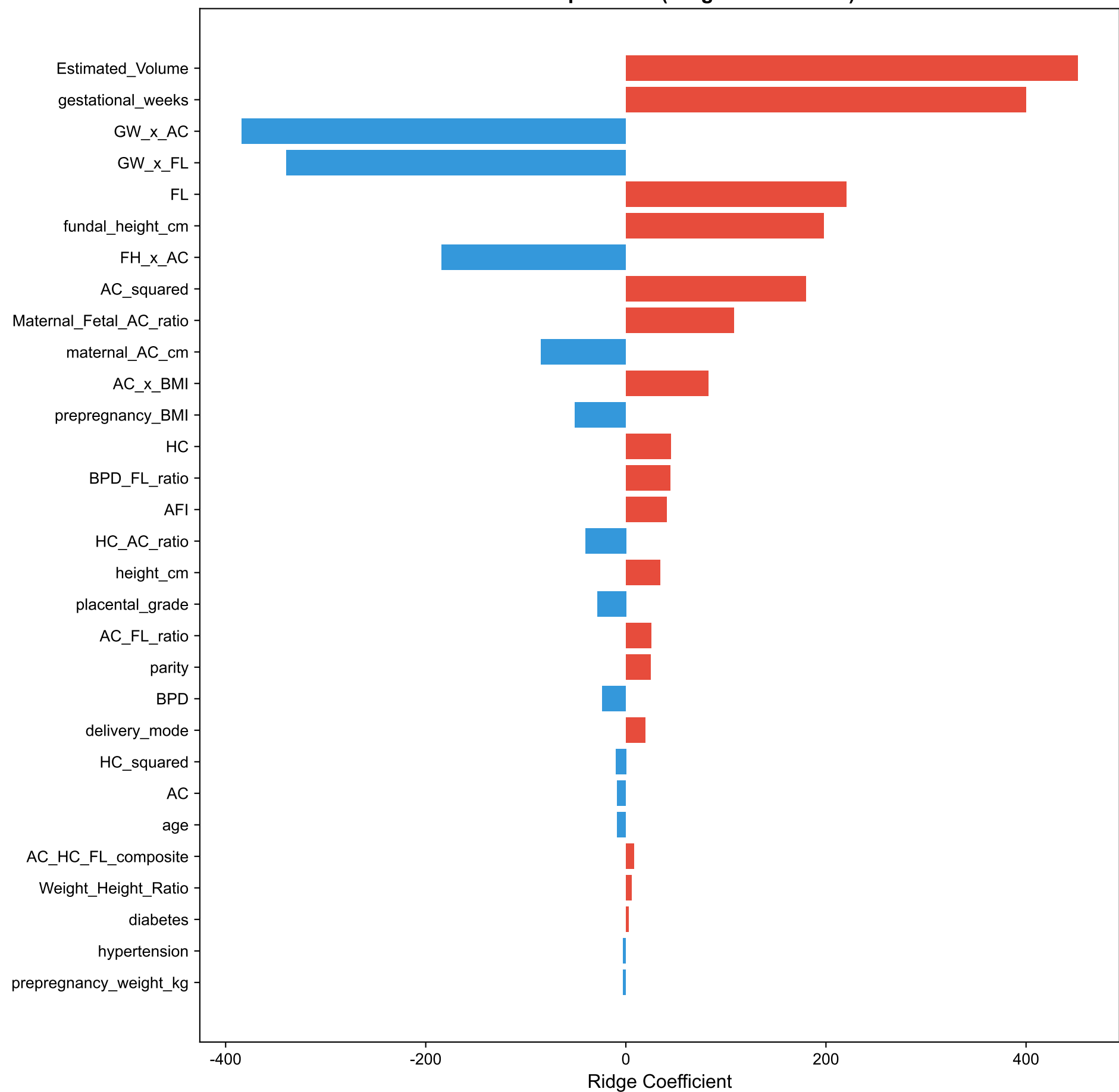
Feature Importance (Ridge Coefficients)
