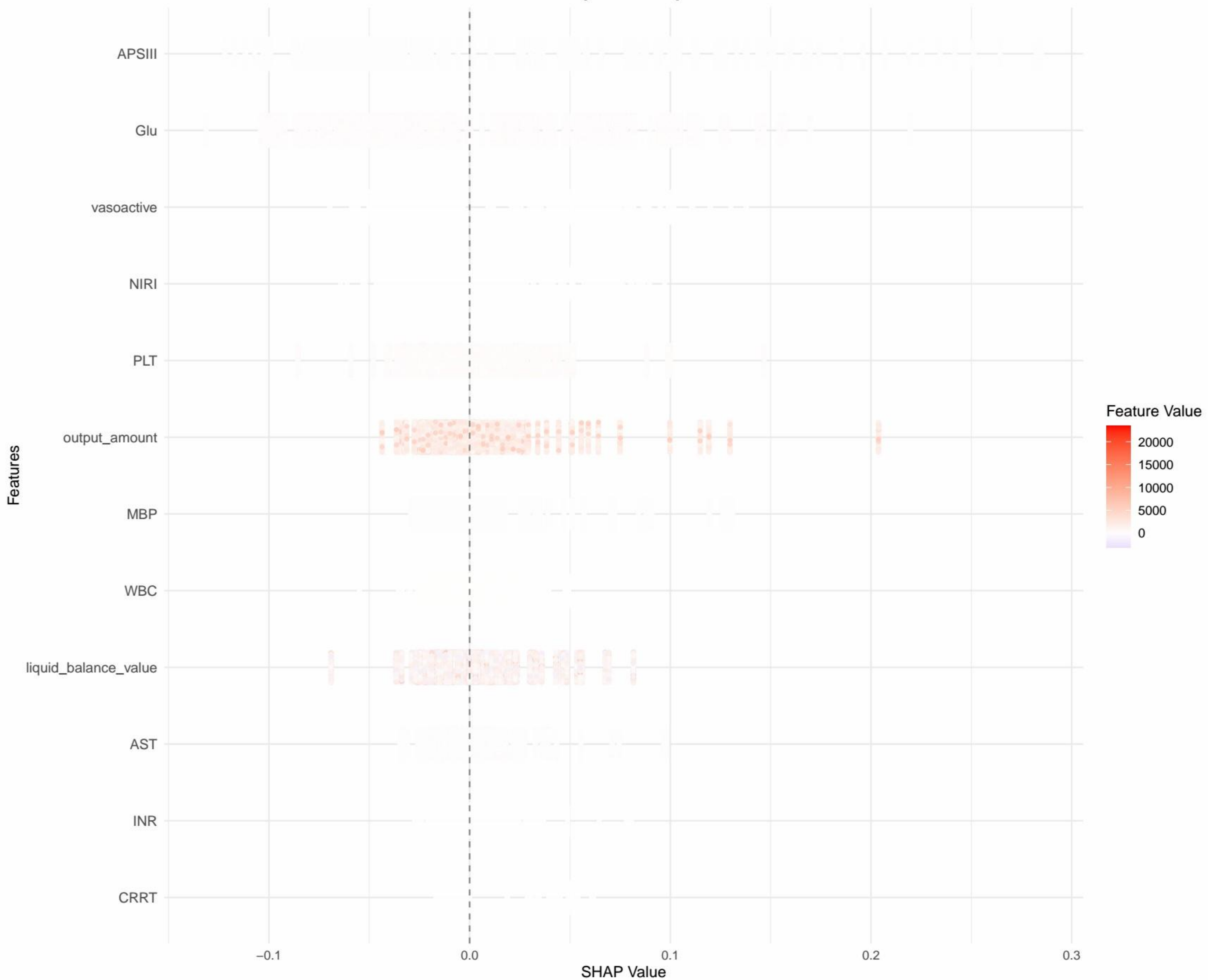
SHAP Summary Plot – Top 20 Features
