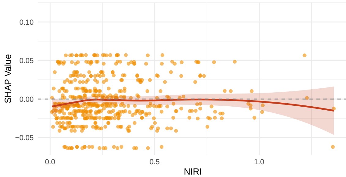
SHAP Dependence Plot: NIRI
