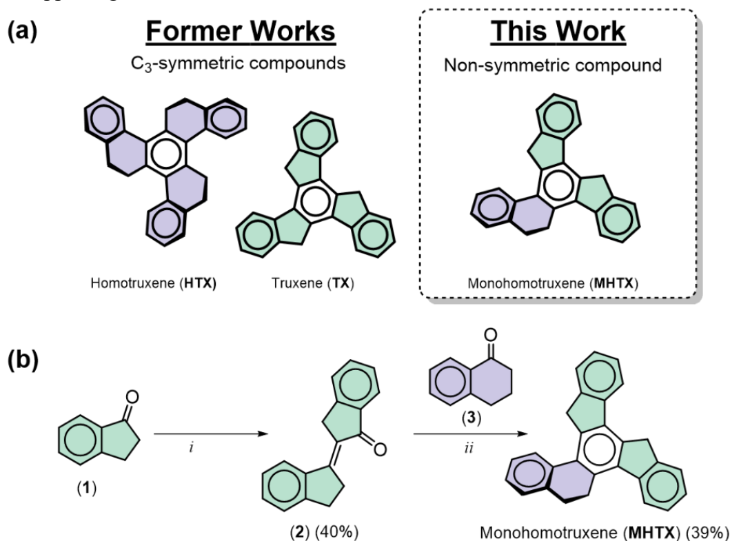
Figure 1. Structure and synthetic route of MHTX. (a) Molecular structures of homotraxene ( HTX ) 16,24 , truxene ( TX ) 28 and the novel non-symmetric MHTX reported in this work. (b) Synthetic route to MHTX : (i) TiCl 4 , triethylamine, dichloromethane, hexane, 16 hours at room temperature under argon; (ii) para -toluenesulfonic acid, propionic acid, ortho -dichlorobenzene, 24 hours at 140 °C under argon in the dark
