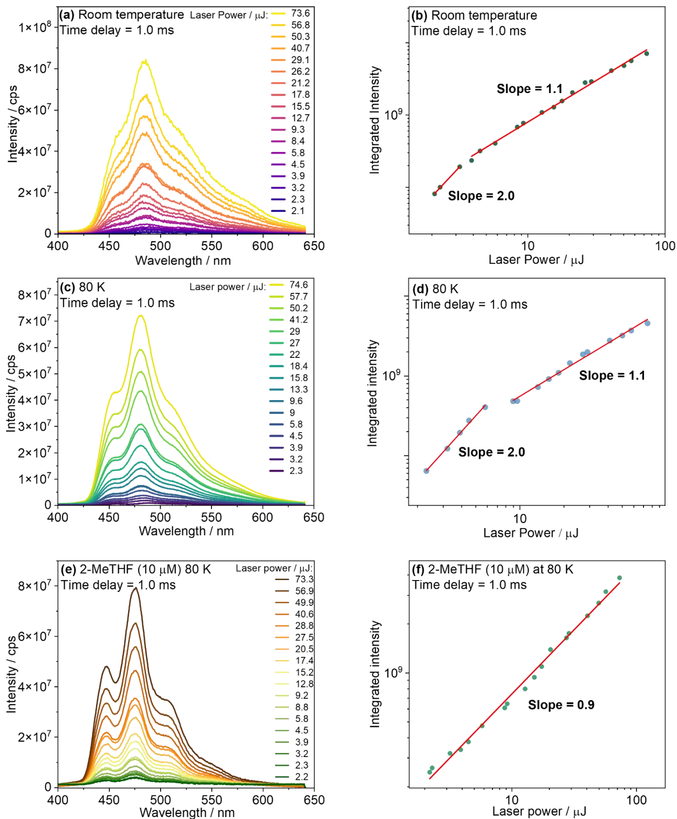
Extended Data Figure 3. Time-resolved photoluminescence spectra (left column) and power-dependent plots (right column) of MHTX under vacuum ( \lambda_{\text{Ex}} = 337 \text{ nm} ) and different conditions: (a) and (b) measurement at 298 K for a 1 wt.% Zeonex drop-cast film; (c) and (d) at 80 K for a 1 wt.% Zeonex drop-cast film. (e) and (f) at 80 K for a 10 \mu\text{M} solution in 2-MeTHF. The time-resolved spectra were collected with a time delay (TD) of 1.0 ms and an integration window of 10 ms.
