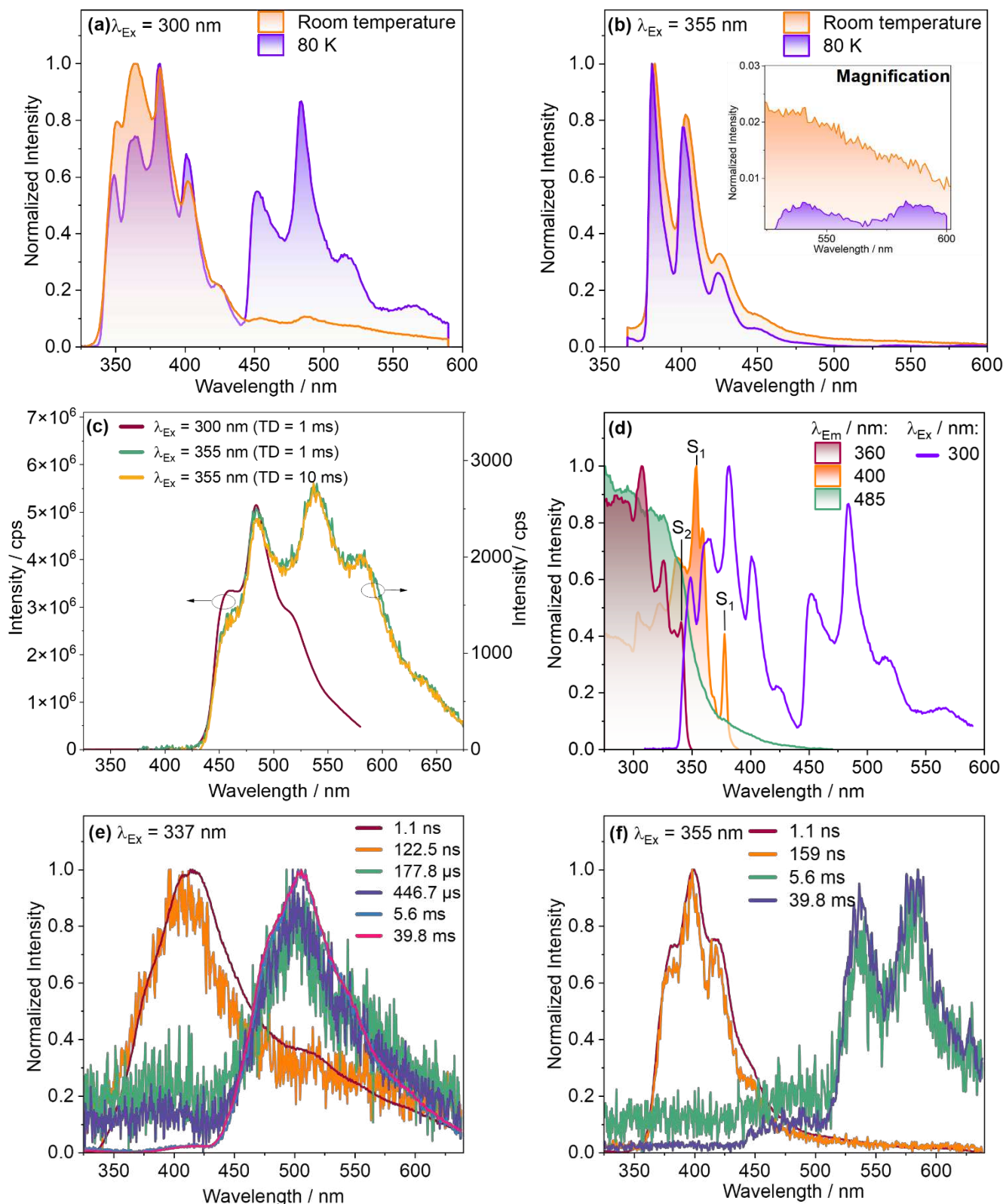
Figure 3. Temperature- and time-dependent photoluminescence of MHTX. (a–b) Normalized steady-state emission of MHTX (1 wt.% in Zeonex) at room temperature (orange area) and 80 K (purple area) upon excitation at (a) 300 nm and (b) 355 nm. (c) Emission spectra at different time delays upon excitation at 300 nm (red line, left y-axis) and 355 nm (orange and green lines, right y-axis) at 80 K. (d) Combined emission and excitation spectra recorded at different emission wavelengths ( \lambda_{Em} ), highlighting the exclusion of S_1 vibrational bands (labeled) when monitoring high-energy phosphorescence. (e–f) Time-gated emission spectra at 80 K recorded at the indicated time delays following excitation at (e) 337 nm (0.5 wt.% in Zeonex) and (f) 355 nm (0.1 wt.% in Zeonex).
