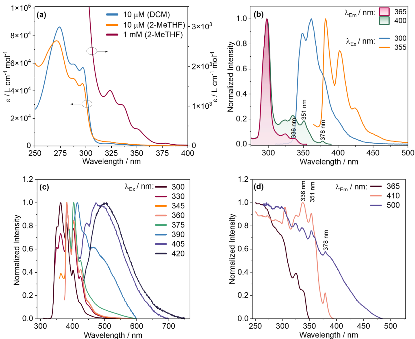
Figure 2. Steady-state photoluminescence and excitation profiles of MHTX at room temperature. (a) Absorption spectra of MHTX in 10 \mu\text{M} solutions in DCM (blue) and 2-MeTHF (orange), and 1 mM solution in 2-MeTHF (dark red). (b) Normalized excitation and emission spectra in 2-MeTHF (10 \mu\text{M} ). (c) Normalized emission spectra of a 1 wt.% drop-cast film in Zeonex under different excitation wavelengths in the presence of molecular oxygen. (d) Normalized excitation spectra under the same conditions as Figure (c).
