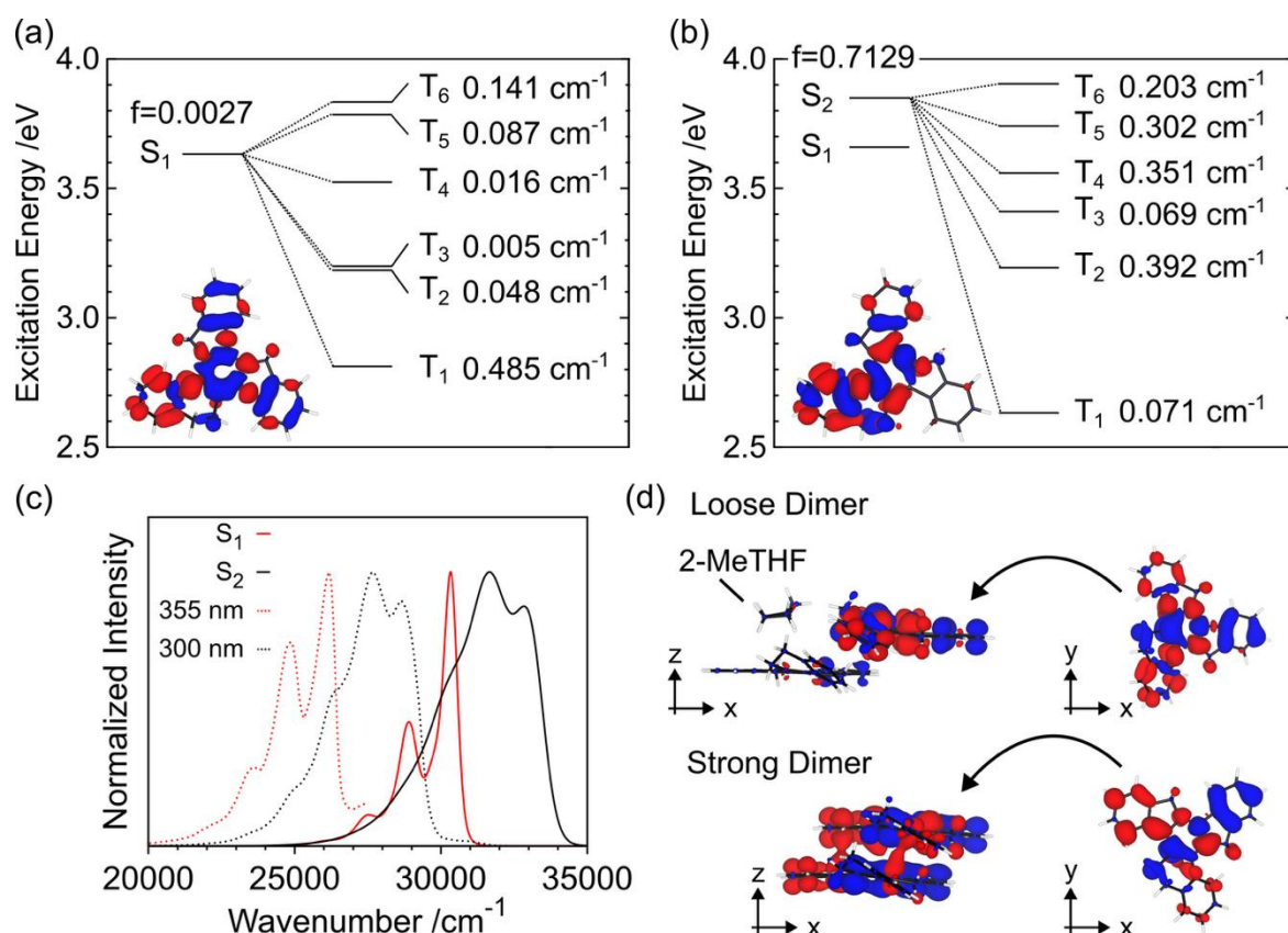
Figure 5. Theoretical calculation on the monomeric and aggregated properties of MHTX. Energy levels of excited states at the (a) S 1 and (b) S 2 optimized structures. Inset shows the electron density difference of S 1 -S 0 and S 2 -S 0 (isosurface value: 5 \times 10^{-4} a.u.). Red and blue regions indicate positive and negative values. Values represent the SOC matrix element between singlets and triplets. f represents the oscillator strength of S 1 -S 0 and S 2 -S 0 . (c) Calculated S 1 and S 2 fluorescence spectra (solid lines), compared with the experimental spectra under 355 nm and 300 nm excitations (Fig. 2b). The density of final vibronic states is expressed using the Gaussian function with a linewidth of 100\text{ cm}^{-1} . (d) Electron density difference between S 1 and S 0 at the S 0 optimized structure for the loose and strong dimers (isosurface value: 5 \times 10^{-4} a.u.).
