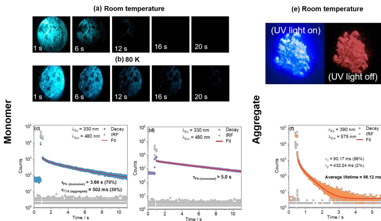
Figure 4. Long-lived luminescence of MHTX . (a–b) Photos showing the persistent cyan luminescence of a film of 1 wt.% MHTX in Zeonex after the removal of the excitation source ( \lambda_{\text{Ex}} = 337 nm) at (a) room temperature and (b) 80 K. (c–d) Time-resolved luminescence decay profiles recorded via TCSPC (11 s time window) for (c) 1 wt.% MHTX in Zeonex at 80 K and (d) a 10 \mu\text{M} solution of MHTX in 2-MeTHF at 80 K ( \lambda_{\text{Ex}} = 330 nm, \lambda_{\text{Em}} = 480 nm). The red solid lines are numerical fits and the gray dots are the instrument response function (IRF). (e) Photos of MHTX powder at room temperature under UV irradiation ( \lambda_{\text{Ex}} = 365 nm, left) and after the excitation source is turned off (right), showing the orange luminescence. (f) Time-resolved luminescence decay profile of the aggregate emission recorded for 1 wt.% MHTX in Zeonex ( \lambda_{\text{Ex}} = 390 nm, \lambda_{\text{Em}} = 575 nm). The red solid line is the numerical fit and the gray dots are the instrument response function (IRF).
