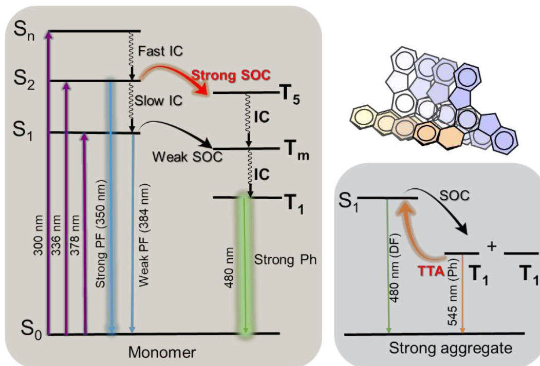
Figure 6. Summary of the excited-state mechanisms of MHTX. Simplified Jablonski diagram summarizing the rich photophysics of monomeric and aggregate species of MHTX .
