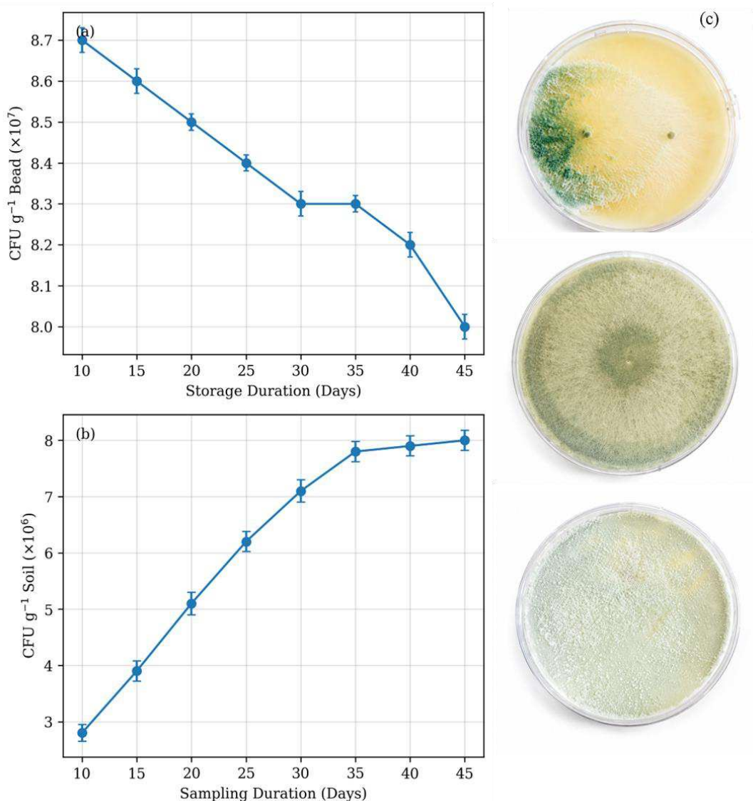
Figure 4. Viability, controlled release behavior, and cultural characteristics of encapsulated Trichoderma longibrachiatum . (a) Storage stability profile showing sustained viability of encapsulated fungal propagules during 45 days of storage, expressed as CFU g -1 bead. (b) Controlled release profile demonstrating gradual diffusion-mediated release of viable spores into soil over 45 days, expressed as CFU g -1 soil. (c) Morphological growth characteristics of released Trichoderma colonies on PDA medium confirming successful recovery and viability of encapsulated fungal spores after release from the hydrogel matrix.
