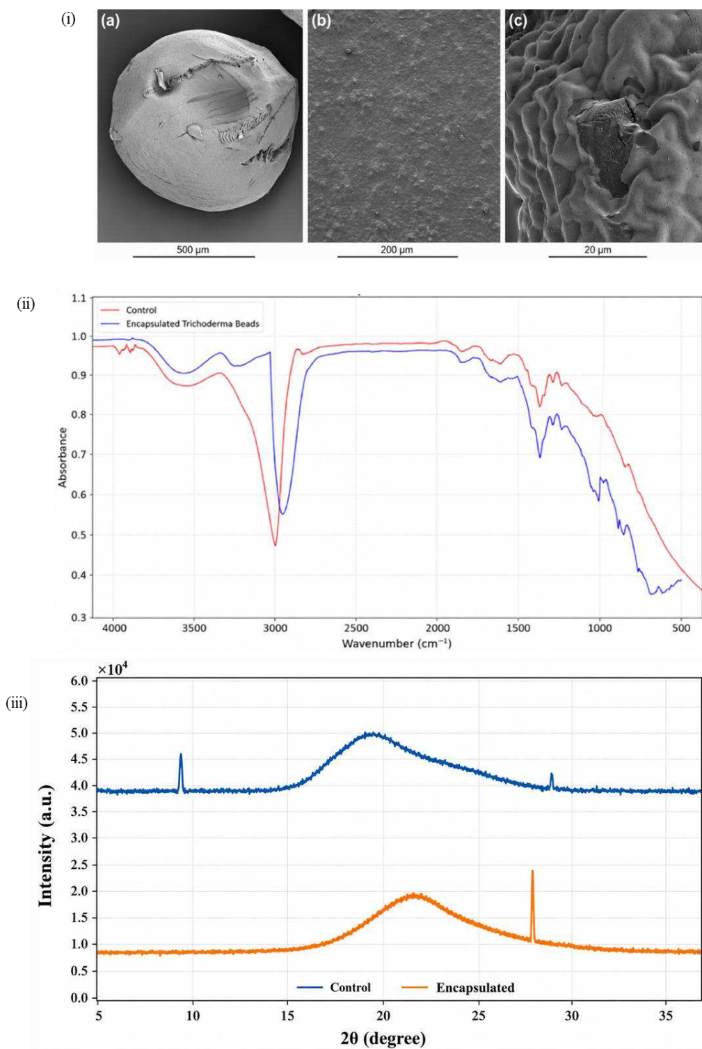
Figure 3. Morphological and structural characterization of encapsulated Trichoderma hydrogel beads: (i) SEM micrographs showing (a) overall bead morphology, (b) surface morphology, and (c) internal porous structure; (ii) FTIR spectra of control and encapsulated Trichoderma beads indicating characteristic peak shifts and intermolecular interactions after encapsulation; and (iii) XRD patterns demonstrating structural modification and reduced crystallinity of the encapsulated beads compared to the control sample.
