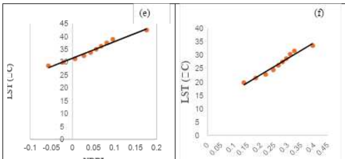
Fig. 11 Correlation between LST and NDBI for March, 2014(e) and February 2021(f)
