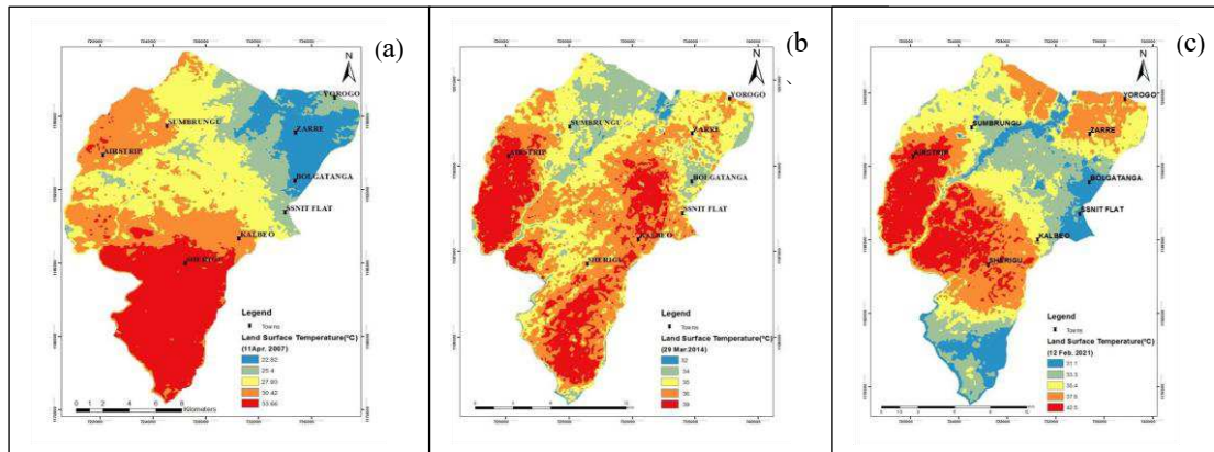
Fig. 6 Spatiotemporal trends in LST dynamics in Bolgatanga municipal for 2007(a), 2014(b), and 2021(c)
