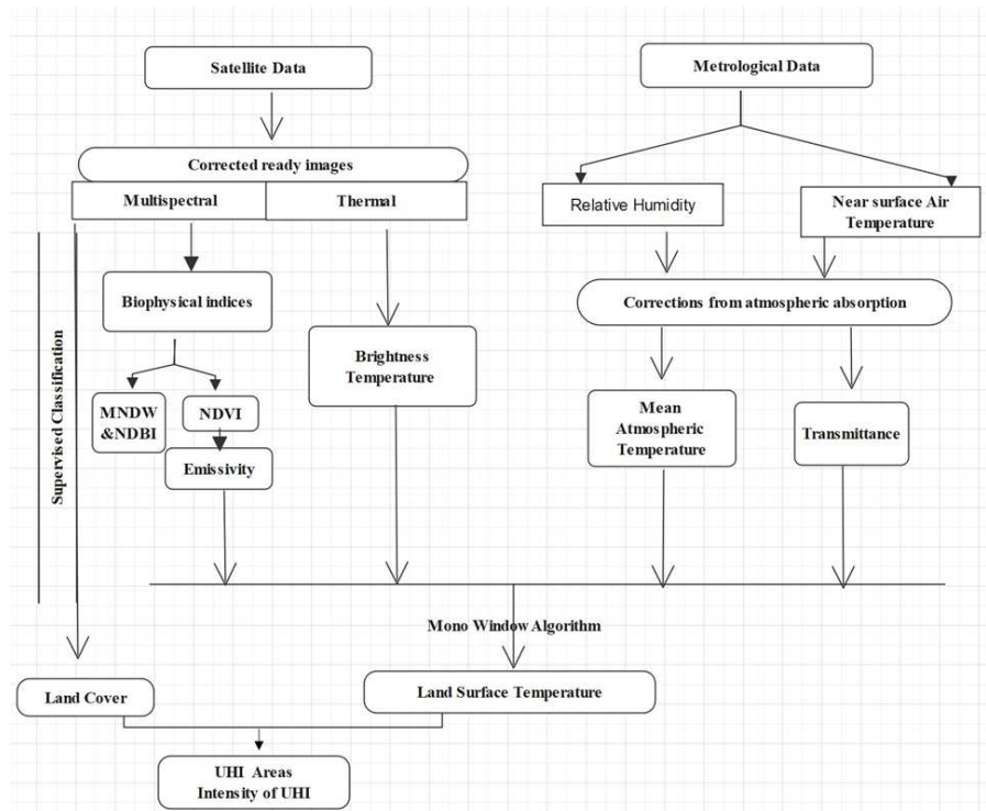
Fig. 3 Flowchart of the approach adopted in deriving the Urban Heat Island Intensity (UHII) from Landsat 5 imagery
