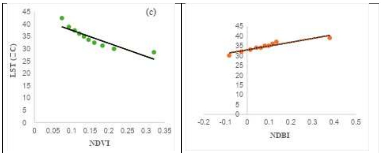
Fig.10 Correlation between LST and NDVI(c) for February, 2021 and LST and NDBI(d) for February 2007
