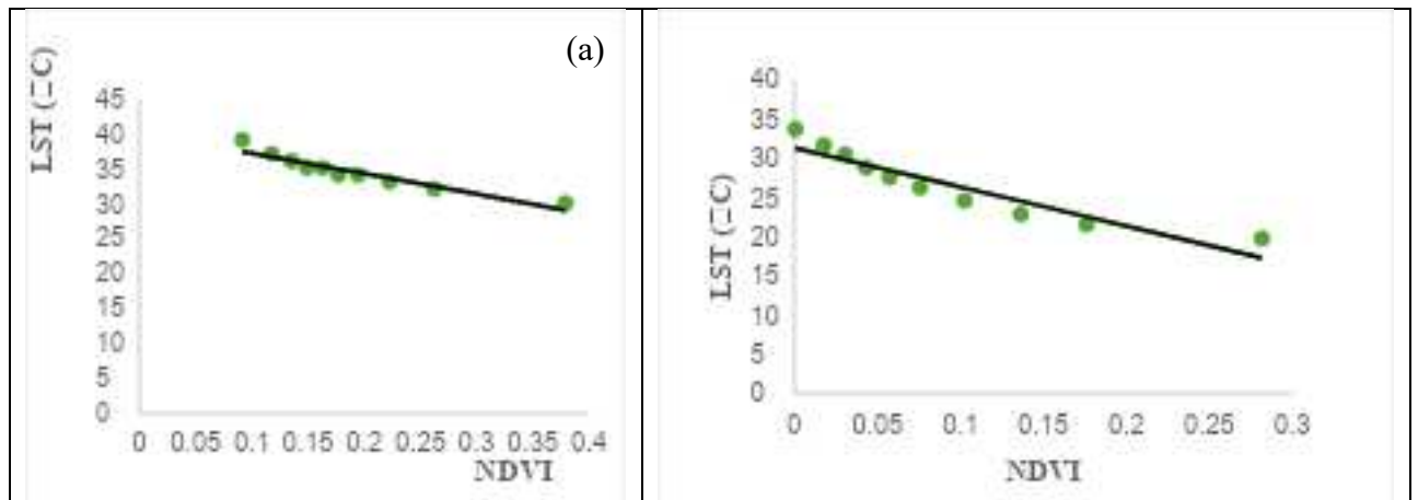
Fig. 9 Correlation between LST and NDVI for March,2007 (a) and April,2014(b)
