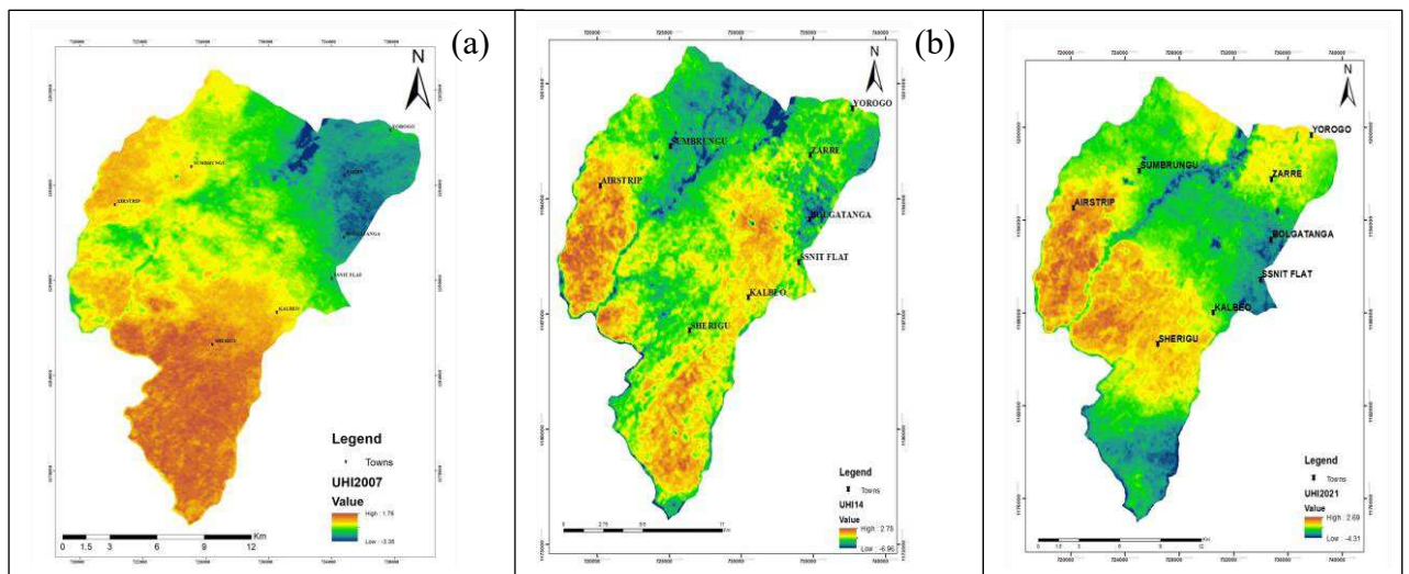
Fig. 7 Urban Heat Island Intensity (UHII) in Bolgatanga municipalities for 2007(a), 2014(b) and 2021(c)
