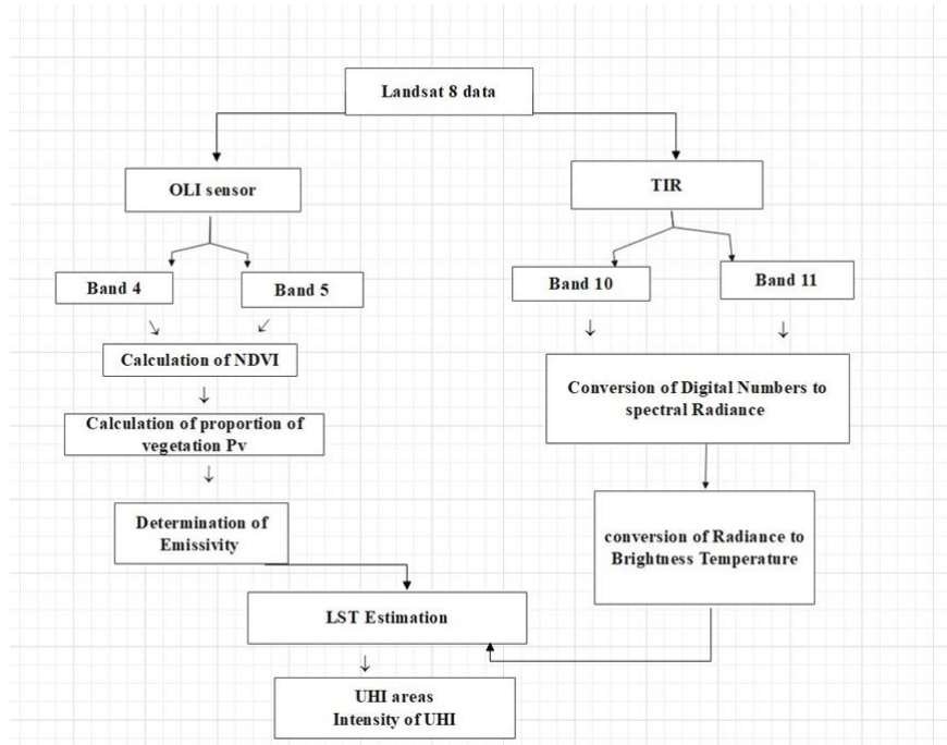
Fig. 2 Flow diagram of the approach used in deriving the Urban Heat Island Intensity (UHII) from Landsat 8 imagery
