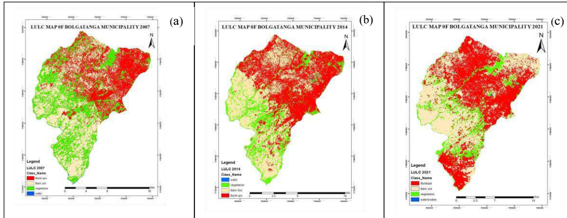
Fig. 4 Land use and Land cover (LULC) classes in Bolgatanga municipalities for 2007(a), 2014(b), and 2021(c)
