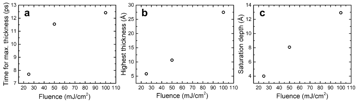
Extended Data Fig. 6. | Dependence of ultrafast disorder dynamics on laser fluence. a, Time required to reach the maximum disordered-layer thickness as a function of fluence. b, Maximum disordered-layer thickness as a function of fluence. c, Saturation depth of the disordered layer as a function of fluence. All three parameters exhibit a systematic increase with increasing fluence.
