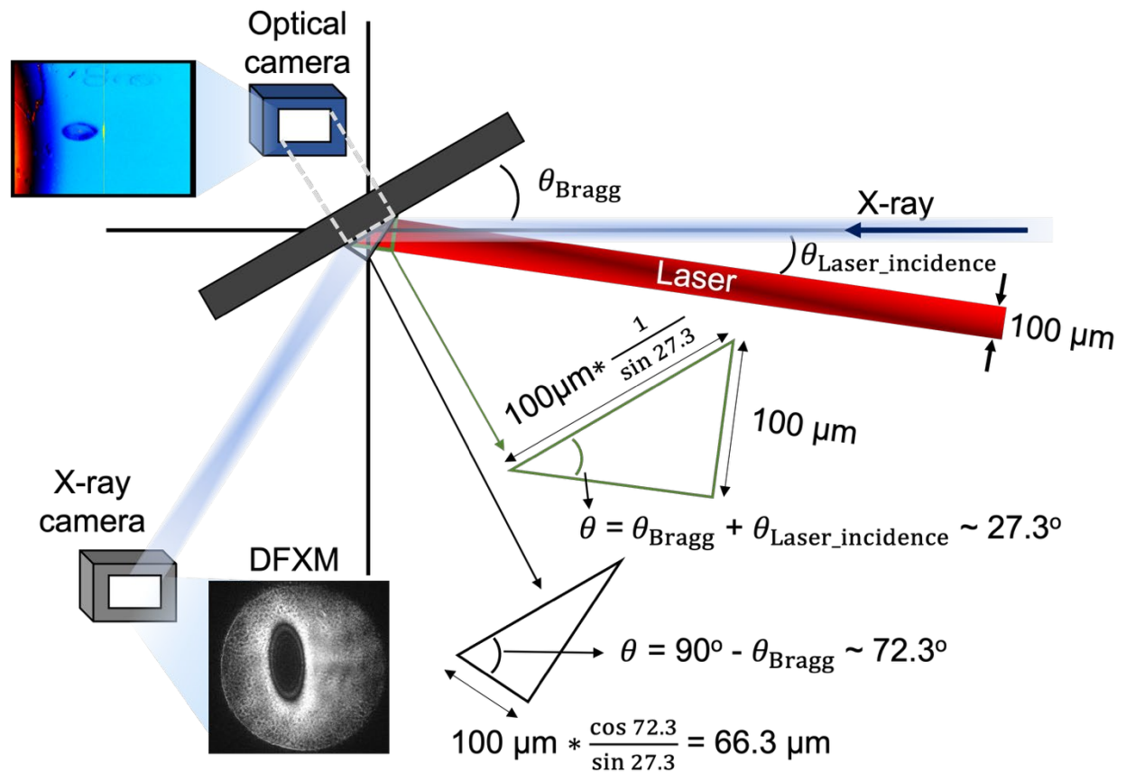
Extended Data Fig. 4. | Relationship between the sample surface projection and the observed projection on the X-ray detector. The projection on the sample surface is influenced by the Bragg angle and laser incident angle, while the observed projection on the detector is determined by the geometric constraints of Bragg reflection.
