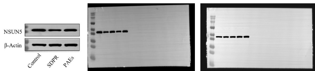
Fig. S2 Chemiluminescent image and overlay of the full membrane containing NSUN5 and \beta -actin.
