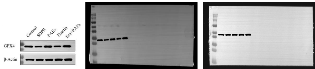
Fig. S1 Chemiluminescent image and overlay of the full membrane containing GPX4 and \beta -actin.
