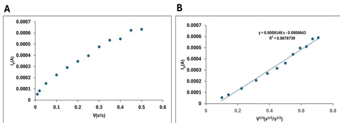
Fig. 7 A presents the relationship between peak current ( I_p ) and scan rate ( \nu ), showing a nonlinear trend. In contrast, B demonstrates a good linear relationship between peak current and the square root of scan rate ( \nu^{1/2} ) with a high correlation coefficient ( R^2 \approx 0.99 ), suggesting that the electrochemical process is predominantly diffusion-controlled
