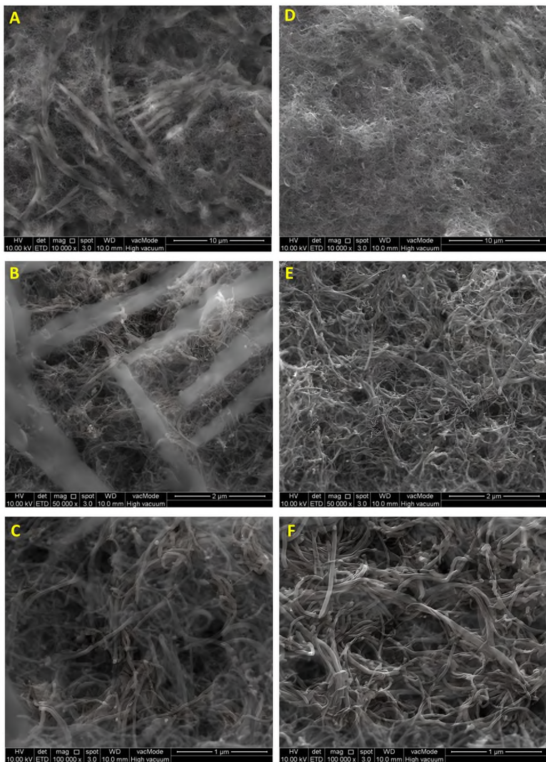
Fig. 3 (A–C) SPCE modified with 0.25 % (w/v) MWCNTs recorded at magnifications of 10k, 50k, and 100k, respectively; (D–F) SPCE modified with 1 % (w/v) MWCNTs recorded at magnifications of 10k, 50k, and 100k, respectively.
