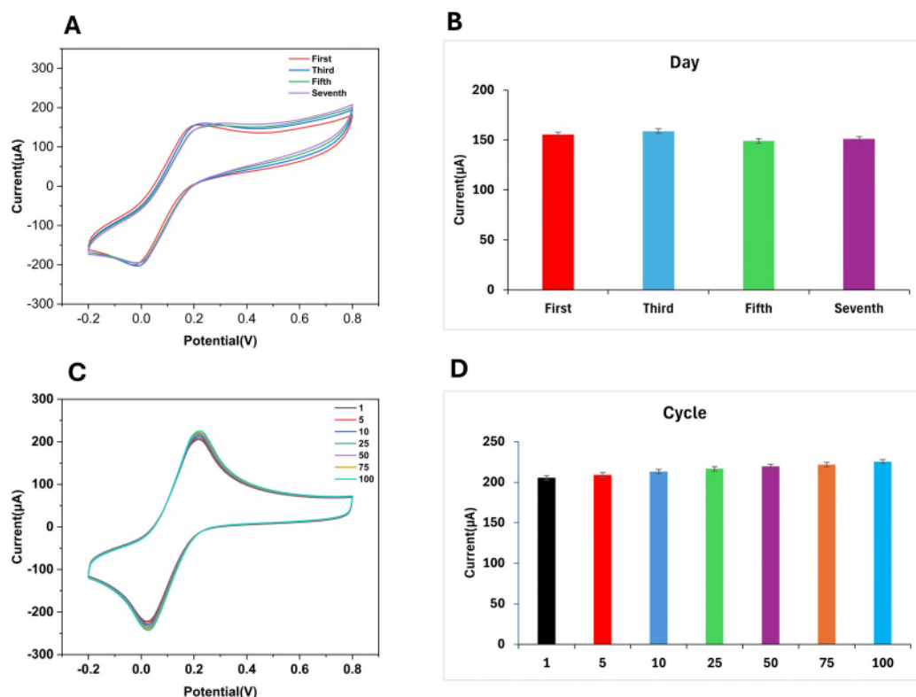
Fig. 10 (A) Corresponding peak current responses over different days, indicating the storage stability of the immunosensor under dry conditions at 4 °C. (B) Related histograms. (C) CV curves obtained over 100 consecutive cycles, used to evaluate the cycling stability. (D) Related histograms.
