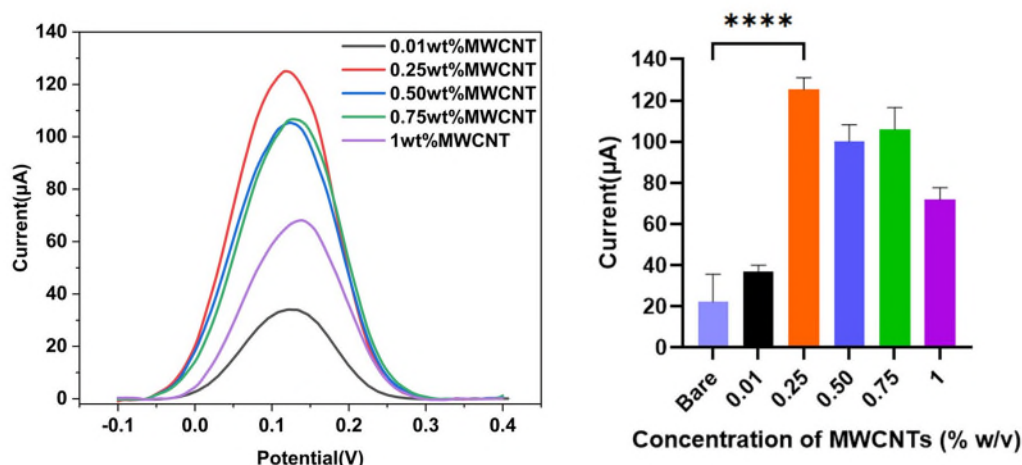
Fig. 5 Effect of MWCNTs concentration on the electrochemical response of SPCE. (A) Differential pulse voltammetry (DPV) curves of SPCE modified by MWCNTs. The peak current varies systematically with MWCNT concentration (0.01, 0.25, 0.50, 0.75, and 1% w/v). (B) Corresponding statistical analysis of DPV peak currents, showing that the 0.25 % (w/v) MWCNT-modified SPCE exhibits the highest current response. Data are presented as mean \pm SD (n = 3). Asterisks denote statistical significance (****, p < 0.0001).
