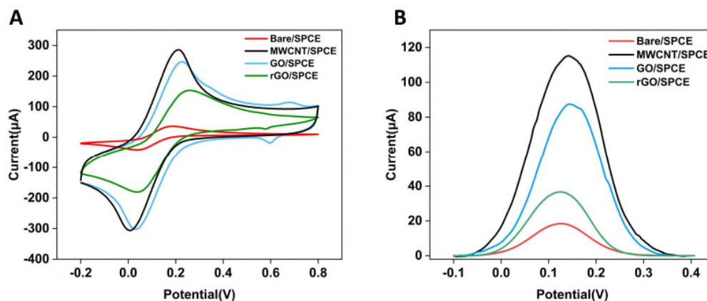
Fig. 2 Electrochemical characterization of SPCE modified with different nanomaterials. (A) Cyclic voltammetry (CV) responses of bare SPCE, GO-SPCE, rGO-SPCE, and 1 %(w/v) MWCNT/SPCE
