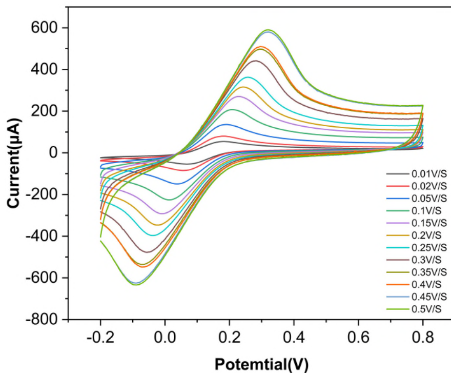
Fig. 6 shows the CVs of the MWCNT-modified electrode in 5 mM [\text{Fe}(\text{CN})_6]^{3-/4-} solution at different scan rates (0.01–0.5 V/s). As the scan rate increases, both anodic and cathodic peak currents increase significantly, while the peak potentials exhibit slight shifts, indicating a typical quasi-reversible electrochemical behavior.
