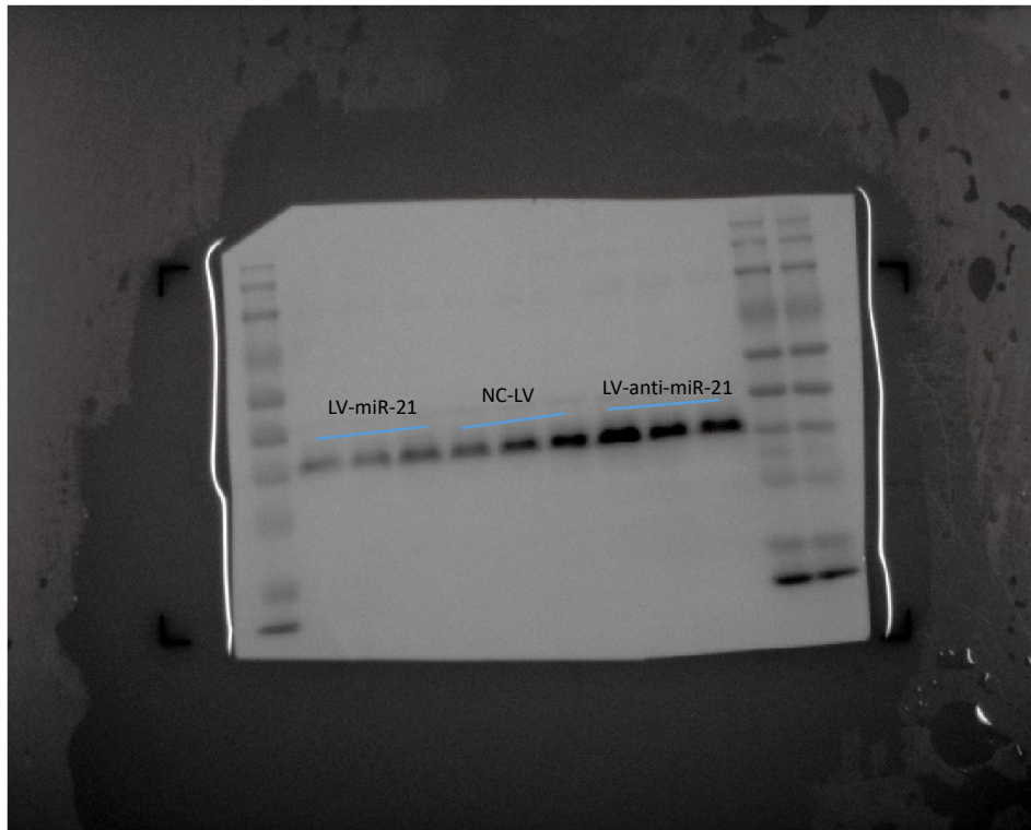
SOX2-ACTIN
