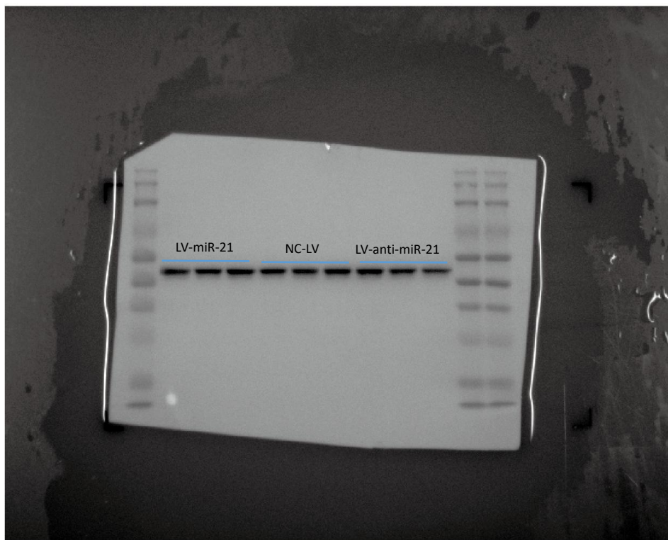
SOX2-ACTIN
