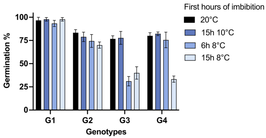
Fig. S2 Impact of temperature and time of cold exposure during early imbibition on final germination percentage.
