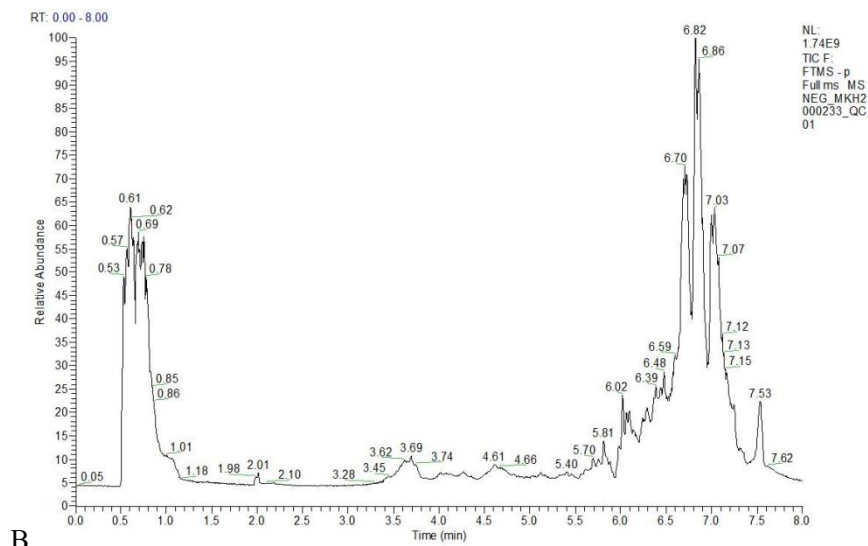
Fig.4 TIC diagram obtained by LC-MS/MS analysis in positive and negative ion modes
