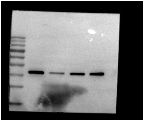
SLC7A11
