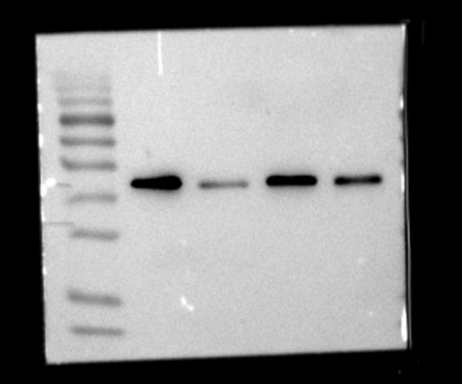
SLC7A11
