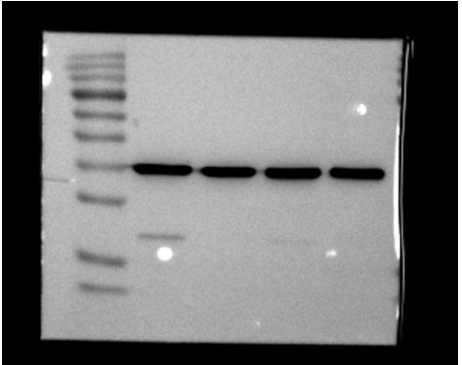
GAPDH
