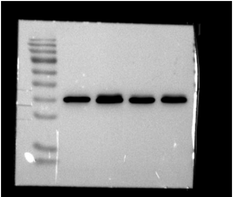
GAPDH
