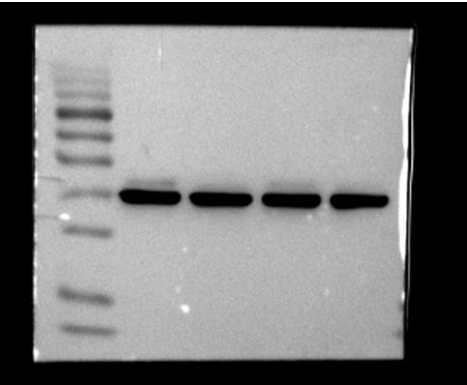
GAPDH
