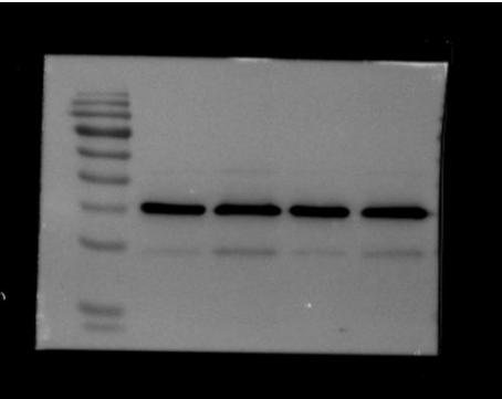
GAPDH
