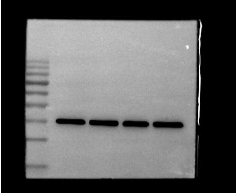
GAPDH
