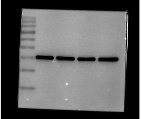
GAPDH
