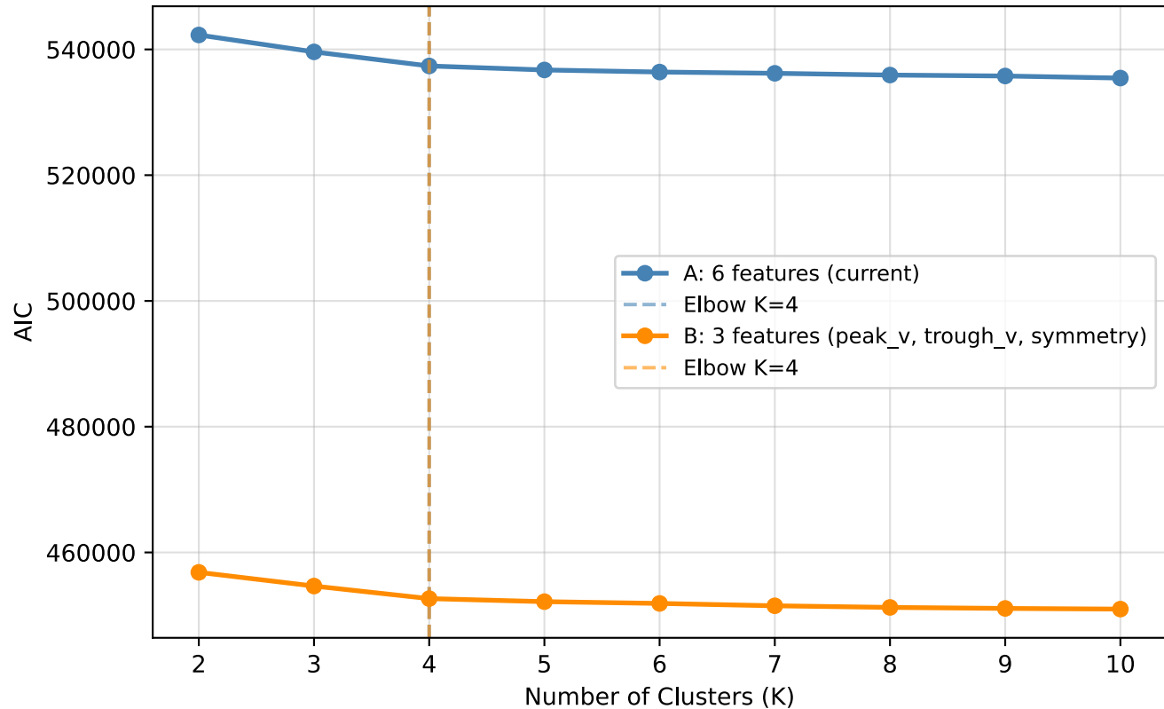
AIC Score by Feature Set
