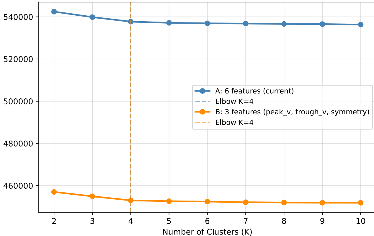
BIC Score by Feature Set
