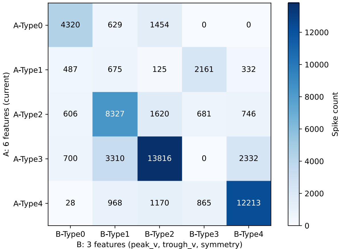
Cross-tabulation A vs B (ARI = 0.407)
