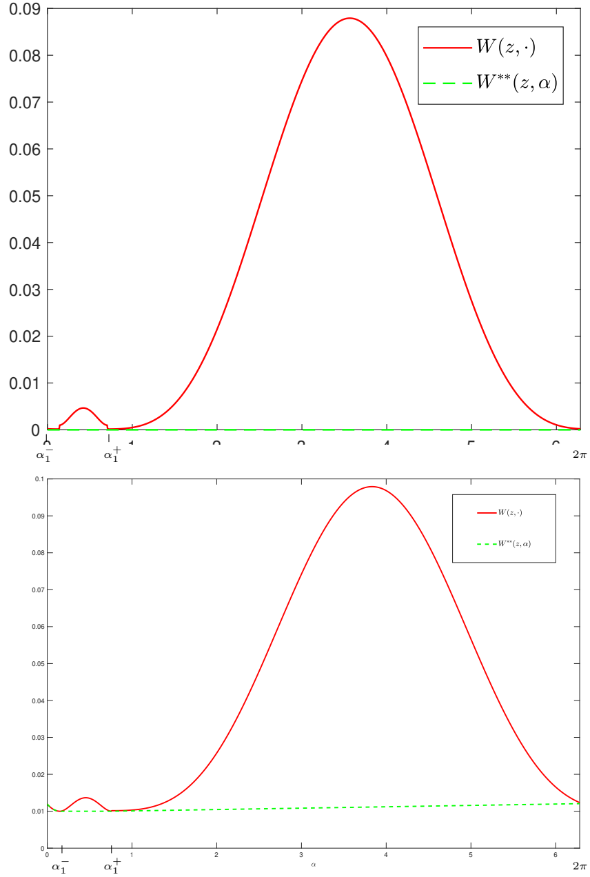
Figure 7: Sketch of the construction of the underestimator L(z, \alpha) of W(z, \alpha) in the proof of Lemma 2 leading to Q^{**}(z, \alpha) . Top: The special case (i) with \mu_c = 0 . Connecting the minima of W(z, \cdot) at \alpha = \alpha_1^- = 0 , at \alpha = \alpha_1^+(z) and at \alpha = 2\pi with minimal energy 0 yields L(z, \alpha) \equiv 0 . Bottom: The case (iii), here with \mu_c < \mu , for fixed z \geq z_{\text{crit}} . For \alpha \in [0, \alpha_1^-(z)) , W(z, \cdot) is strictly convex. For \alpha \in [\alpha_1^-(z), \alpha_1^+(z)] , L(z, \alpha) \equiv e_{\mu, \mu_c}(z) - \frac{\mu}{2}z^2 is constant, connecting the two minima by a straight line. For \alpha \in [\alpha_1^+(z), 2\pi] , L(z, \alpha) is a slightly increasing affine function, connecting (\alpha_1^+(z), W(z, \alpha_1^+(z))) with (2\pi, W(z, 2\pi)) . In both plots, the double well is strongly exaggerated to better illustrate the principle.
