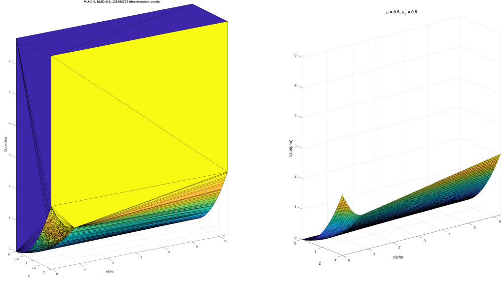
Figure 8: Left: Simplified triangulation of the convexification of \text{epi}(Q) for (z, \alpha) \in [0, 2] \times [0, 2\pi] and \mu = \mu_c = 0.5 as computed by our algorithm. The lateral and top surfaces are in blue, the color of the front depends on the value of z (e.g. yellow for z = 2 ). Right: Plot of l(z, \alpha) for (z, \alpha) \in [0, 2] \times [0, 2\pi] and \mu = \mu_c = 0.5 defined by the right hand side of Eqn. (44), cf. the proof of Lemma 2. In both plots one can identify the region on the bottom left where Q(z, \alpha) = Q^{**}(z, \alpha) = W(z, \alpha) + \frac{\mu}{2}z^2 .
