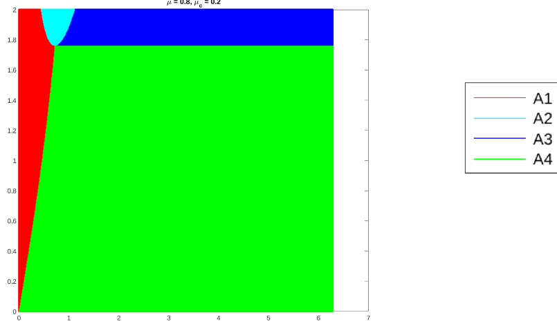
Figure 6: Plot of the sets A_i , 1 \leq i \leq 4 for \mu = 0.8 , \mu_c = 0.2 . \Gamma_{14} := \overline{A_1} \cap \overline{A_4} is not a straight line.
