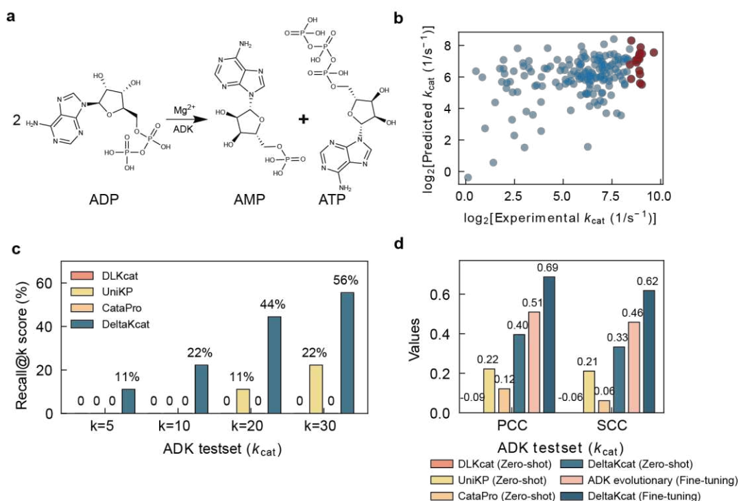
Fig. 5 Evaluation of DeltaKcat on an external adenylate kinase (ADK) dataset. (a) Adenylate kinase catalyzes the reaction. (b) Scatter plot of predicted versus observed absolute k_{\text{cat}} values for the external ADK dataset. Red points denote enzymes with observed k_{\text{cat}} values in the top 5% of the dataset. (c) Recall of highly active enzymes among top-ranked candidates. Highly active enzymes were defined as the top 5% by true k_{\text{cat}} . (d) Comparison of prediction performance between zero-shot and fine-tuned models on the ADK dataset, evaluated by Pearson and Spearman correlation coefficients.
