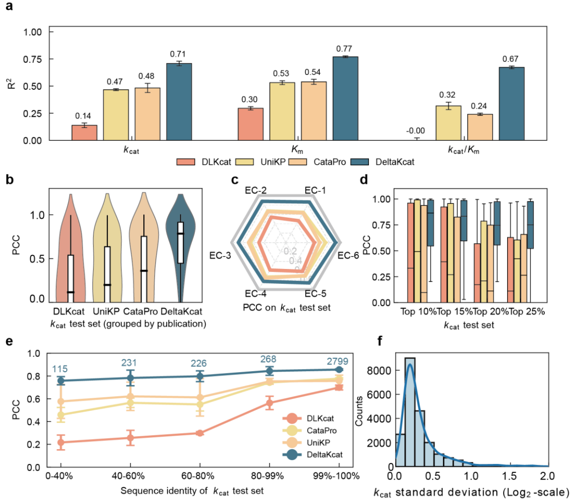
Fig. 3 Absolute kinetic parameter prediction on the sequence-diversity dataset. (a) Comparison of R^2 values for absolute parameter prediction. Performance of DeltaKcat versus DLKcat, UniKP, and CataPro baseline models on inferring absolute k_{cat} , K_m , and k_{cat}/K_m . (b) Publication-level Pearson correlation coefficients for absolute prediction across studies with more than five data points. (c) PCC results of different model based on EC classifications 1-6. (d) Evaluation of k_{cat} prediction (PCC) on subsets of the test set representing the top 10%, 15%, 20%, and 25% of absolute k_{cat} values within each EC class. (e) PCC evaluation across varying thresholds of maximum sequence similarity to the training set. (f) Histogram showing the distribution of the standard deviation of multiple absolute k_{cat} estimates for the same test complex, derived from different training-set reference anchors. The solid blue line is a kernel density estimate. The data in a, e and f are presented as mean values, and the error bars represent the standard deviation (s.d.) across three independent experiments using different random seeds. In each box plot, the lower and upper boundaries of the box represent the first quartile (Q1) and the third quartile (Q3), respectively. The whiskers extend from the quartiles to the minimum and maximum values within 1.5 times the interquartile range. The black line inside the box represents the median.
