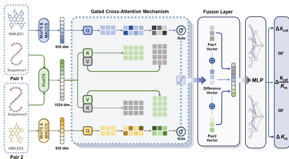
Fig. 1 DeltaKcat framework for predicting relative enzyme kinetic parameters. DeltaKcat takes a pair of enzyme-substrate complexes as input and predicts their relative k_{\text{cat}} , K_m , or k_{\text{cat}} / K_m values as the output, respectively. Protein sequences are encoded by ProtT5, and substrates are represented using MolT5 and MACCS features. Sequence and substrate embeddings are integrated through a gated cross-attention module, in which substrate-derived queries attend to protein-derived keys and values to capture enzyme-substrate interactions. A gating unit is applied after the softmax step to refine attention allocation. The resulting interaction vectors for the two complexes, together with their difference vector, are concatenated and passed to a multilayer perceptron for prediction.
