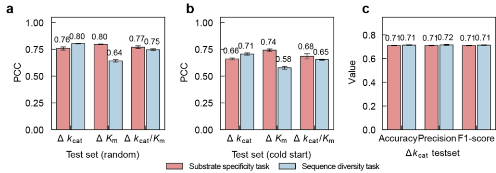
Fig. 2 Prediction of relative enzyme kinetic parameters by DeltaKcat. (a, b) Predictive performance of DeltaKcat on the sequence-diversity dataset and substrate-specificity dataset under random-split (a) and cold-start (b) settings for relative k_{cat} , relative K_m , and relative k_{cat}/K_m . In the cold-start split, each test pair contained at least one protein sequence not observed during training. (c) Classification performance of DeltaKcat for predicting the direction of kinetic changes in the sequence-diversity and substrate-specificity tasks. The data in a-c are presented as mean values, and the error bars represent the standard deviation (s.d.) across three independent experiments using different random seeds.
