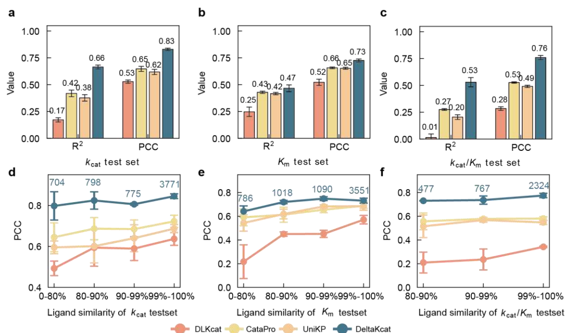
Fig. 4 Absolute kinetic parameter prediction on the substrate-specificity dataset. (a-c) Comparison of R^2 and PCC values for absolute parameter prediction. Performance of DeltaKcat versus DLKcat, UniKP, and CataPro baseline models on inferring absolute k_{cat} , K_m , and k_{cat}/K_m . (d-f) PCC evaluation across varying thresholds of maximum ligand similarity to the training set on k_{cat} , K_m , and k_{cat}/K_m . The data in a-f are presented as mean values, and the error bars represent the standard deviation (s.d.) across three independent experiments using different random seeds.
