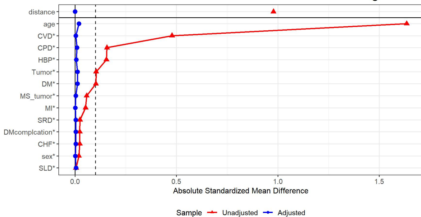
Standardized Mean Differences Before and After Matching
