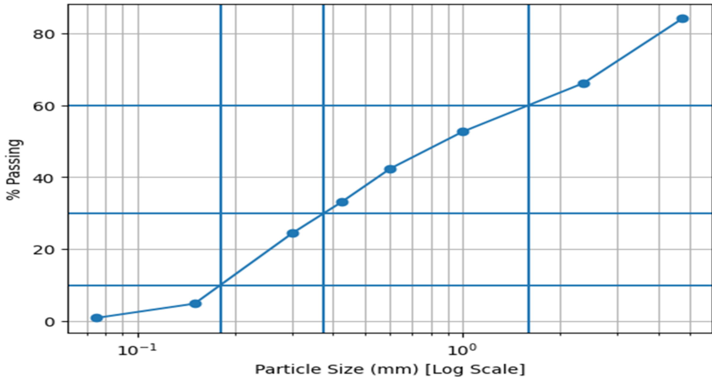
Grain Size Distribution Curve with D10, D30, D60
