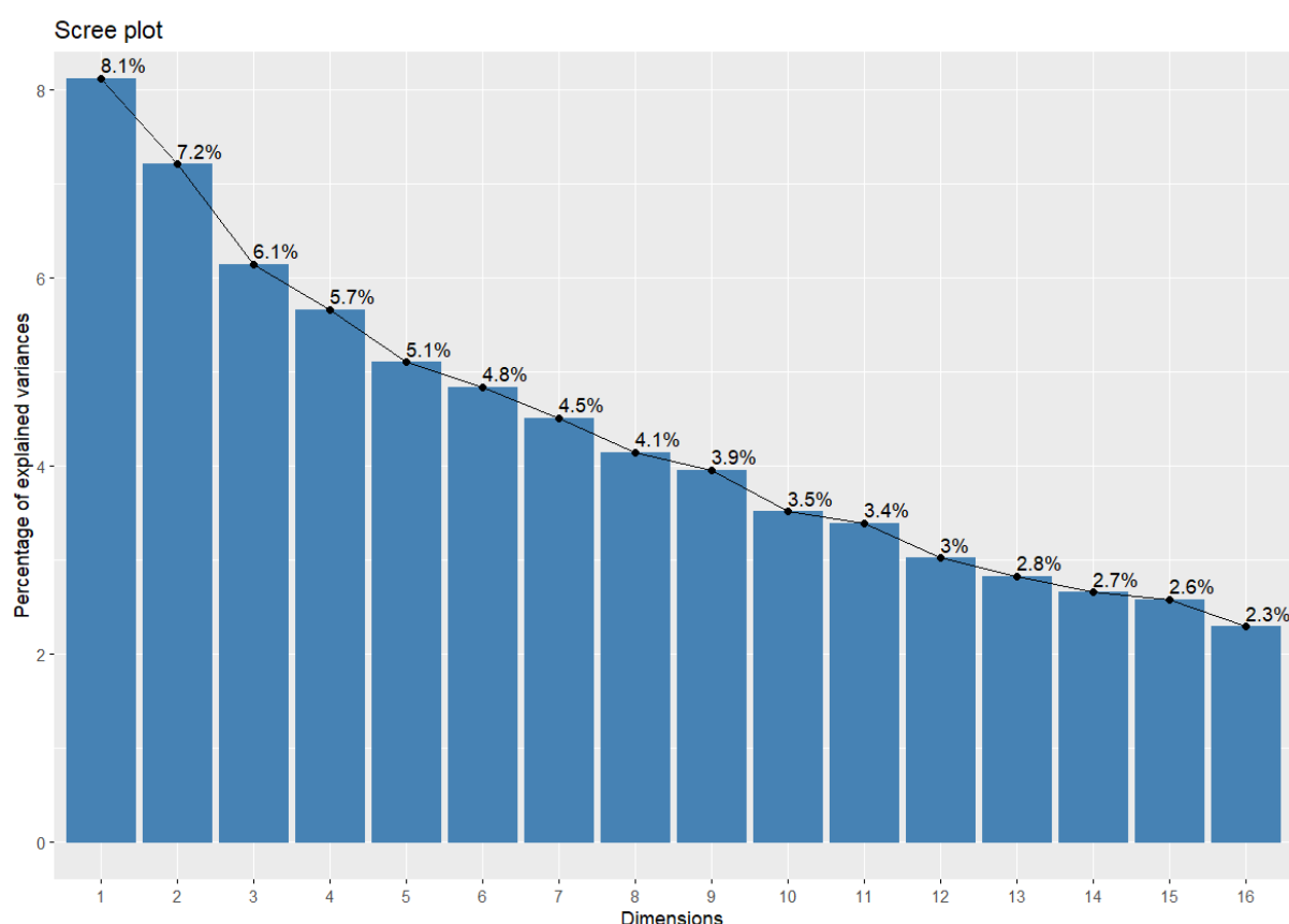
Figure S1. Scree plot illustrating the percentage of variation explained by the dimension
