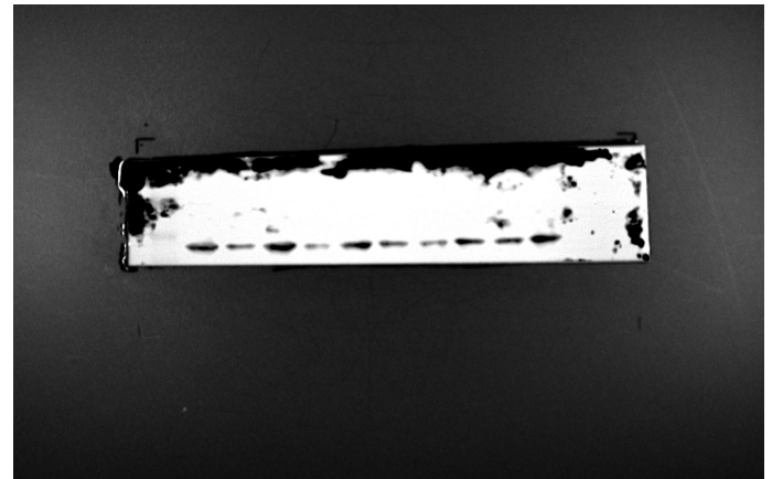
NFKB
