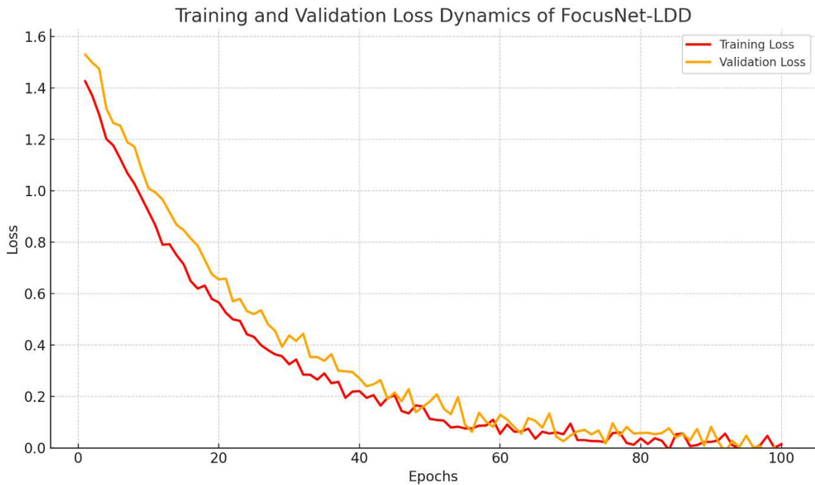
Figure 5: Training and Validation Loss Dynamics of the FocusNet-LDD Model Over 100 Epochs, Indicating Stable Optimization and Minimal Overfitting.
