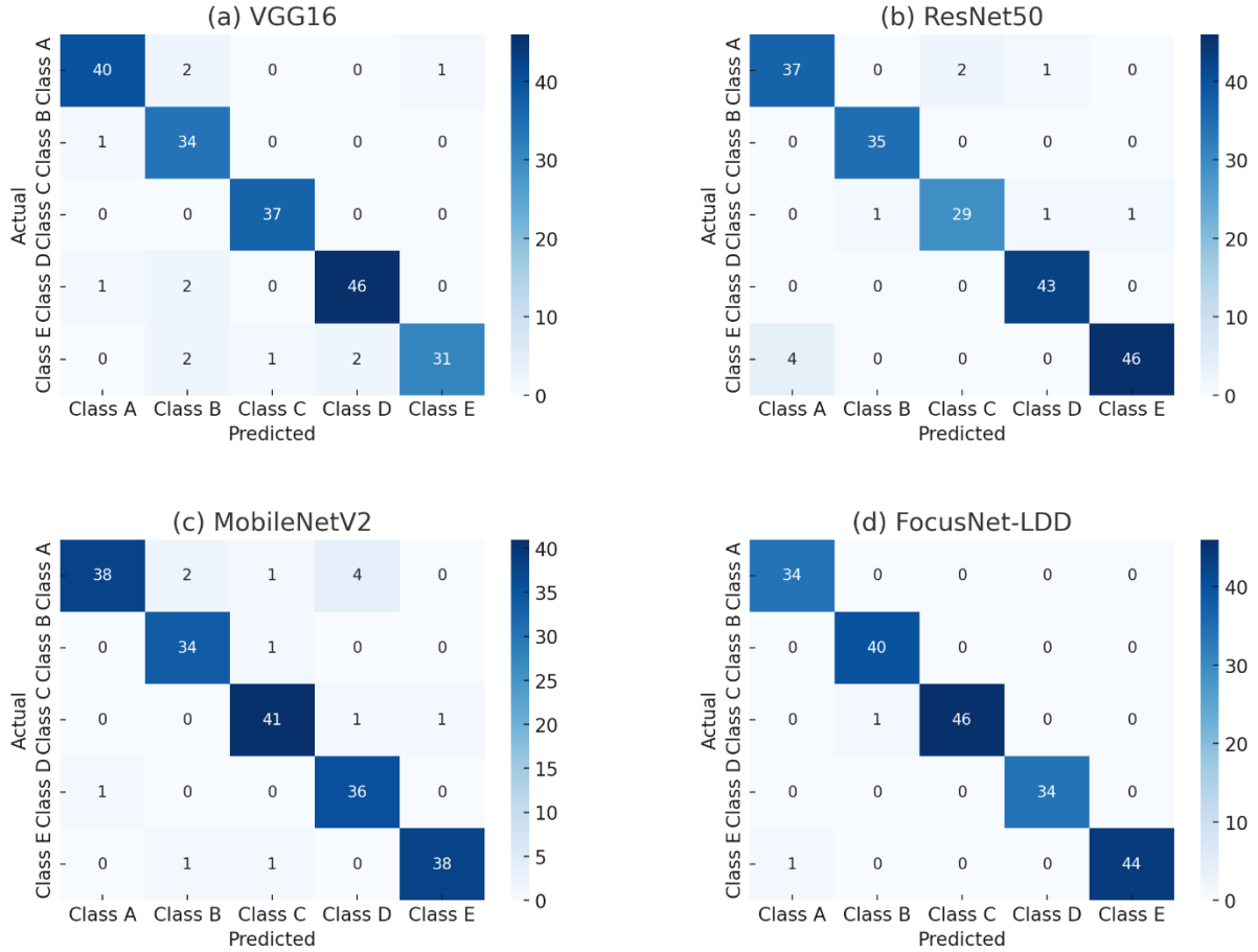
Figure 6: Confusion Matrices of VGG16, ResNet50, MobileNetV2, and FocusNet-LDD Showing Class-Wise Prediction Accuracy for Leaf Disease Classification
