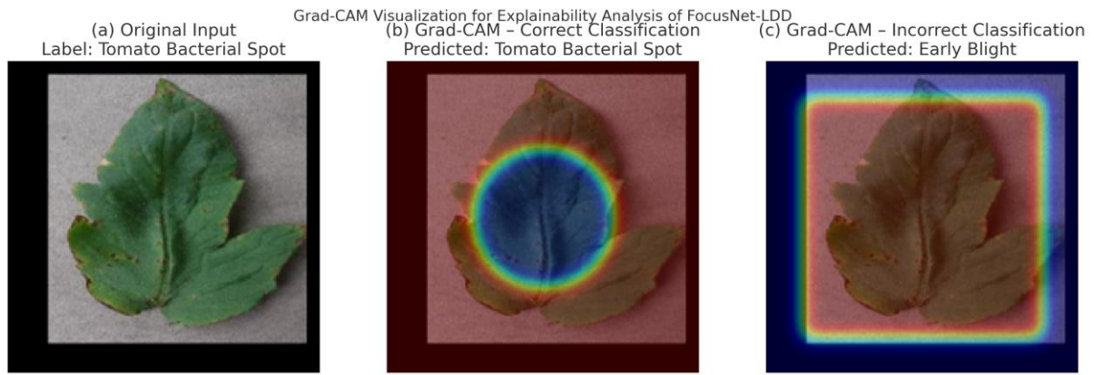
Figure 10: Grad-CAM Visualizations that show Attention Alignment in Correct vs. Incorrect Classifications by the FocusNet-LDD Model.
