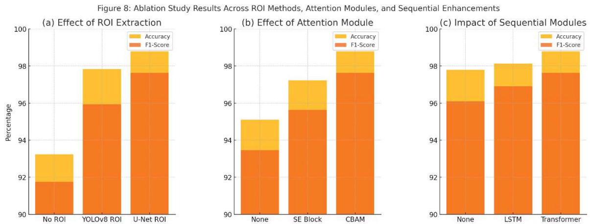
Figure 9: Ablation Testing of ROI Extraction, Attention Modules and Sequential Improvements. FocusNet-LDD Model of Leaf Disease Classification in focusnet
