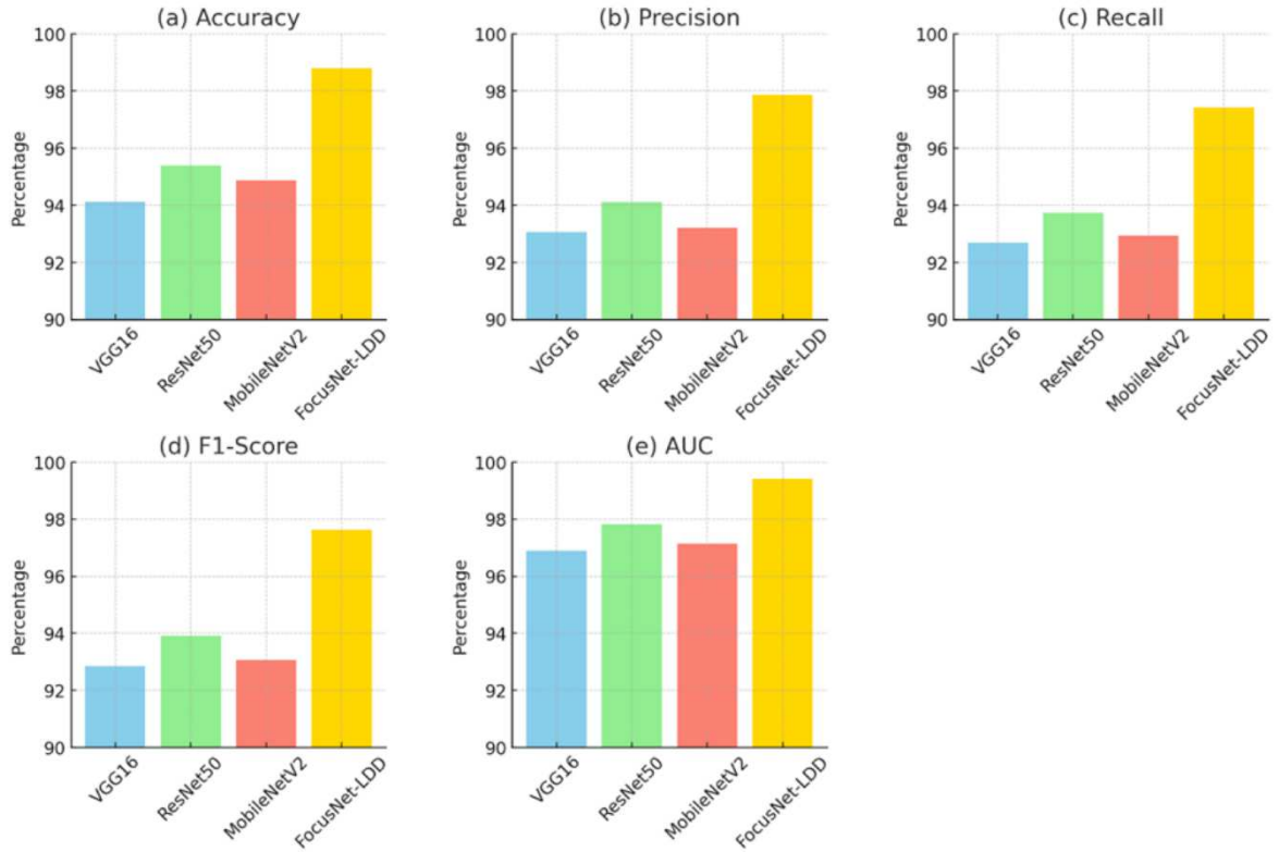
Comparative Performance of FocusNet-LDD and Baseline Models Across Evaluation Metrics
