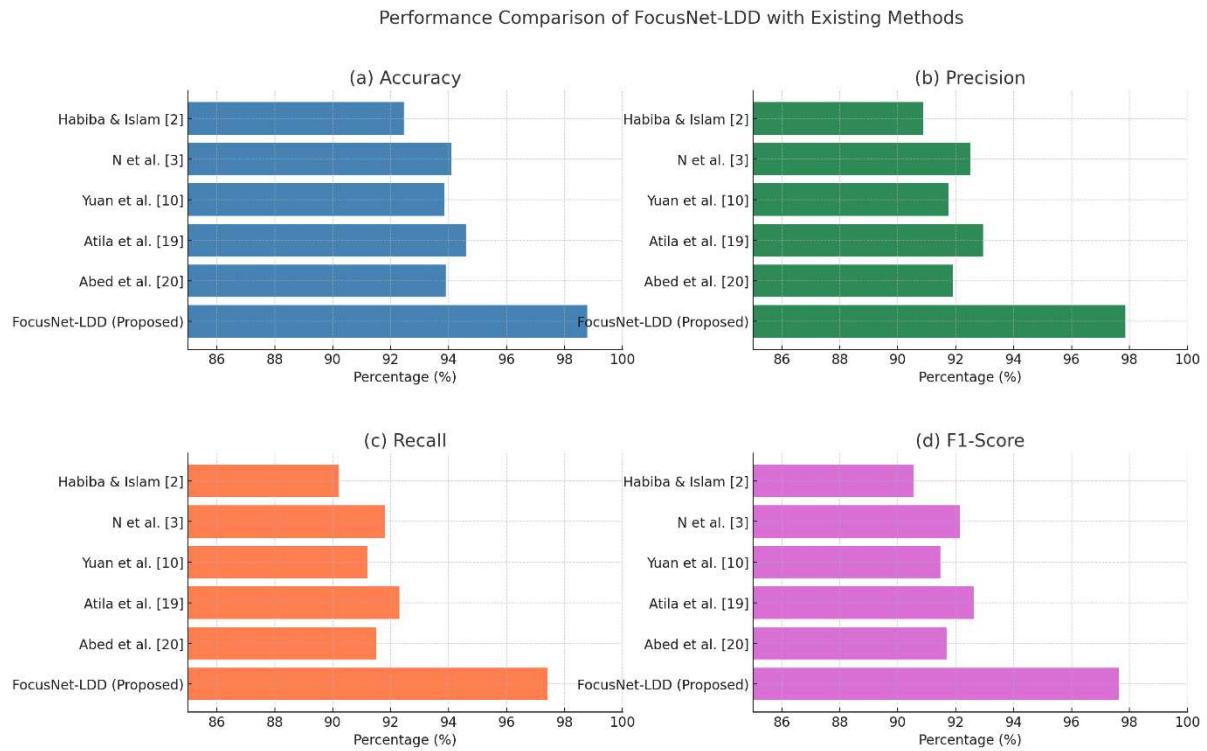
Figure 11: Performance Comparison of FocusNet-LDD with Existing Plant Disease Detection Approaches Both in Accuracy and Precision and in Recall and F1-Score Measures.
