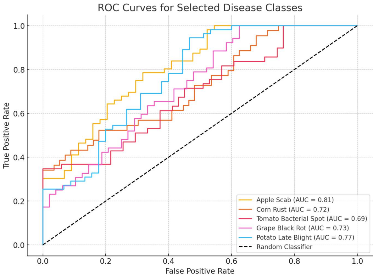
Figure 7: ROC Curves for Selected Plant Disease Classes Showing Model Discrimination Ability Across Different True Positive and False Positive Rates
