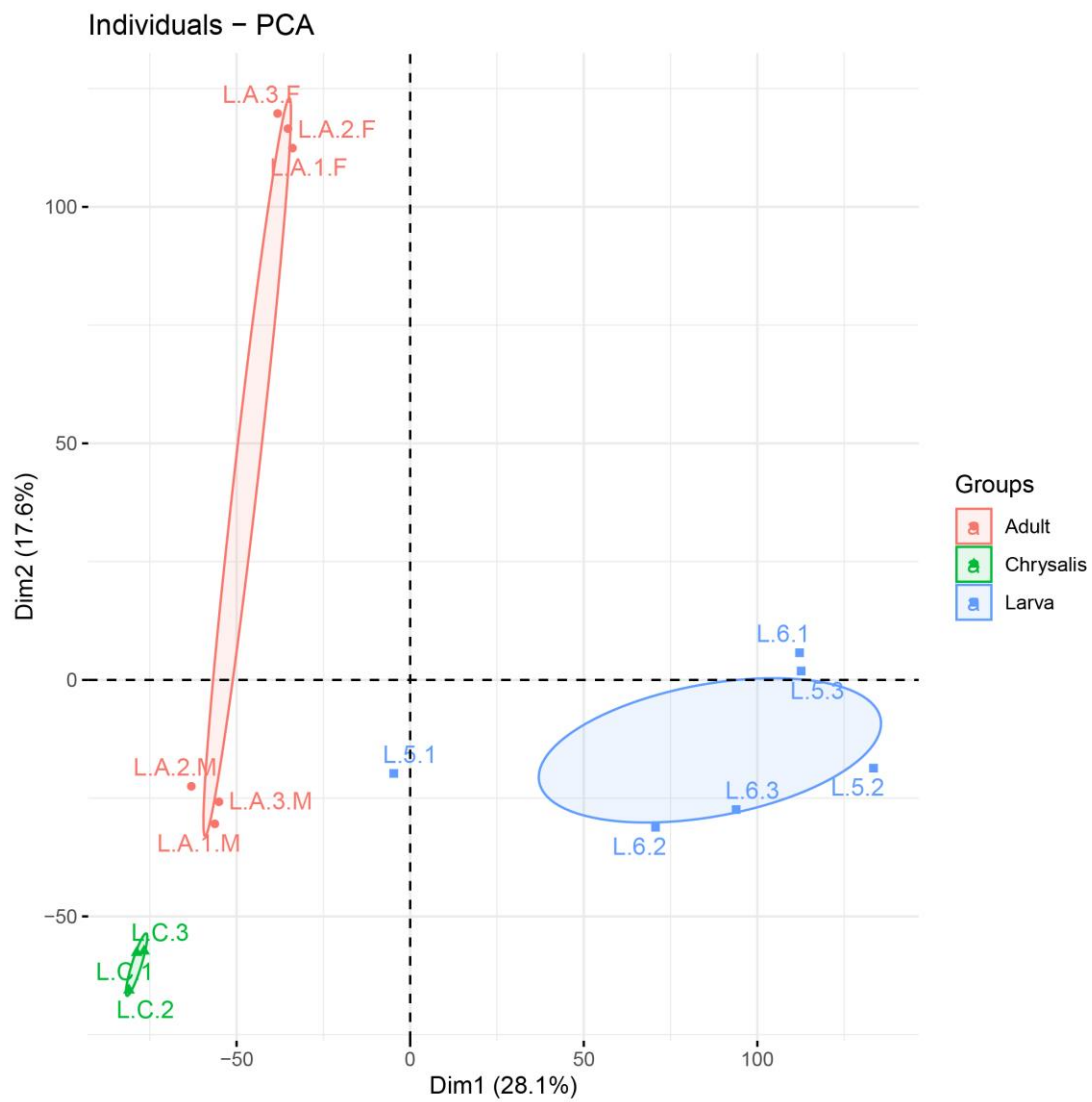
Figure S1 The principal components analysis of three developmental stages in S. litura . The expression of transcripts was transformed using rlog function.
