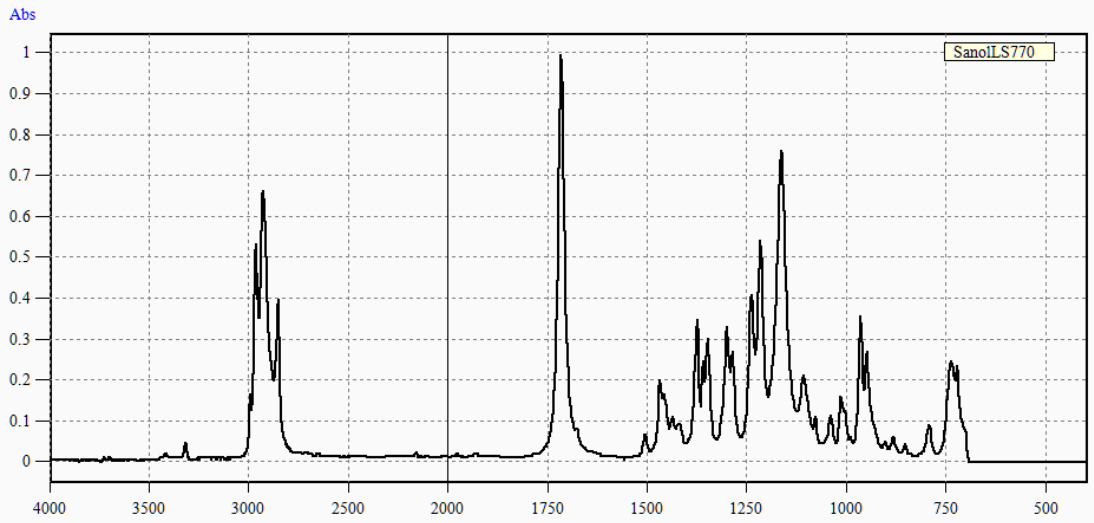
SanoL S770HINDERED AMINE LIGHT STABILIZERBIS(2,2,6,6-TETRAMETHYL-4-PIPERIDYL)SEBACATEC28H52N2O4CAS NO. 52829-0799ATR/dia
