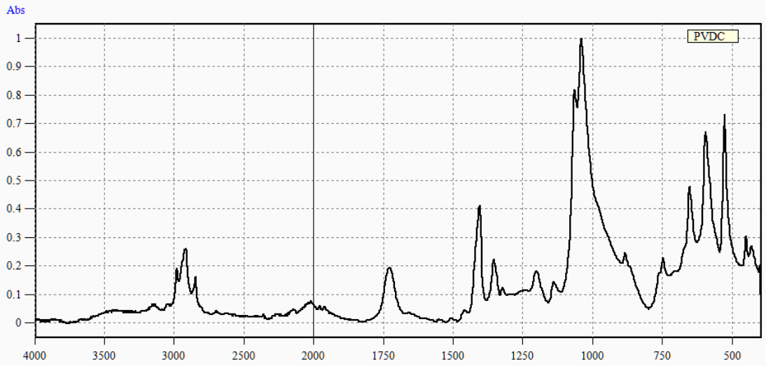
PVDC, Poly (vinylidene chloride) /wlap filmATR/diamond ATRcorrected
