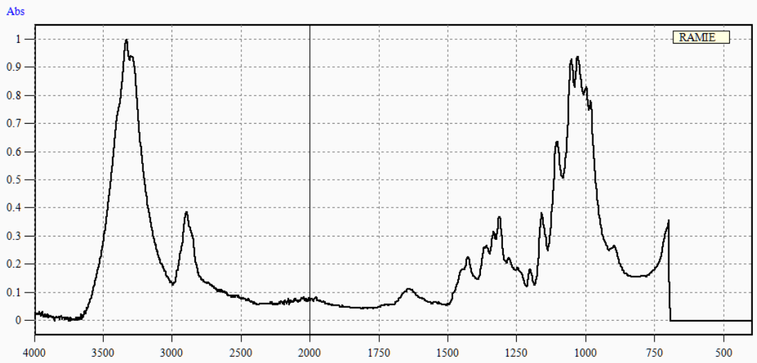
Ramie FiberATR/diamond ATRcorrected
