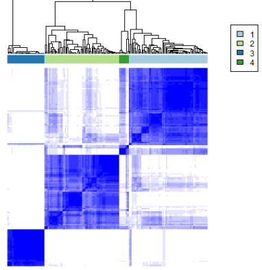
C consensus matrix k=4
