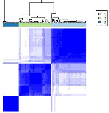
B consensus matrix k=3
