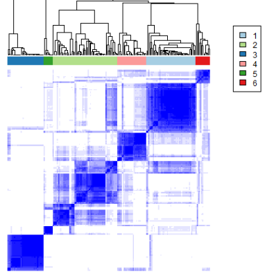
E consensus matrix k=6
