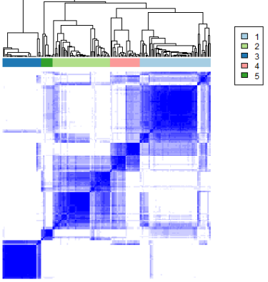
D consensus matrix k=5
