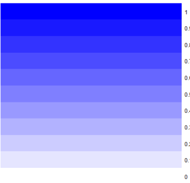
A consensus matrix legend
