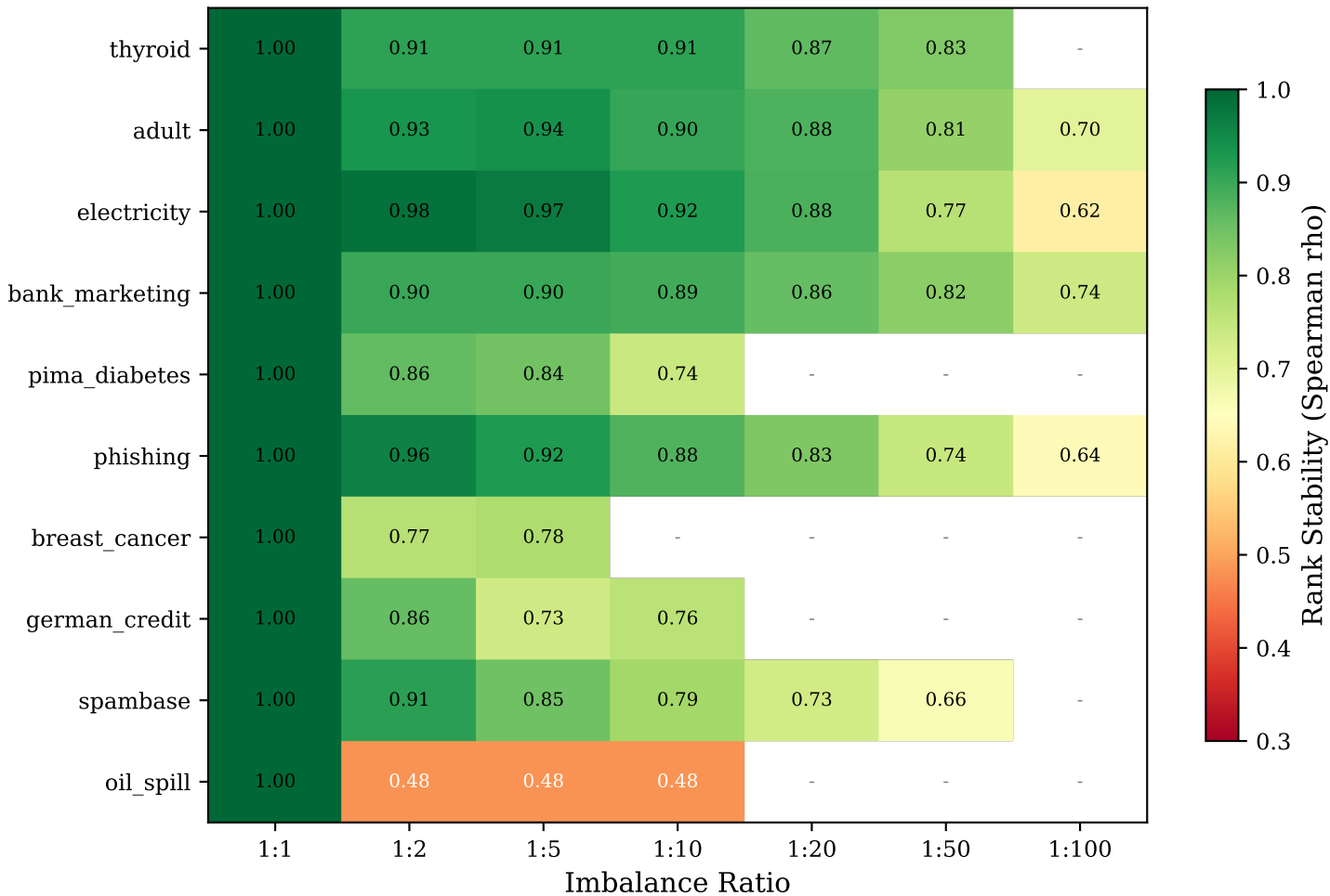
Rank Stability by Dataset and Imbalance Ratio
