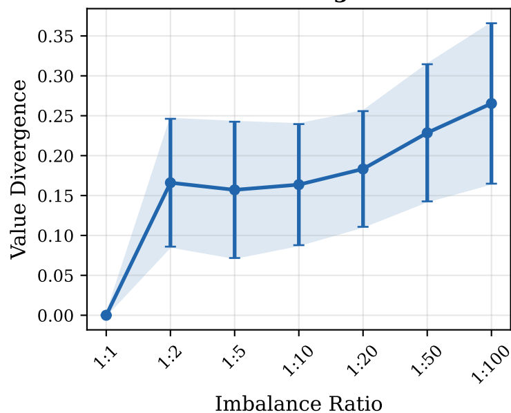
Value Divergence
