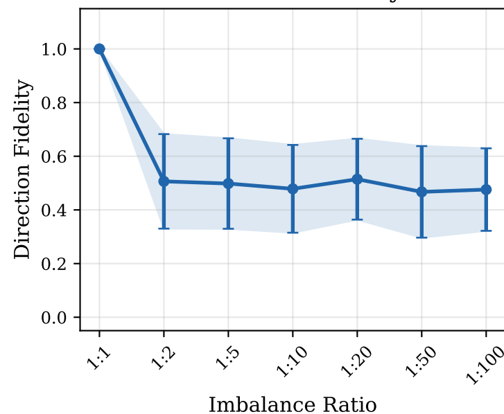
Direction Fidelity
