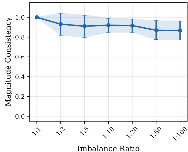
Magnitude Consistency
