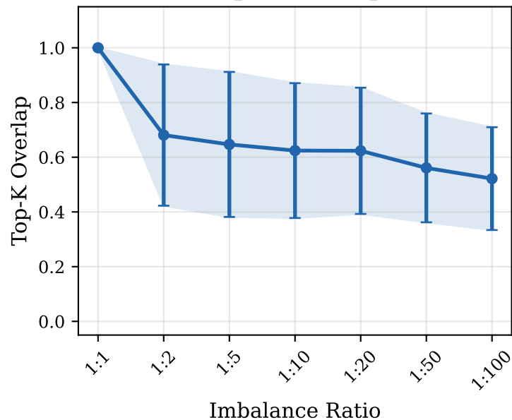
Value Divergence
