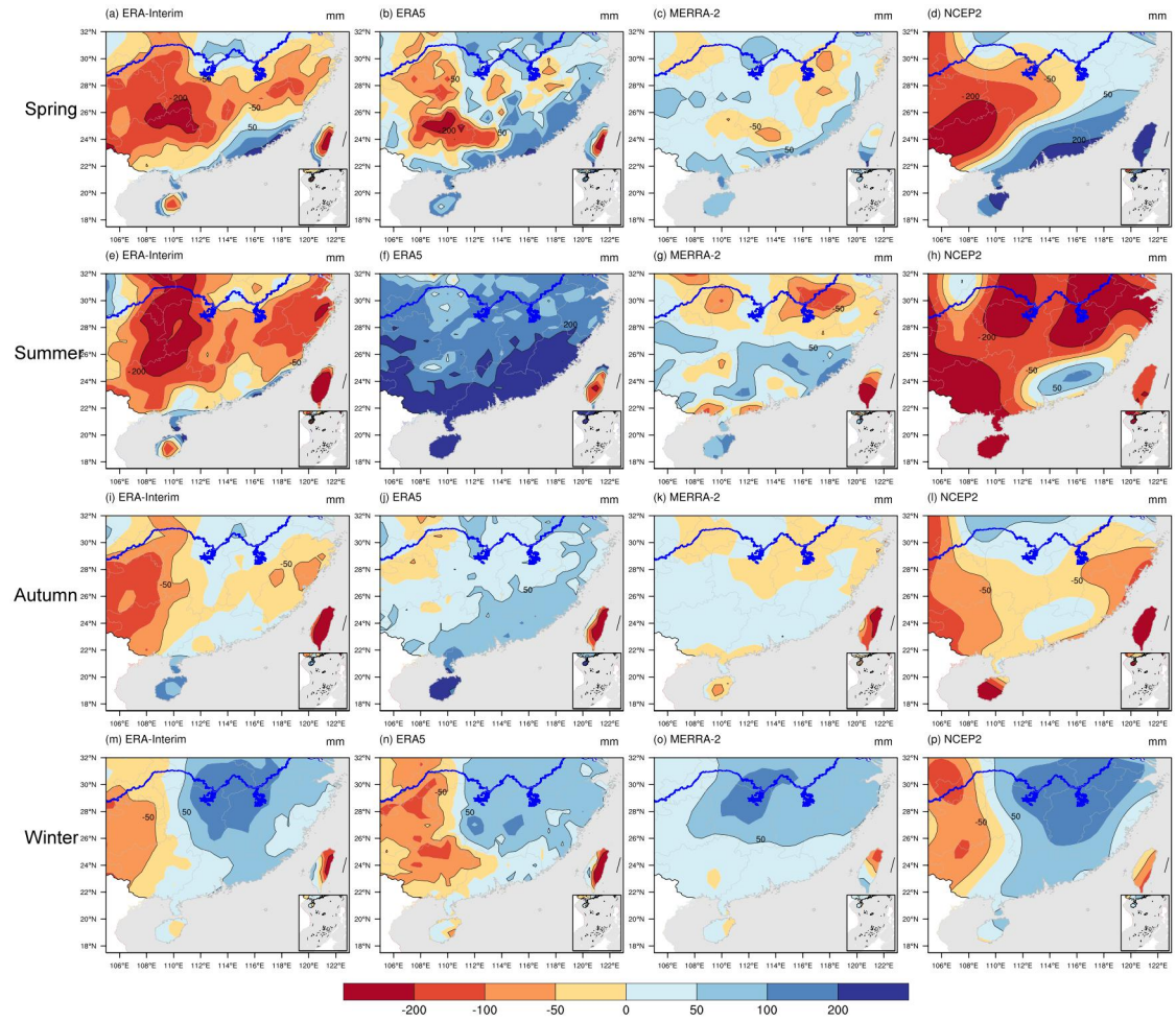
Fig. S2. Same as in Fig. S1 but for (a) to (d) spring, (e) to (h) summer, (i) to (l) autumn, and (m) to (p) winter.
