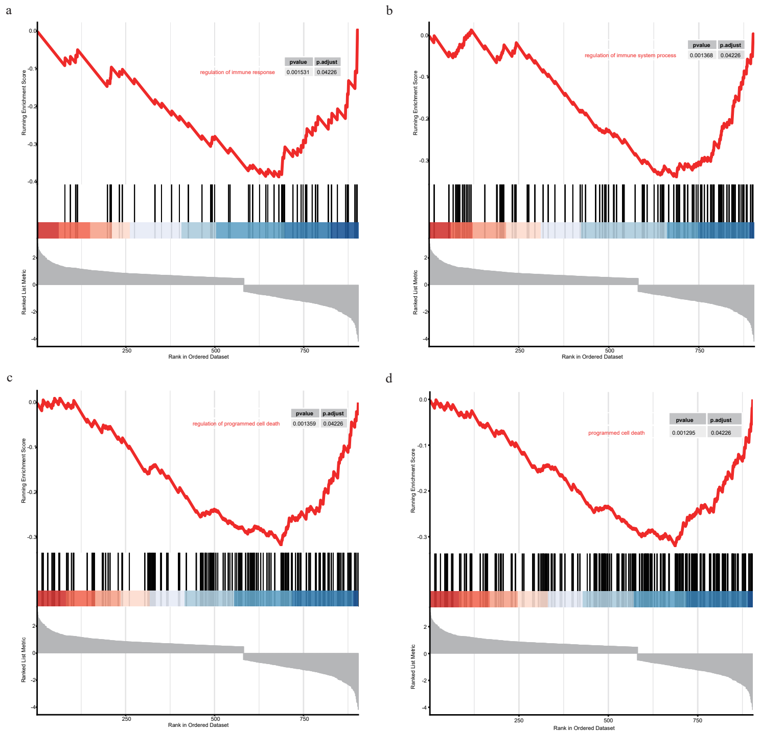
Fig S1 GSEA analysis of the BICC1+ CAFs. (a)regulation of immune response. (b)regulation of immune system process. (c) regulation of programmed cell death. (d) programmed cell death processes.
