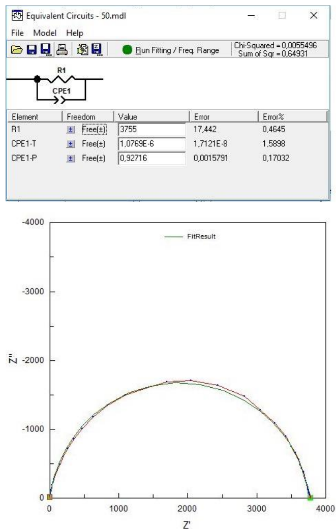
Fig. S2. Equivalent-circuit fitting of the Nyquist plot ( R_1 \parallel CPE_1 model).
