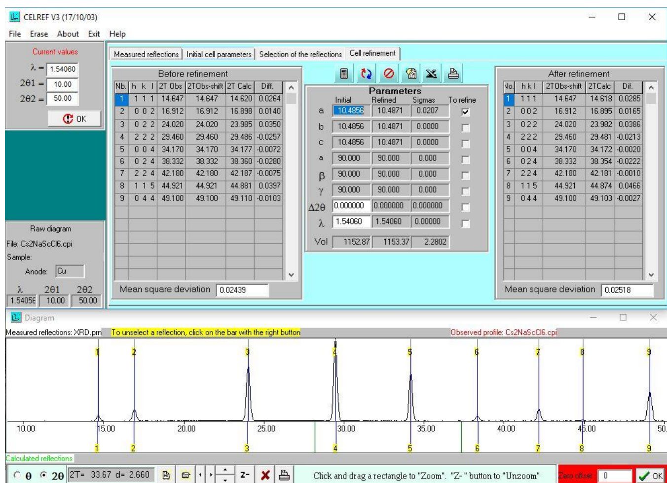
Fig. S1. Full-pattern XRD refinement of \text{Cs}_2\text{NaScCl}_6 using CELREF.
