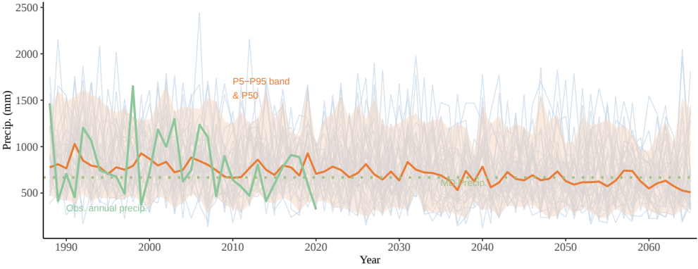
D Pintué 4 annual precip. under SSP585 (1988–2065)
