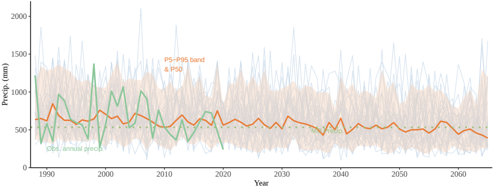
C Pintué 3 annual precip. under SSP585 (1988–2065)
