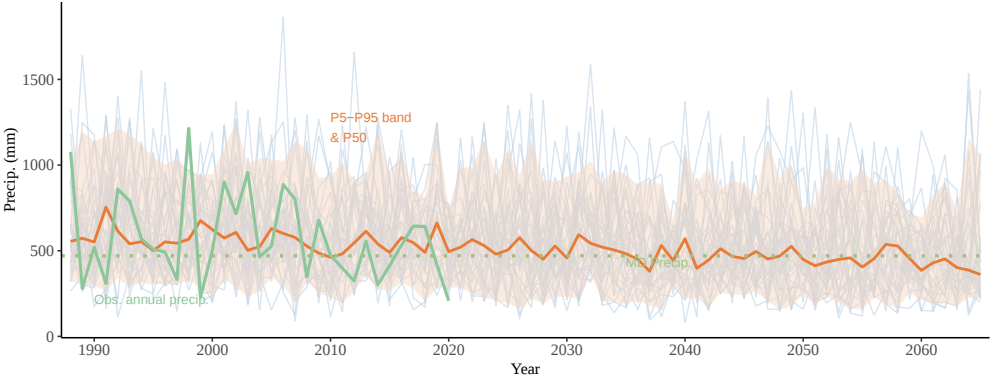
B Pintué 2 annual precip. under SSP585 (1988–2065)
