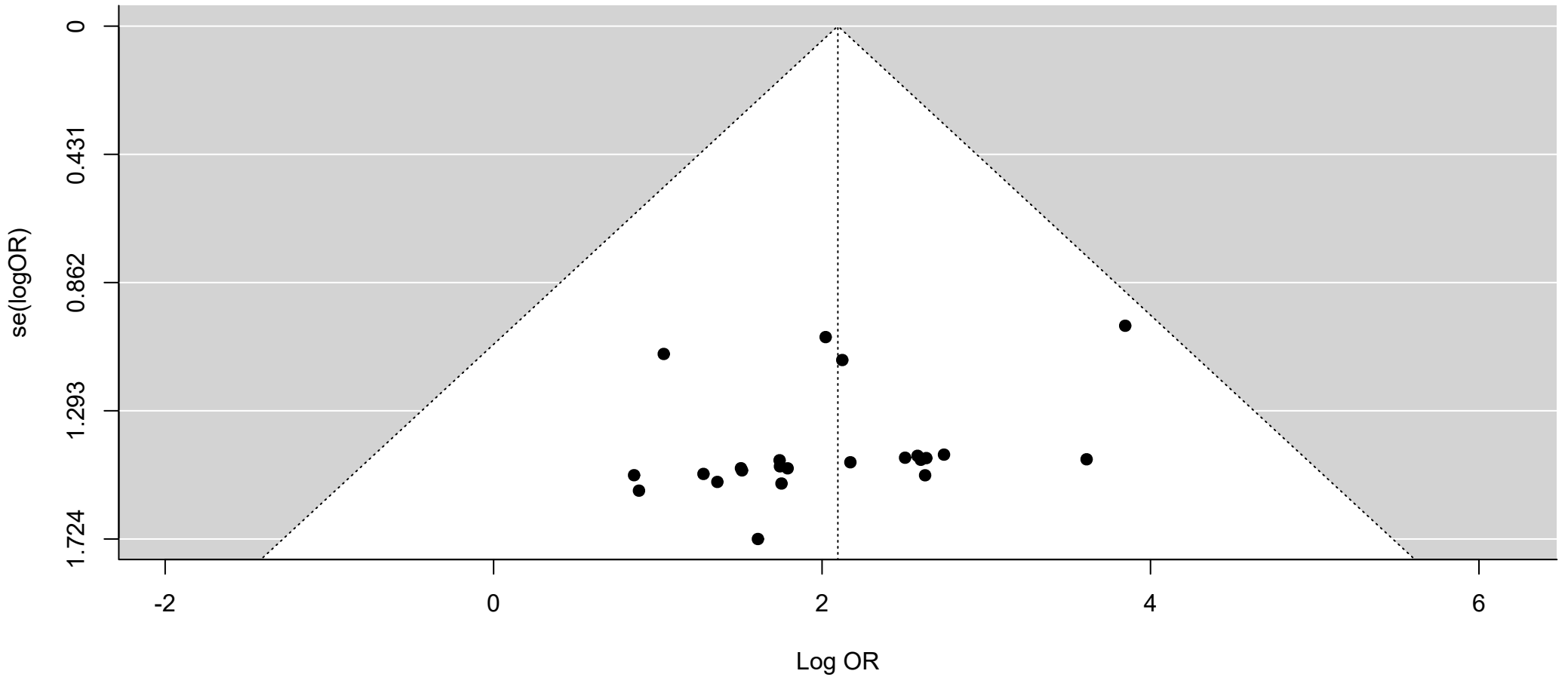
Funnel plot with pseudo 95% confidence limits
