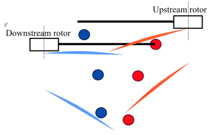
Highest thrust: Upstream tip vortex aligns near the downstream blade.
