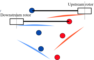
Lowest thrust: Wake structures convect downstream without interaction.
