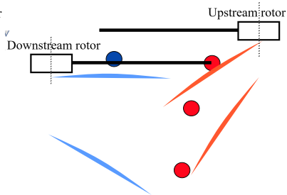
Intermediate thrust: Upstream tip vortex impinges and dissipates on the downstream blade.
