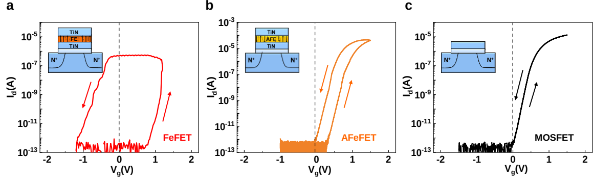
Supplementary Figure 1. Volatility of AFeFET. a Typical transfer curves of FeFET. b Typical transfer curves of AFeFET. c Typical transfer curves of MOSFET. The sweeping DC voltage is applied to the gate of FeFET, and 0.3 V DC voltage is applied to the drain terminal during measurement. The arrows indicate the switching sequences. Compared to MOSFET, both the transfer curves of FeFET and AFeFET exhibit counterclockwise hysteresis due to the polarization switching of \text{Hf}_x\text{Zr}_{1-x}\text{O}_2 films under the electric field. But the transfer curve of AFeFET differs from that of FeFET at V_G=0 V, indicating that the AFeFET is volatile. Moreover, the AFeFET is electroforming-free.
