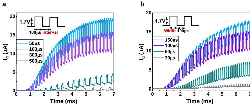
Supplementary Figure 6. The tendencies of I_d under continuous gate pulses with different gate pulse parameters. a Different gate pulse intervals (fixed 1.7 V amplitude, 50 \mu s -500 \mu s interval, fixed 100 \mu s width). The I_d increases faster and a larger saturation value in the case of shorter pulse intervals, as shorter intervals will limit the recover duration of AFE domains and contribute to the I_d increase. b Different gate pulse widths (fixed 1.7 V amplitude, fixed 100 \mu s interval, 30 \mu s -150 \mu s width). The larger pulse width corresponds to a larger I_d saturation value due to more AFE t -phase domains can be switched to FE domains under longer integration time.
