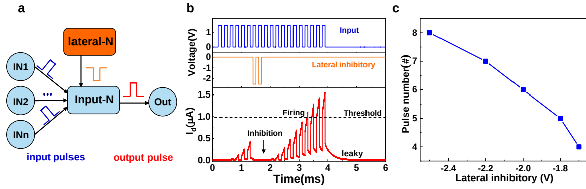
Supplementary Figure 8. The lateral inhibitory property of AFeFET neuron. a Schematic illustration of the lateral inhibitory. Negative gate pulses as inhibitory stimuli from adjacent neurons are applied during a series of excitatory input spikes (100 \mu s width, 100 \mu s interval, 1.5 V amplitude). b The response of AFeFET neuron to inhibitory stimuli. The excitability is inhibited once receiving inhibitory stimuli (100 \mu s width, 100 \mu s interval, -2.5 V amplitude) from adjacent neurons. After inhibition, the AFeFET neuron gets excitive again and fires under the continuous excitatory stimuli. c The pulse number for the next firing after receiving different inhibitory stimuli (-1.7 V, -1.8 V, -2 V, -2.2 V, -2.5 V). The AFeFET neuron needs more excitatory stimuli for the next firing with stronger inhibitive intensity.
