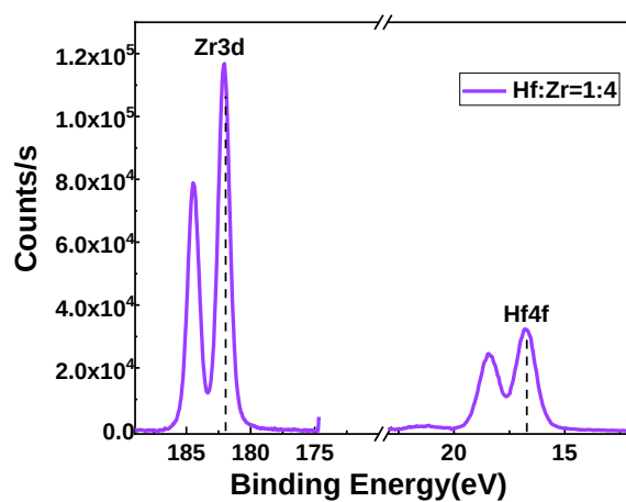
Supplementary Figure 4. The XPS results of \text{Hf}_{0.2}\text{Zr}_{0.8}\text{O}_2 . The AFE \text{Hf}_x\text{Zr}_{1-x}\text{O}_2 film composition is confirmed as hafnium: zirconium \approx 1:4 .
