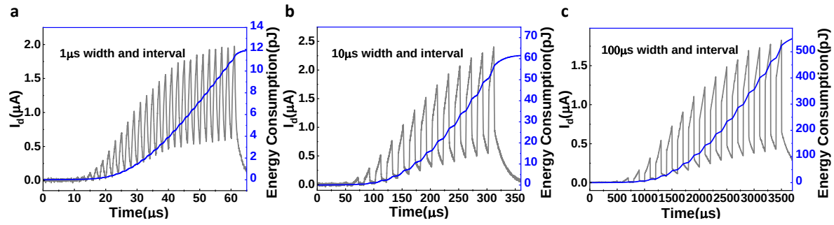
Supplementary Figure 9. The energy consumption per spike dependence on pulse parameters and the threshold value of AFeFET neurons. The energy consumption of AFeFET neurons with a 1 μs b 10 μs c 100 μs gate pulse width and interval. The energy consumption E_{\text{AFeFET}} is achieved by accumulating I_d V_{\text{ds}} \Delta t , the V_{\text{ds}} is 0.3V during measurement. With the reduction of pulse width or threshold value, the energy consumption decreases and the measured lowest energy consumption is 37 fJ per spike (1 μs width and interval, 50 nA threshold). The energy consumption can be further reduced as pulse width and threshold decreasing.
