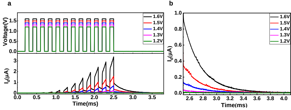
Supplementary Figure 7. The leakage process of AFeFET neuron with different I_d . a
