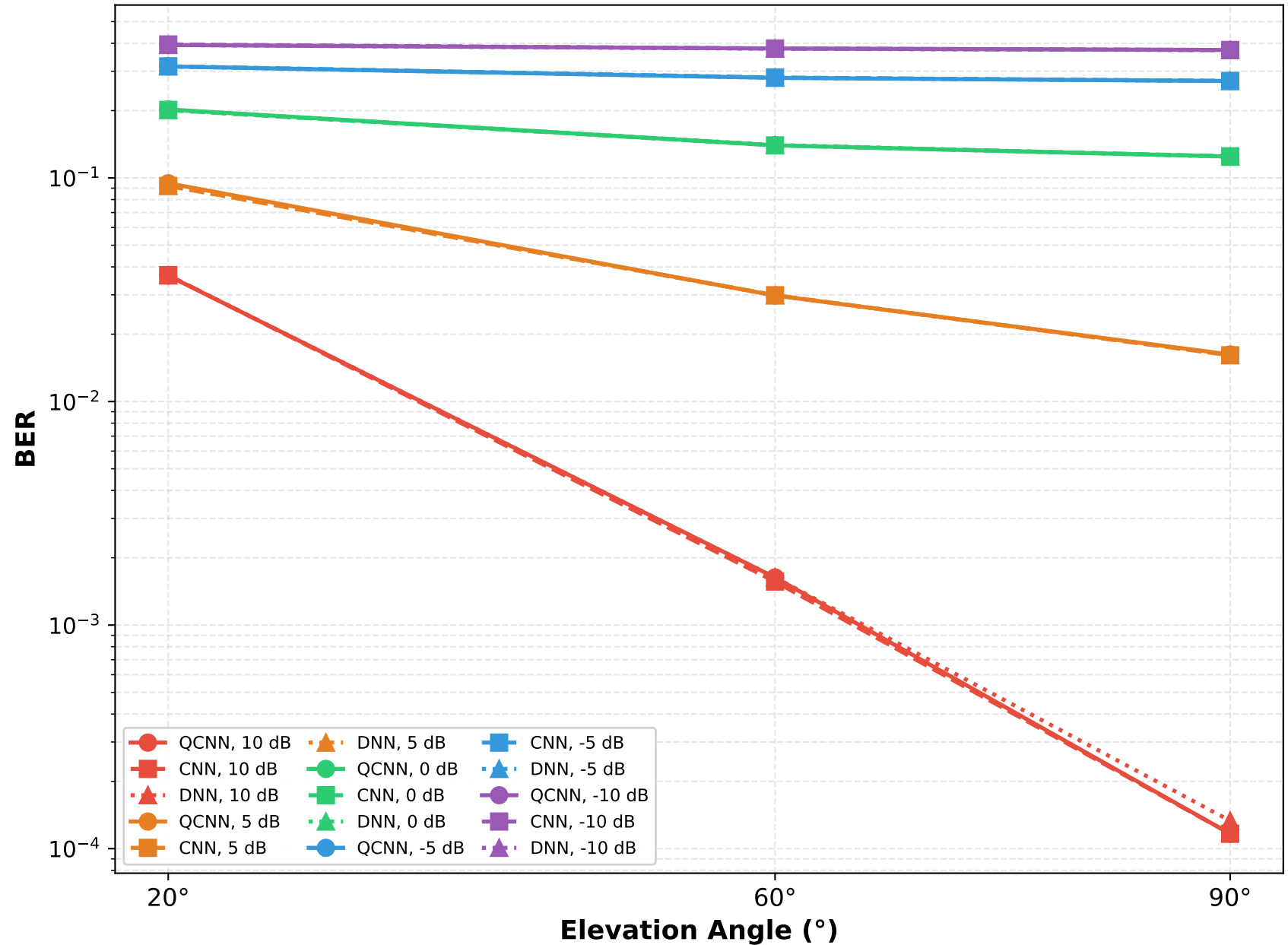
BER vs Elevation Angle (Log Scale)
