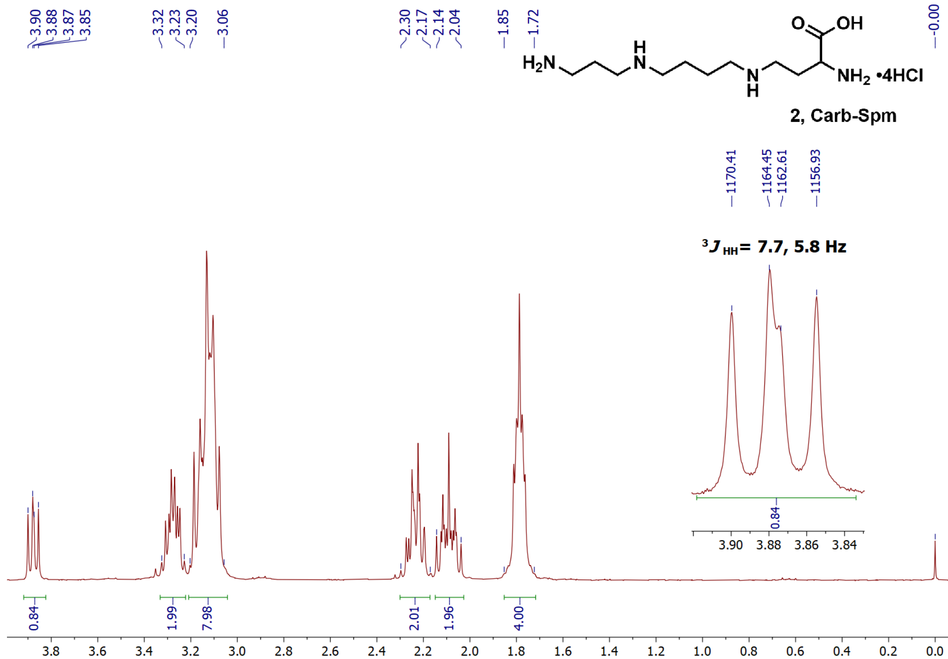
Figure S6. ^1\text{H} NMR spectrum of Carb-Spm, 2 .
