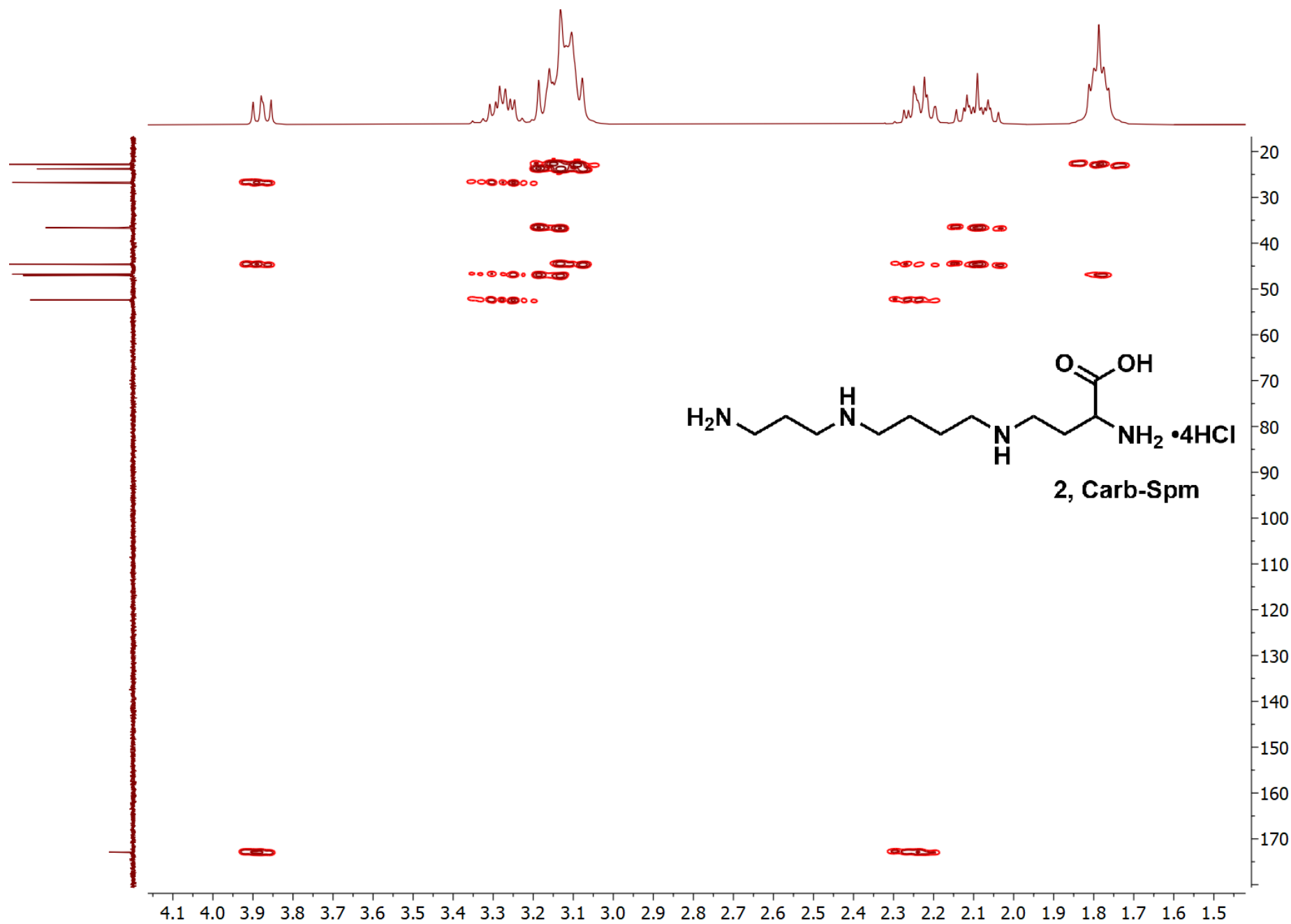
Figure S10. HMBC spectrum of Carb-Spm, 2.
