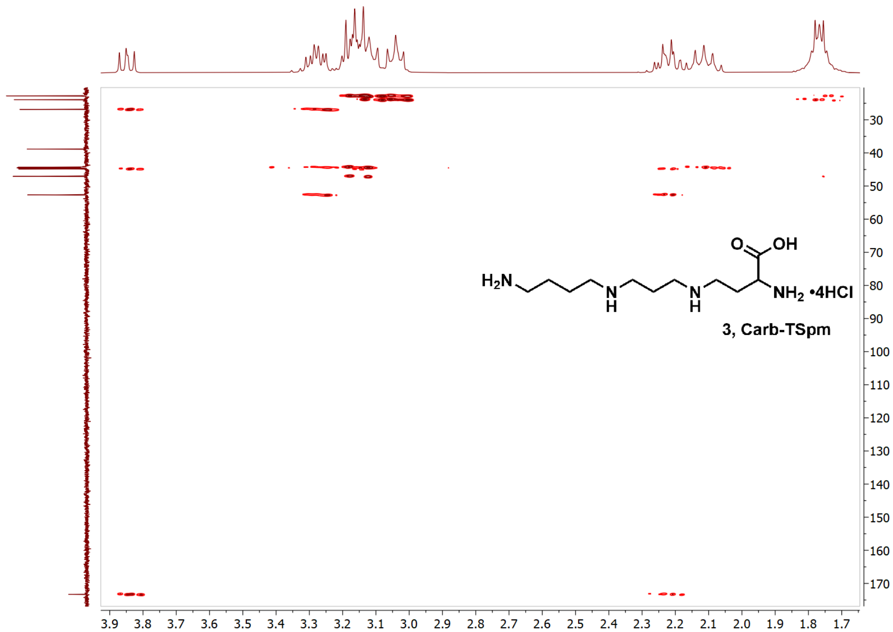
Figure S15. HMBC spectrum of Carb-TSpm, 3 .
