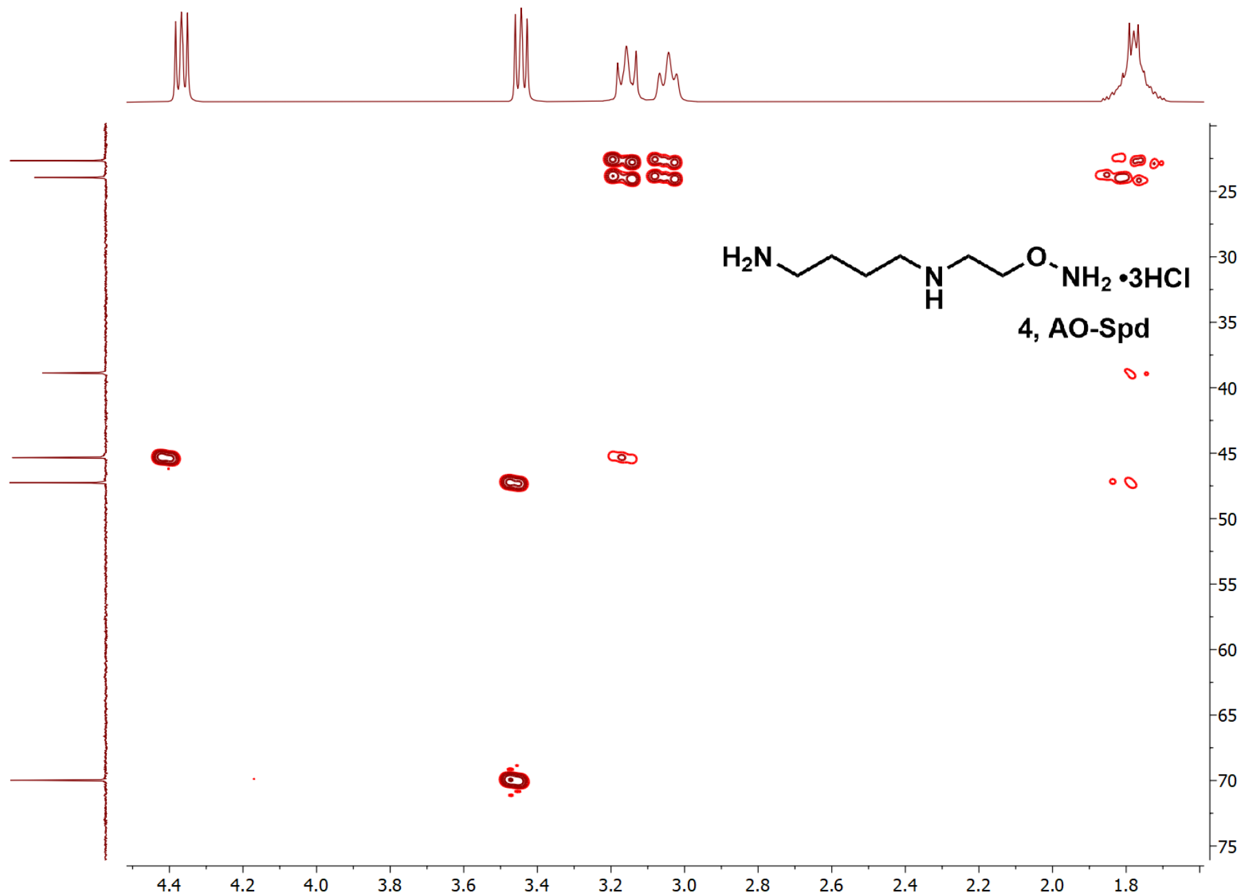
Figure S20. HMBC spectrum of AO-Spd, 4 .
