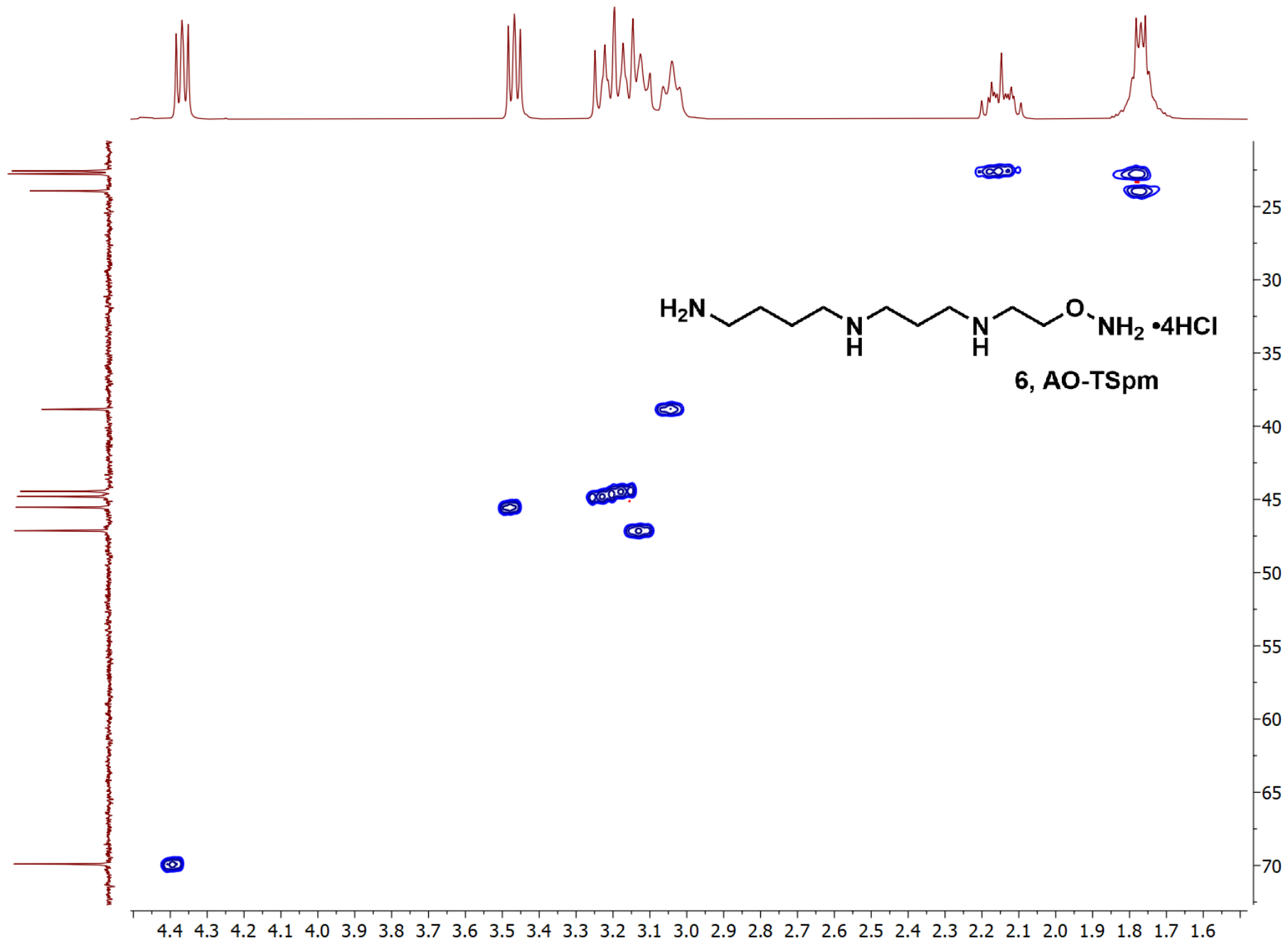
Figure S29. HSQC spectrum of AO-TSpM, 6.
