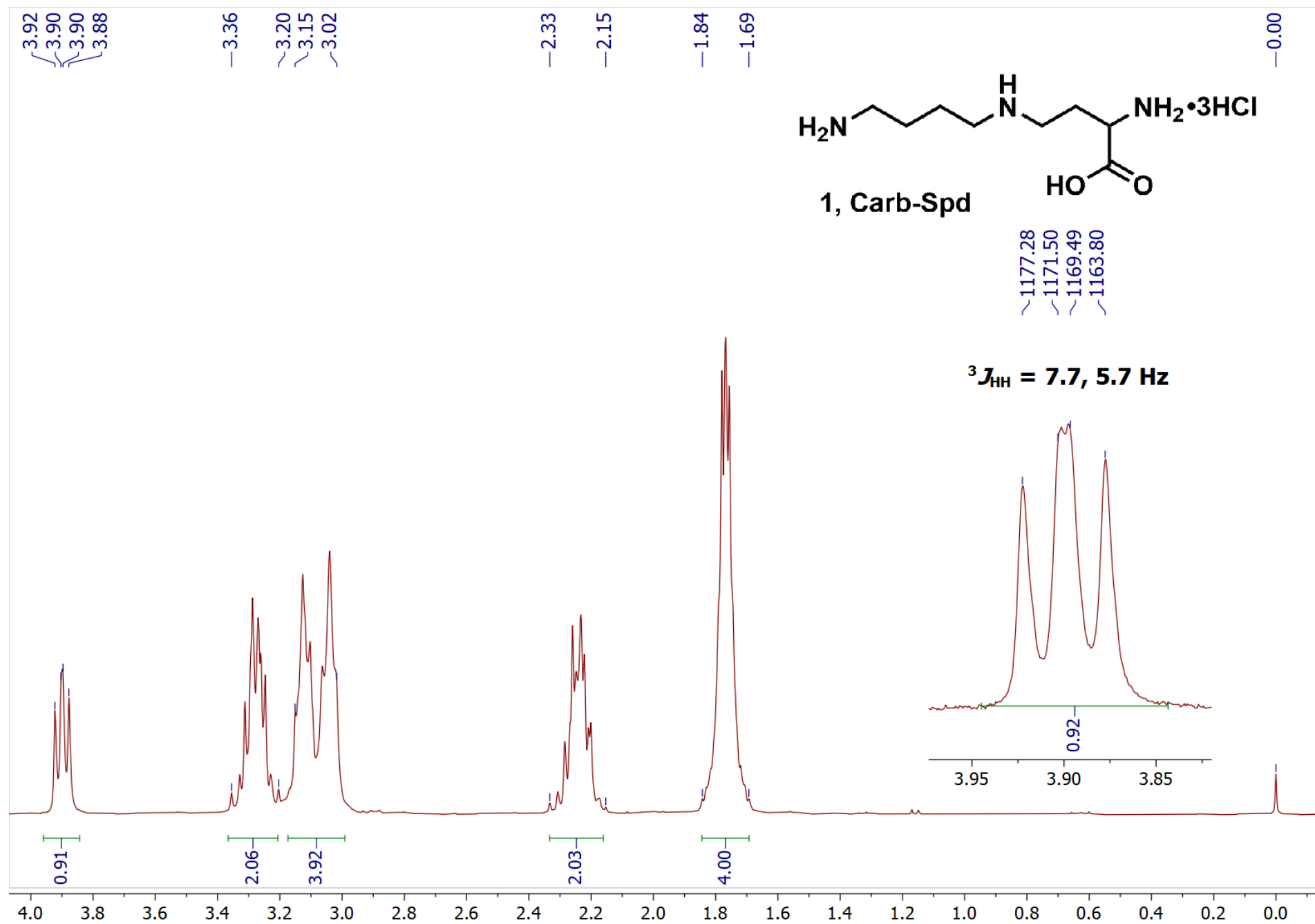
Figure S1. ^1\text{H} NMR spectrum of Carb-Spd, 1 .
