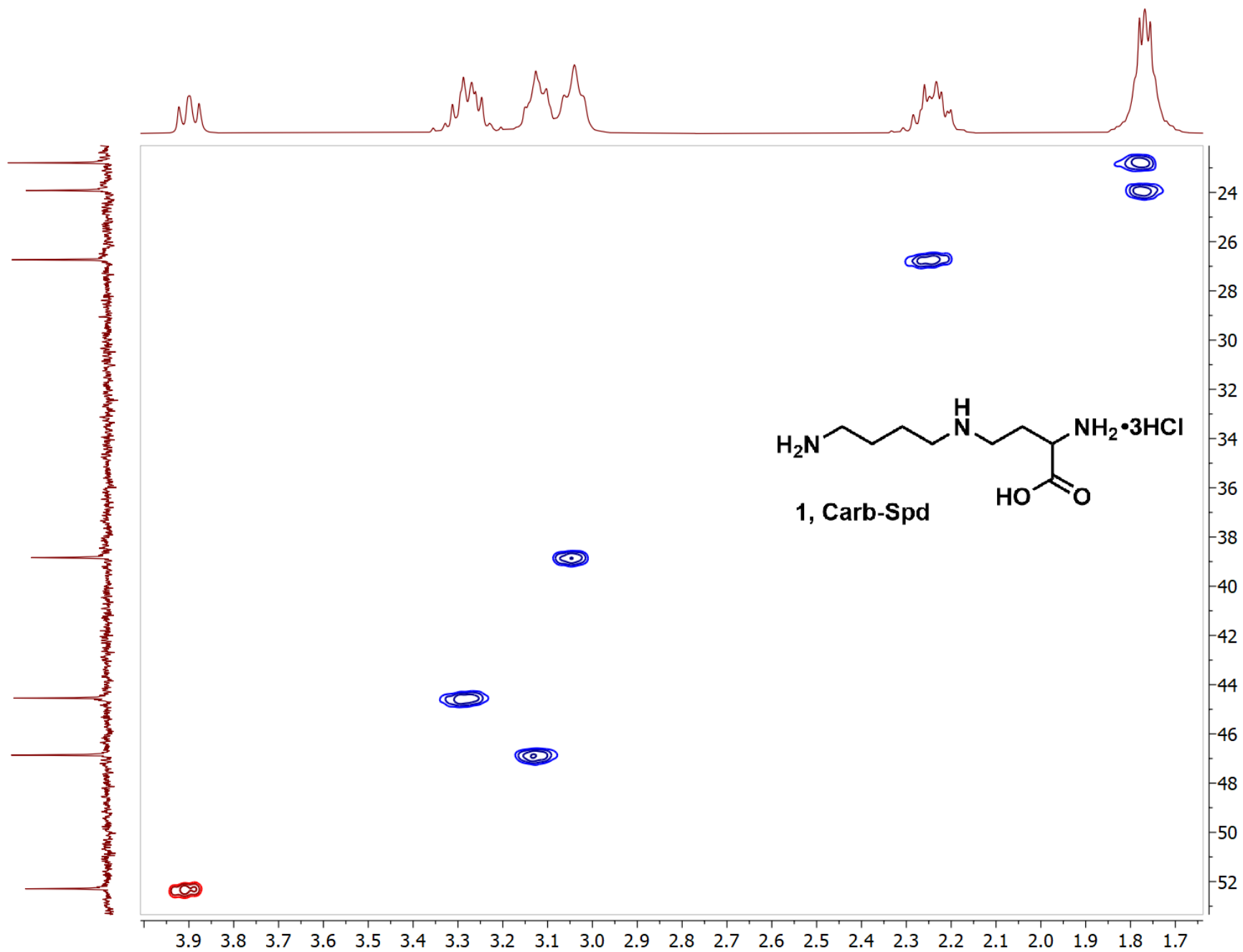
Figure S4. HSQC spectrum of Carb-Spd, 1.
