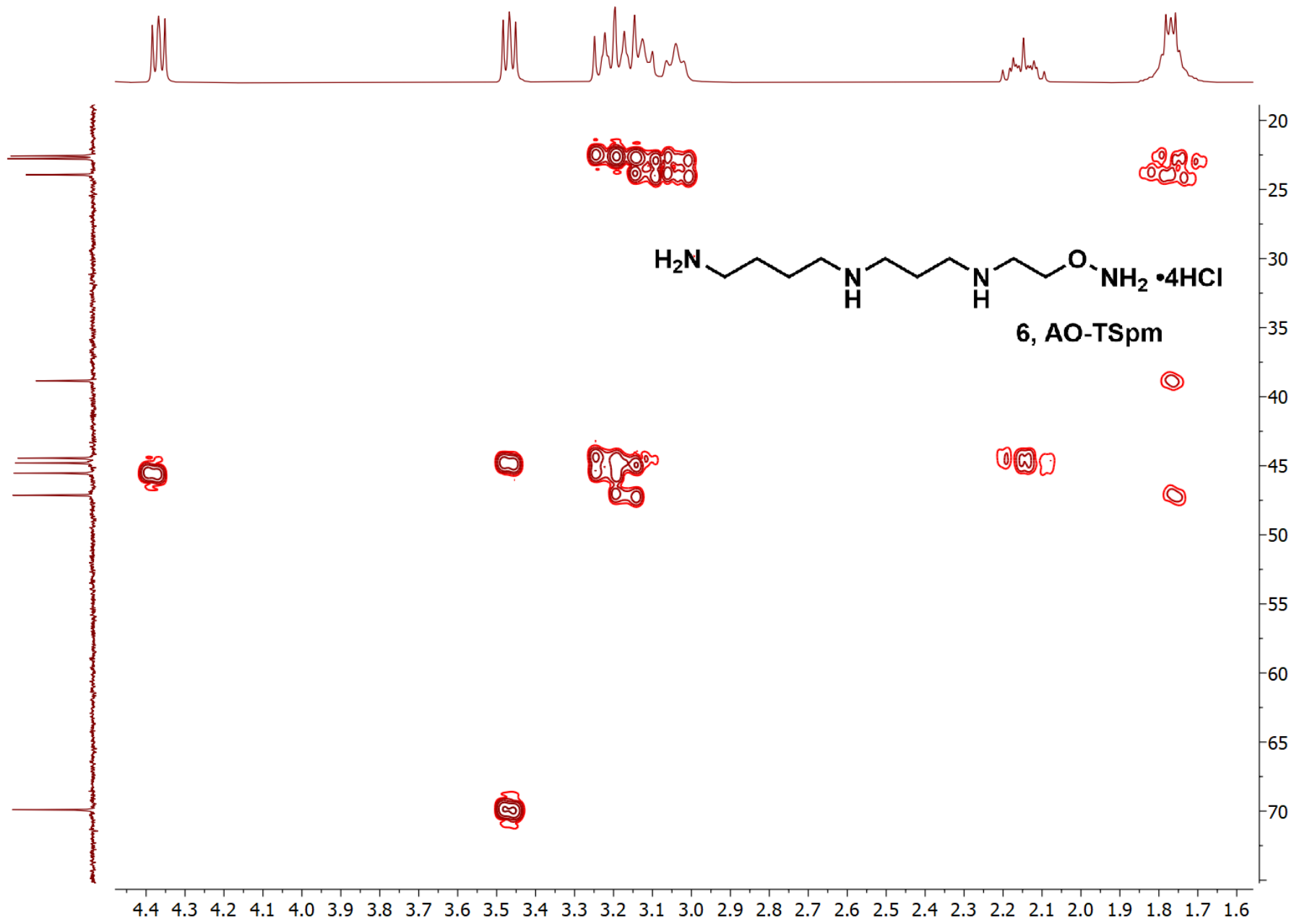
Figure S30. HMBC spectrum of AO-TSpM, 6.
