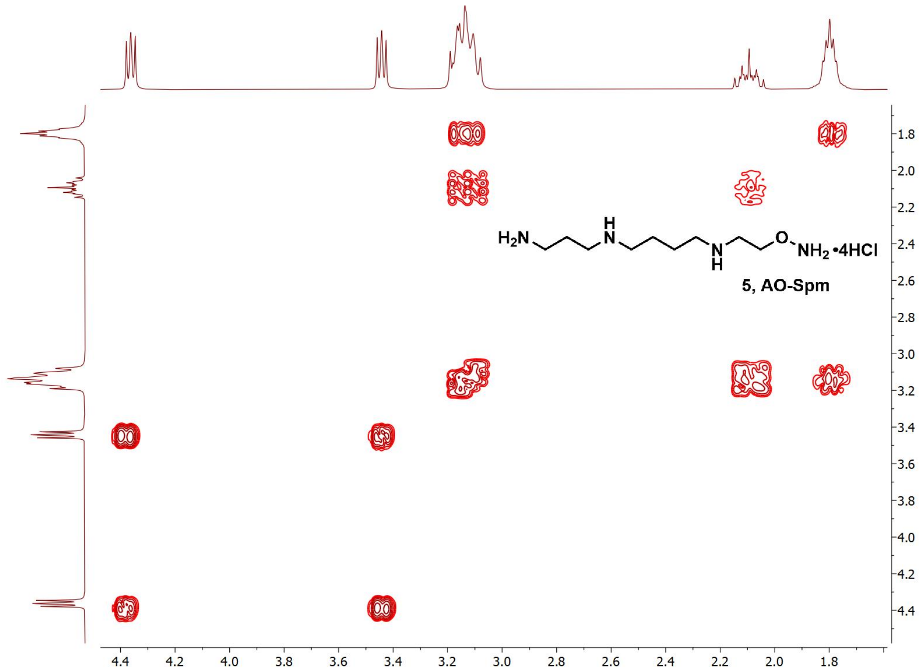
Figure S23. COSY spectrum of AO-Spm, 5.
