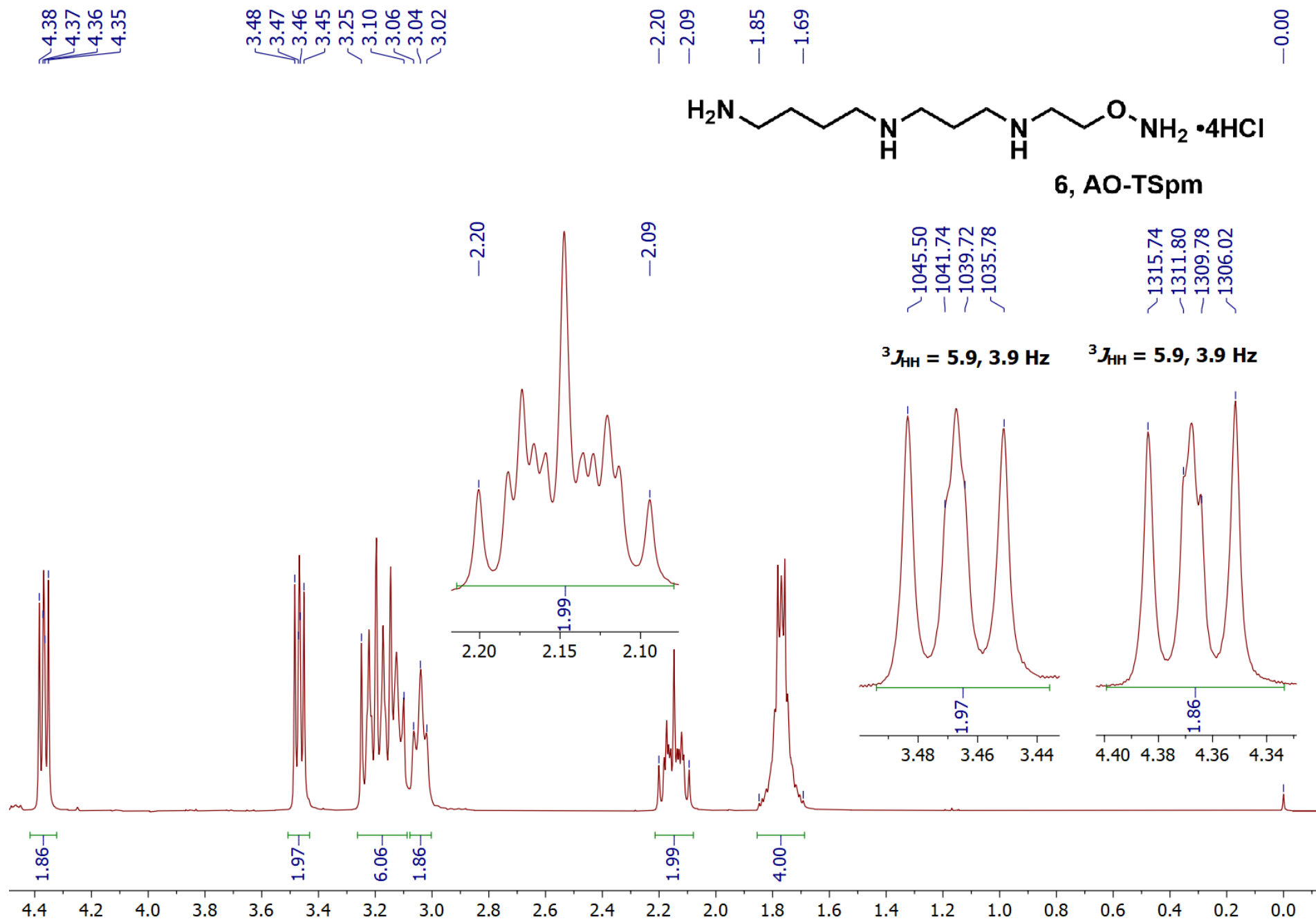
Figure S26. ^1\text{H} NMR spectrum of AO-TSpm, 6 .
