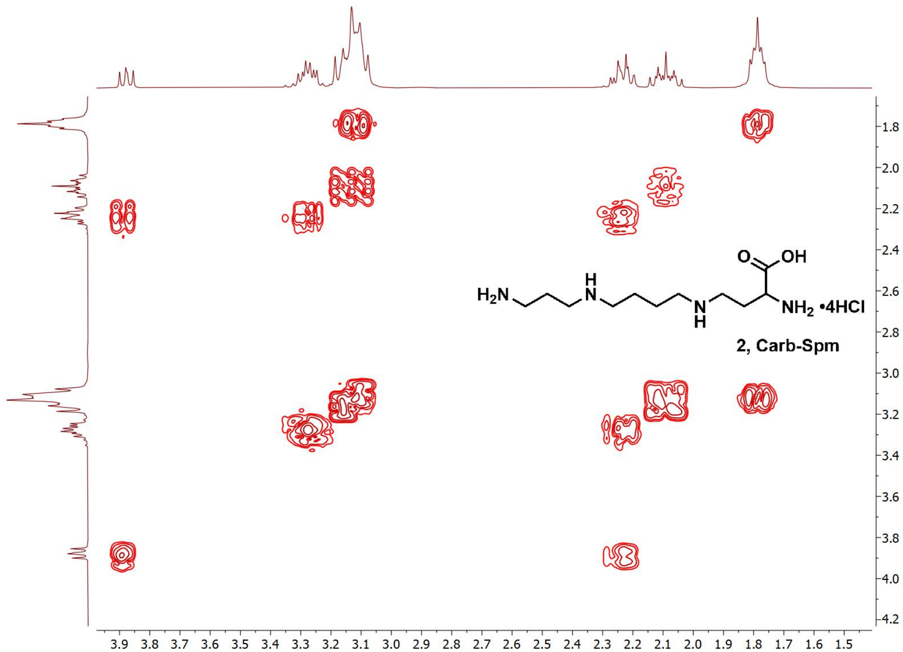
Figure S8. COSY spectrum of Carb-Spm, 2 .
