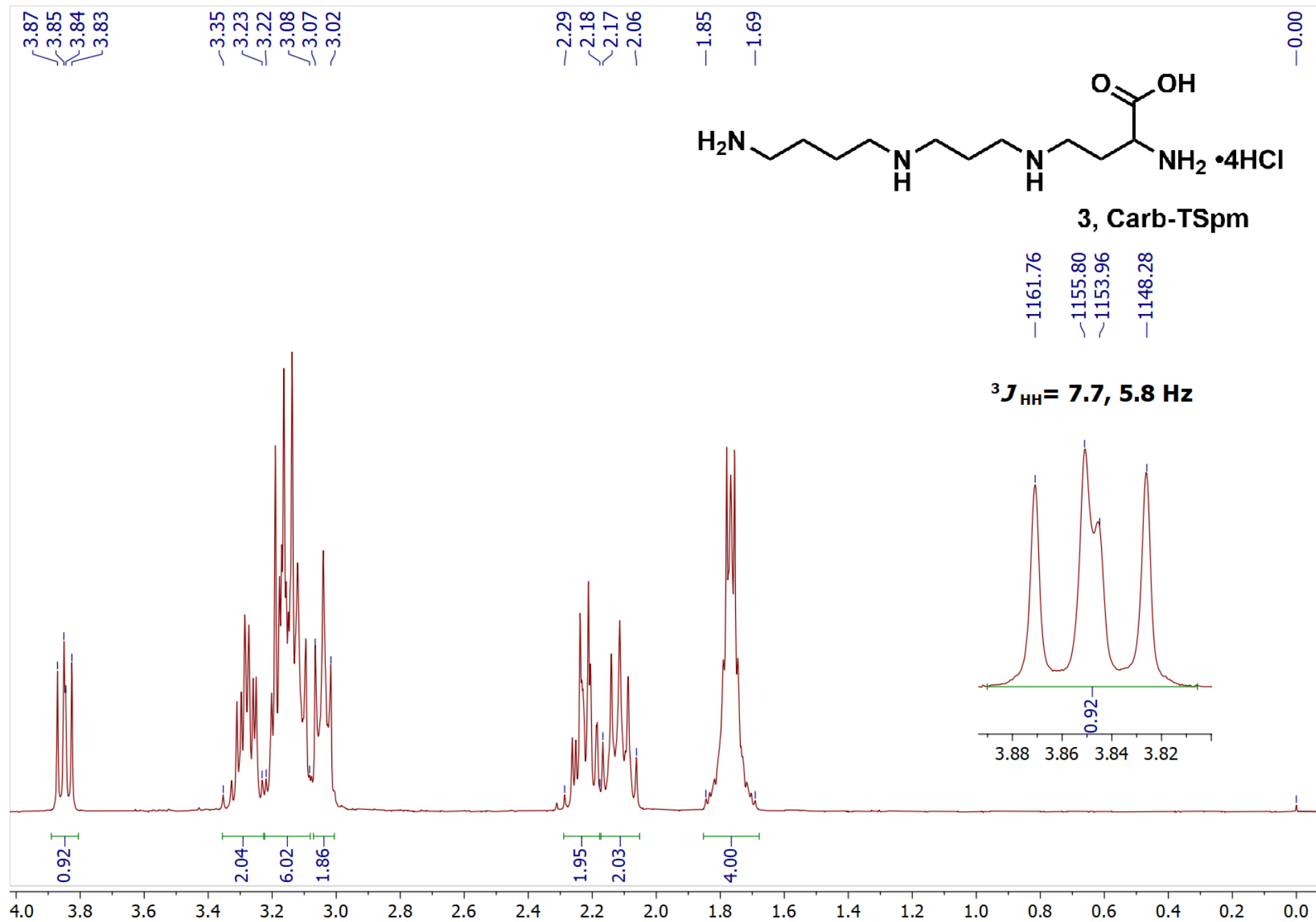
Figure S11. ^1\text{H} NMR spectrum of Carb-TSpm, 3 .
