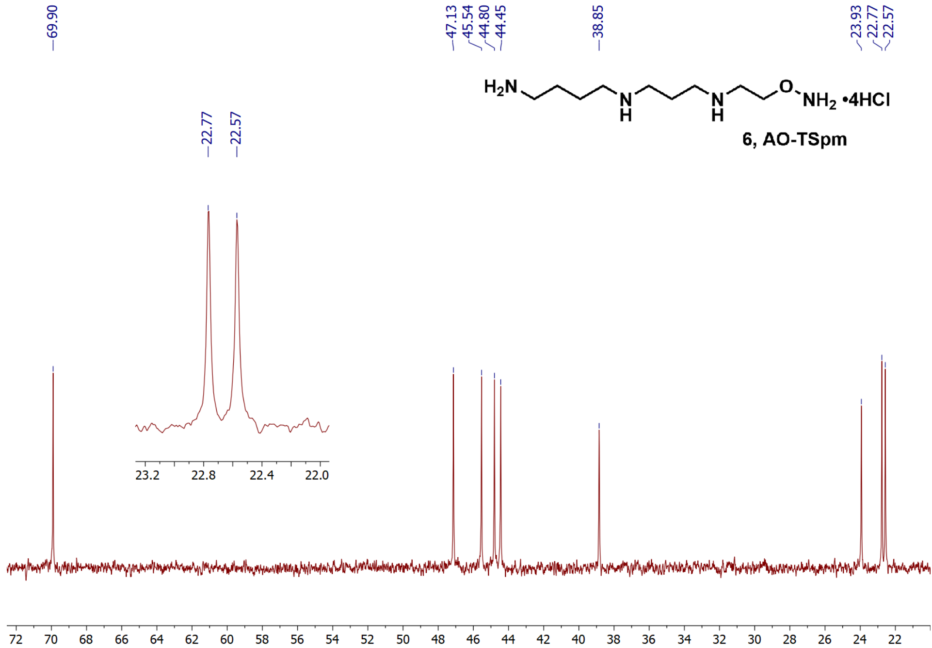
Figure S27. ^{13}\text{C} NMR spectrum of AO-TSpM, 6.
