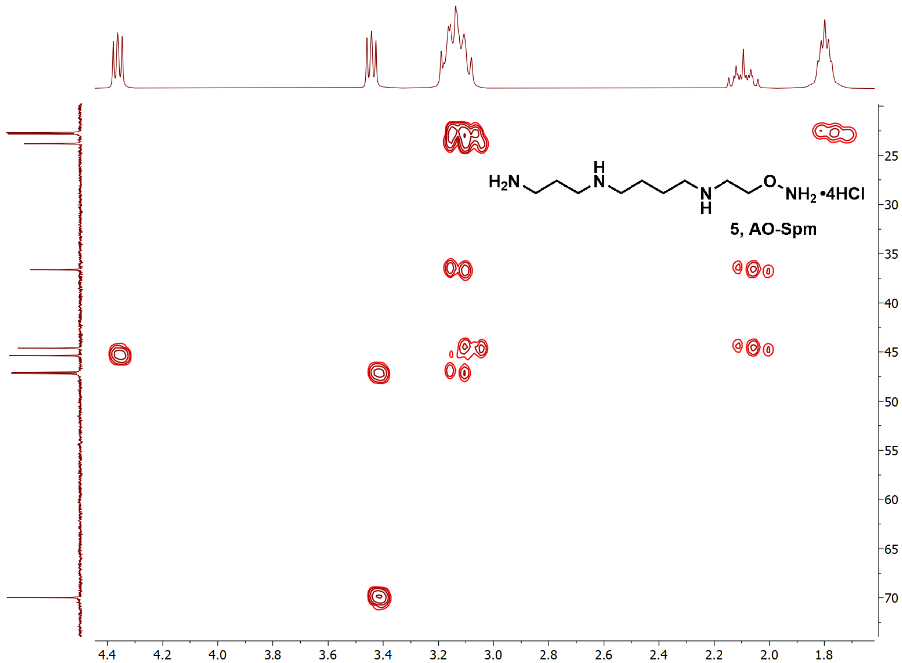
Figure S25. HMBC spectrum of AO-Spm, 5 .
