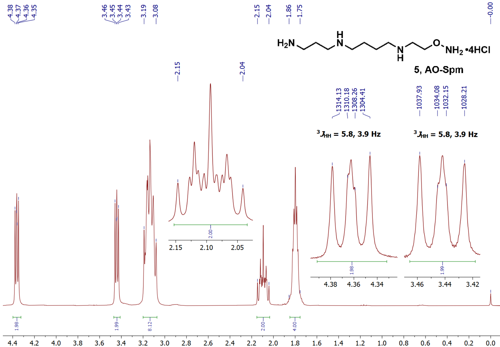
Figure S21. ^1\text{H} NMR spectrum of AO-Spm, 5 .
