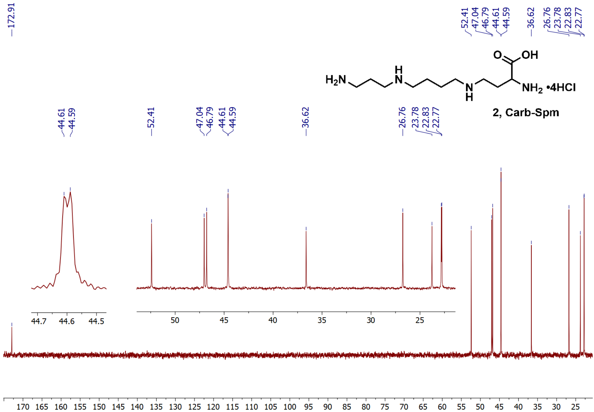
Figure S7. ^{13}\text{C} NMR spectrum of Carb-Spm, 2 .
