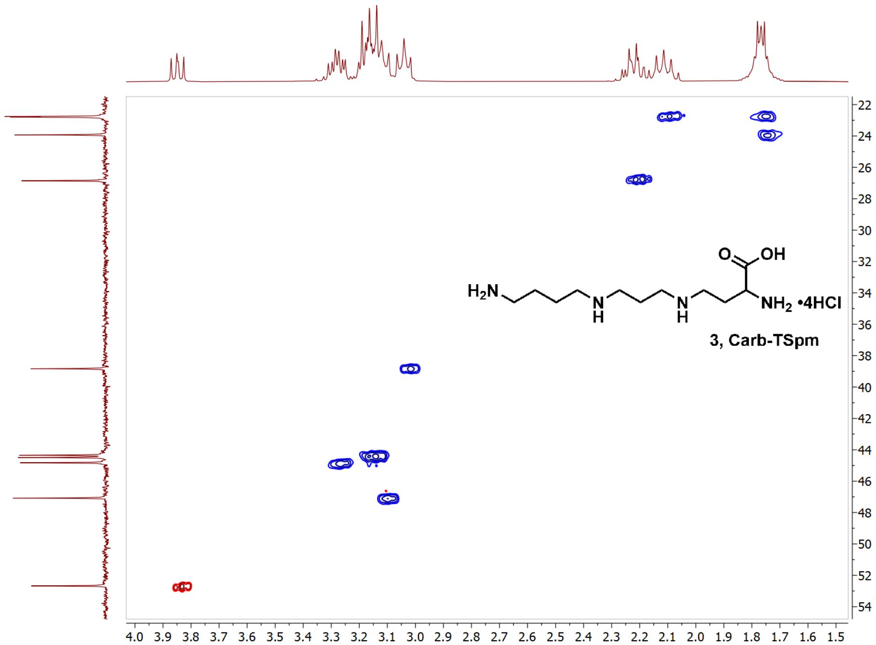
Figure S14. HSQC spectrum of Carb-TSpm, 3 .
