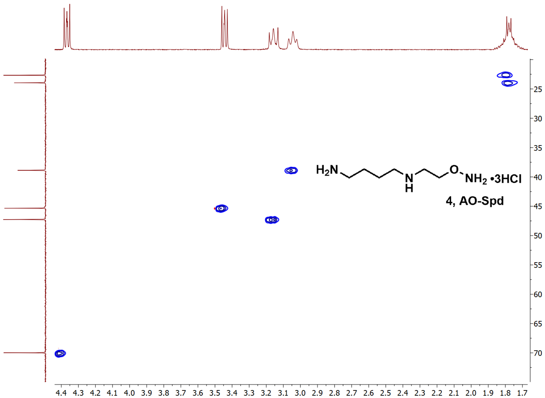
Figure S19. HSQC spectrum of AO-Spd, 4.
