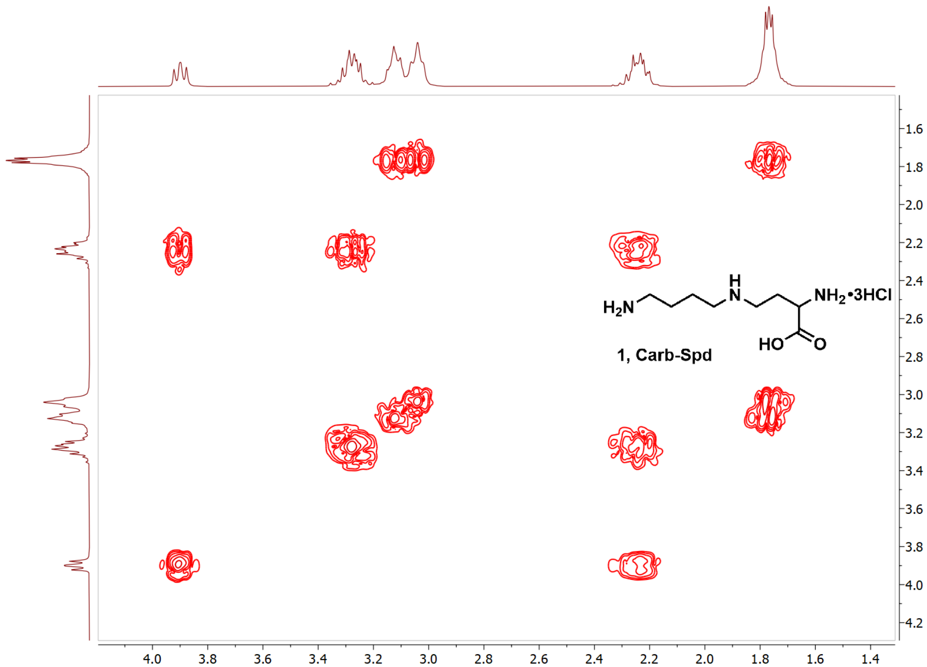
Figure S3. COSY spectrum of Carb-Spd, 1 .
