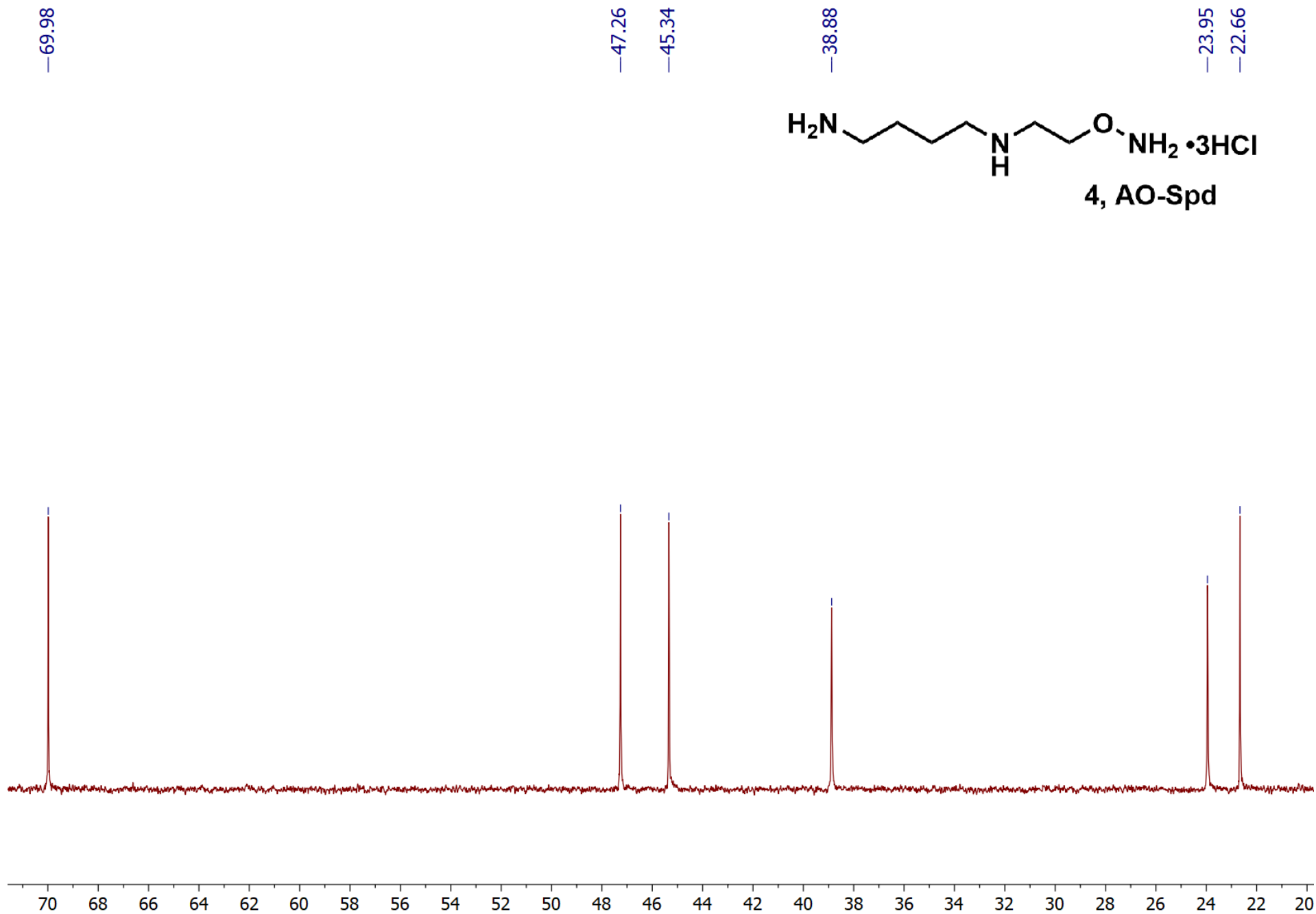
Figure S17. ^{13}\text{C} NMR spectrum of AO-Spd, 4.
