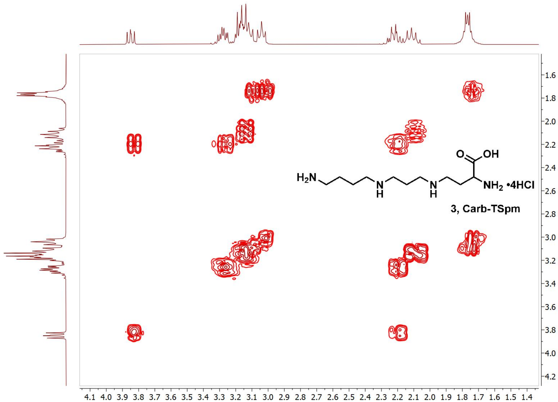
Figure S13. COSY spectrum of Carb-TSpm, 3 .
