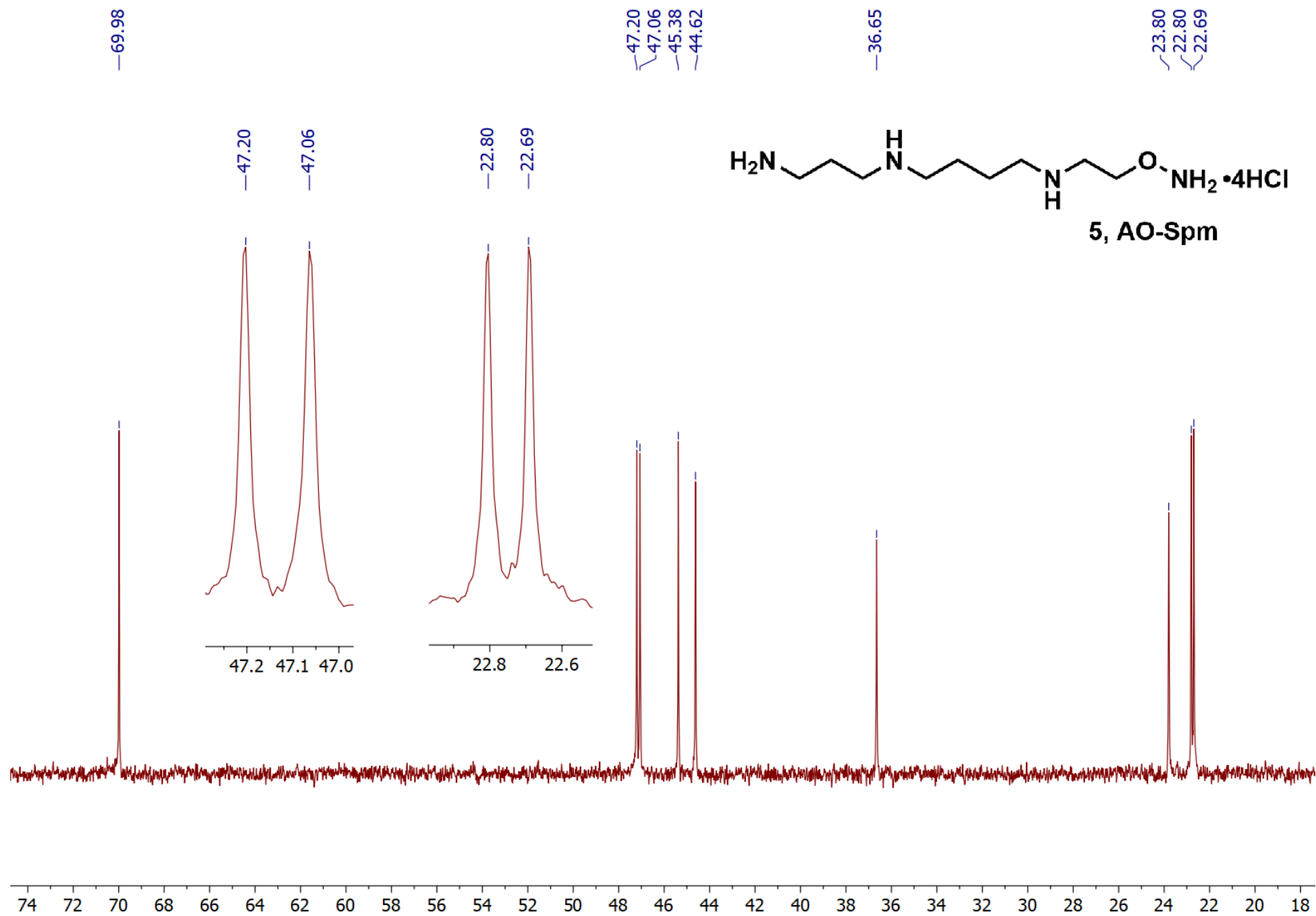
Figure S22. 13 C NMR spectrum of AO-Spm, 5 .
