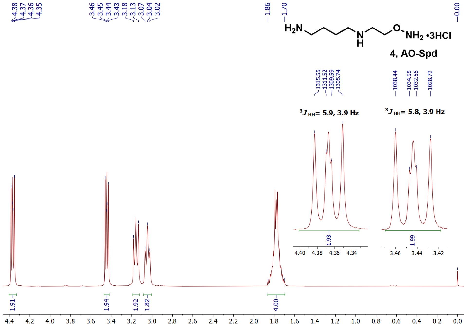
Figure S16. 1 H NMR spectrum of AO-Spd, 4 .
