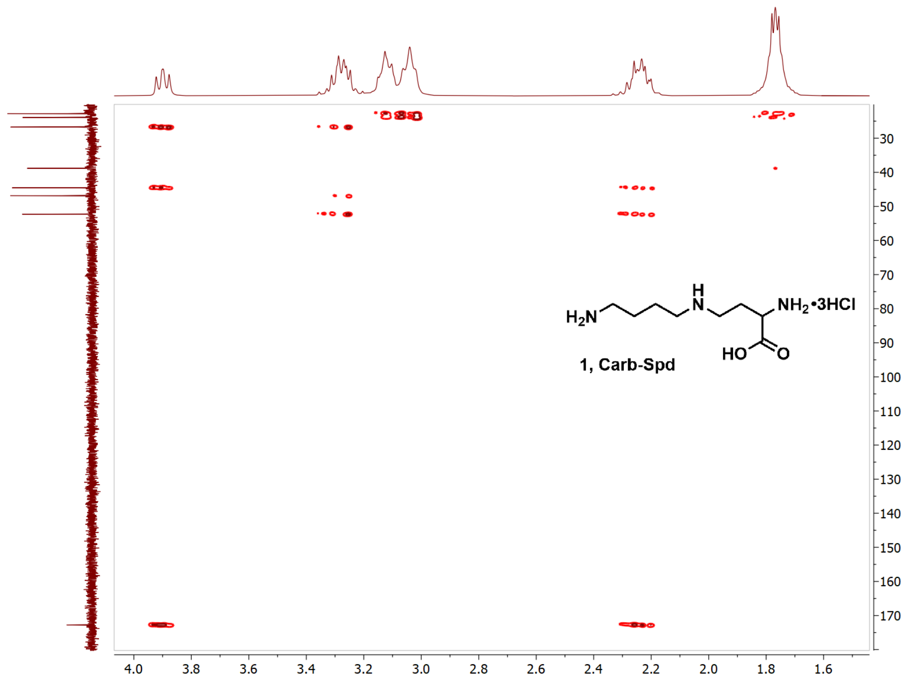
Figure S5. HMBC spectrum of Carb-Spd, 1.
