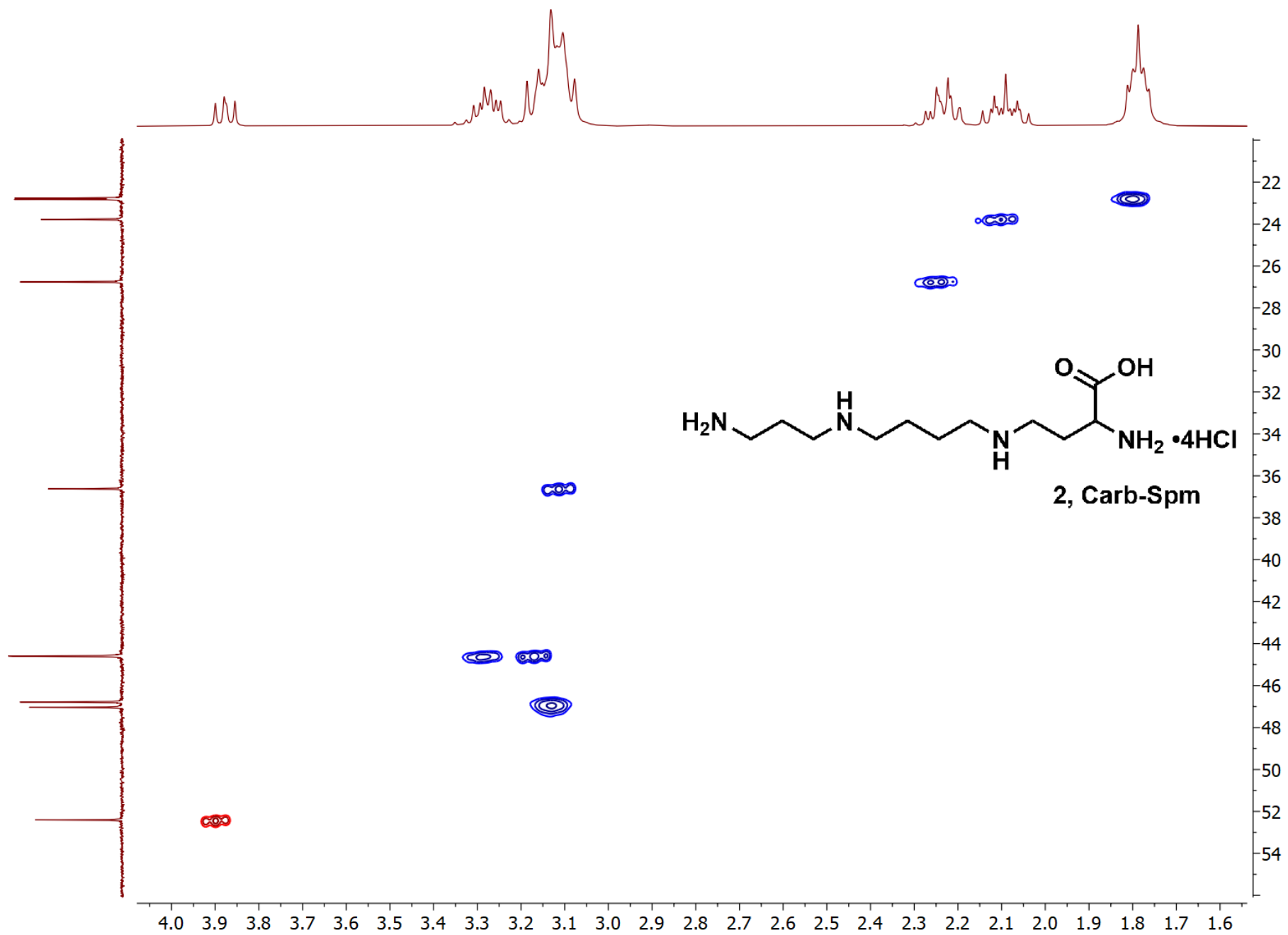
Figure S9. HSQC spectrum of Carb-Spm, 2.
