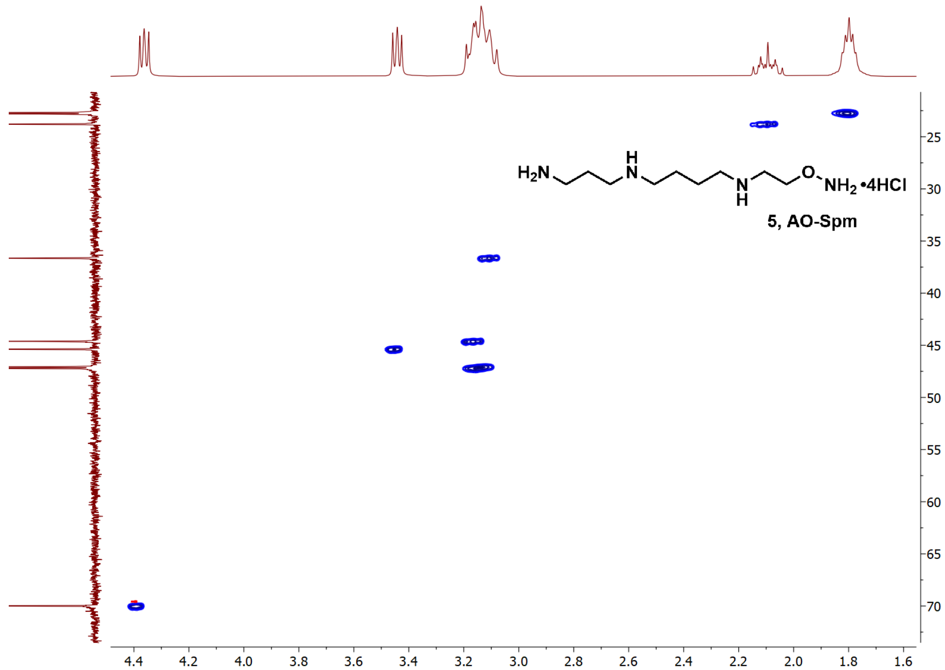
Figure S24. HSQC spectrum of AO-Spm, 5.
