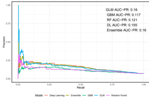
Precision-Recall Curve Comparison
