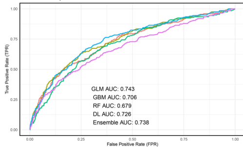
ROC Curve Comparison
