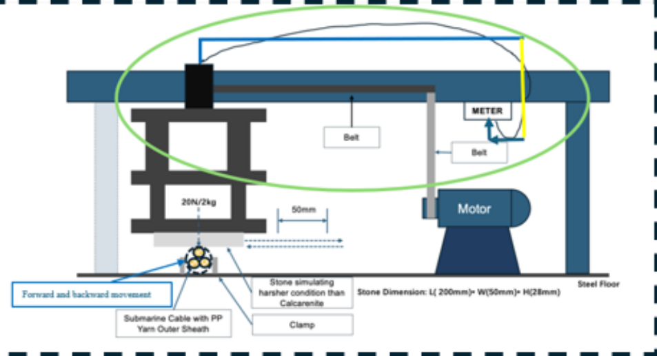
Abrasive device : Test Set-up
