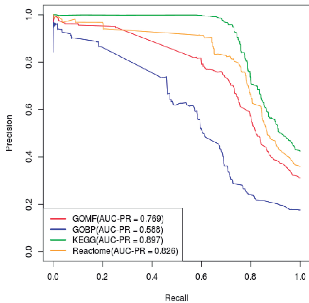
(g) Simpson
