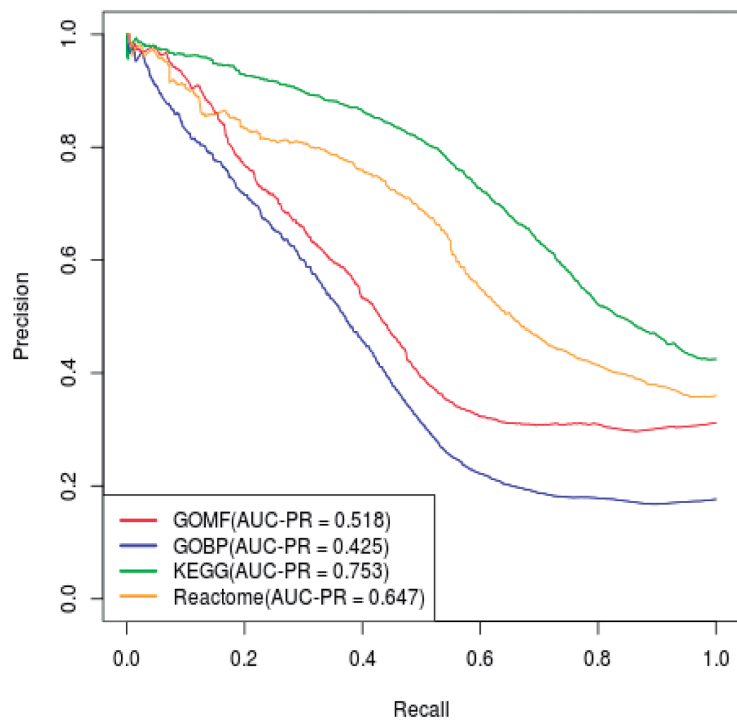
(e) PCC
