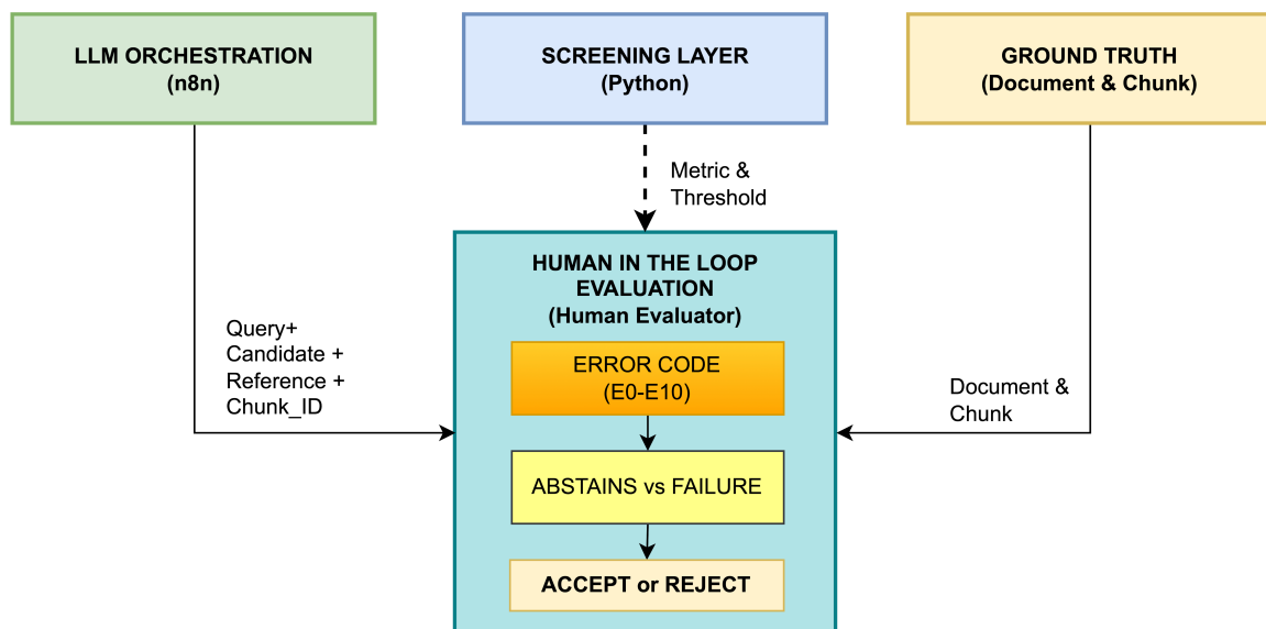
Figure 4. HITL Evaluation Artifact and Annotation Schema.
