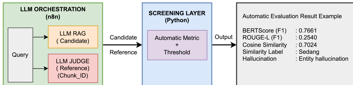
Figure 3. Automatic Screening Layer with Metric and Thresholds.
