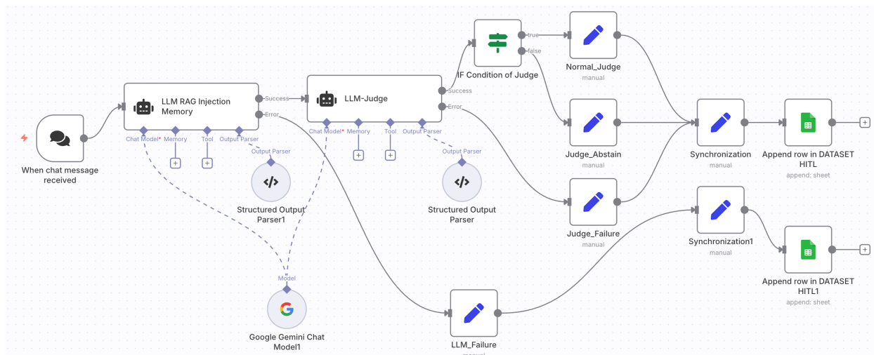
Figure 3. n8n Workflow Orchestration for Candidate, Reference Generation, and Chunk_ID Retrieval.
