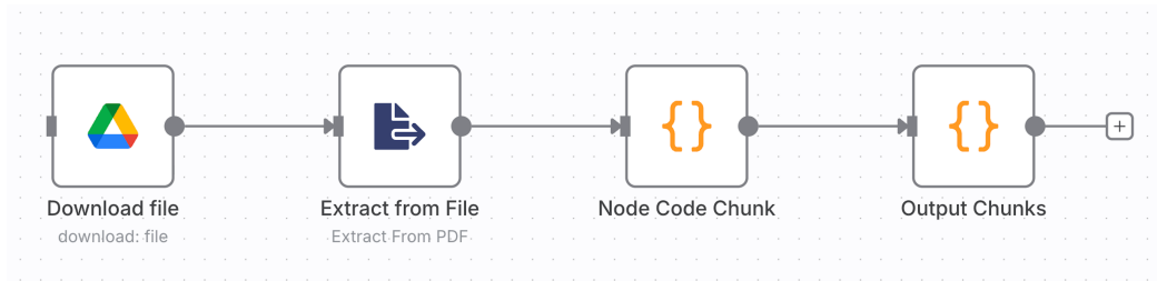
Figure 2. Chunk Generation for RAG Memory Injection.
