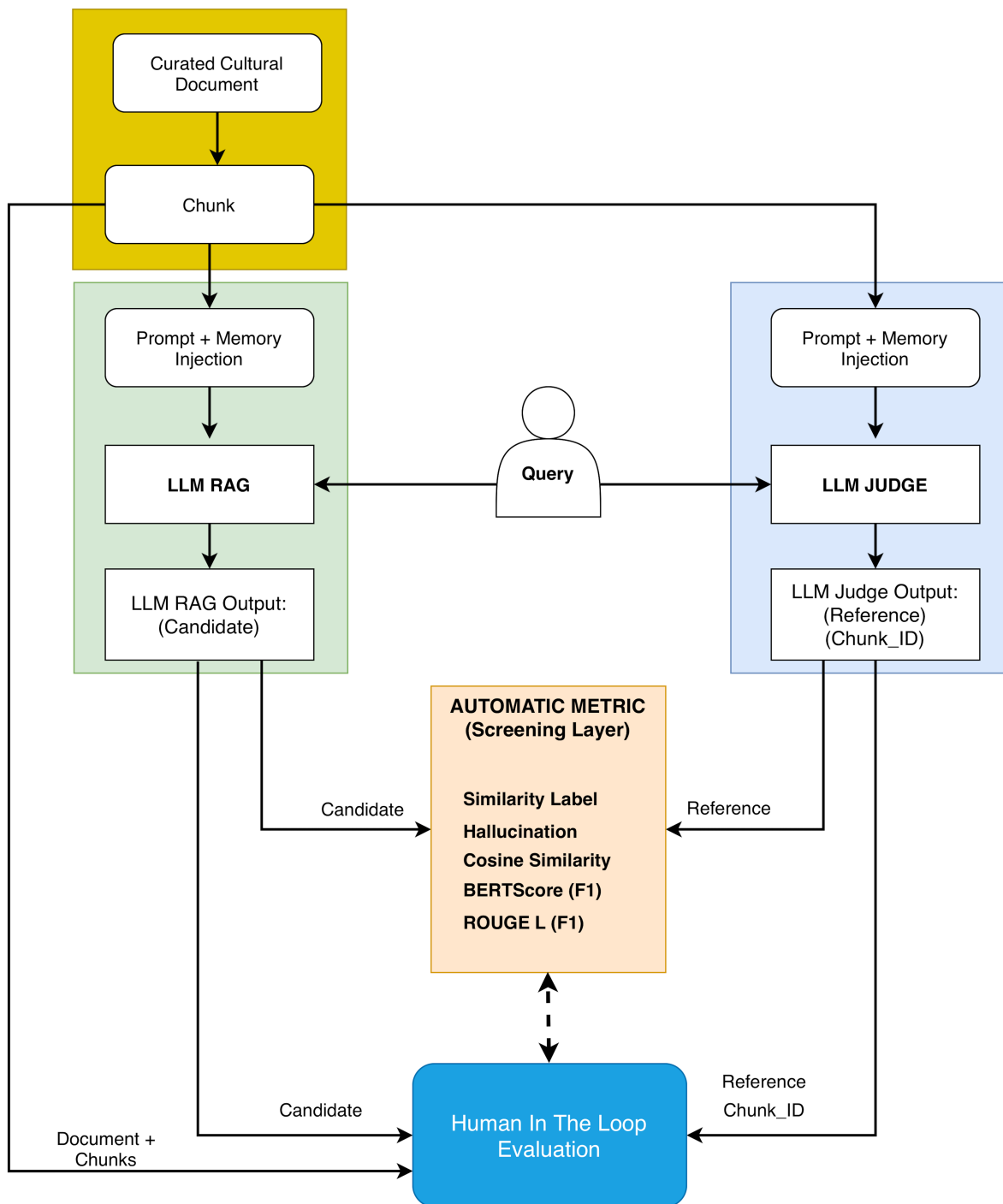
Figure 1. HITL-RAG Evaluation Framework.
