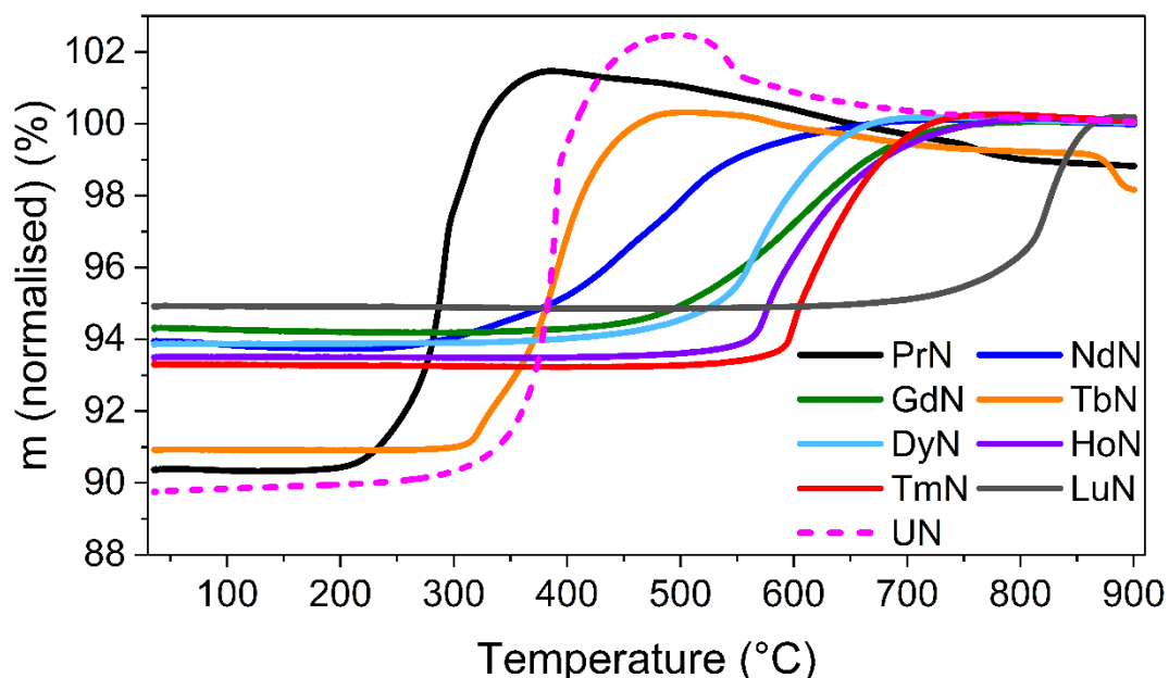
Figure 8. TGA profiles for investigated \text{LnN} ( \text{Ln} = \text{Pr}, \text{Nd}, \text{Gd}, \text{Tb}, \text{Dy}, \text{Ho}, \text{Tm}, \text{Lu} ) and UN samples heated to 900 °C in synthetic air, normalised to the endpoint of the measurements.
