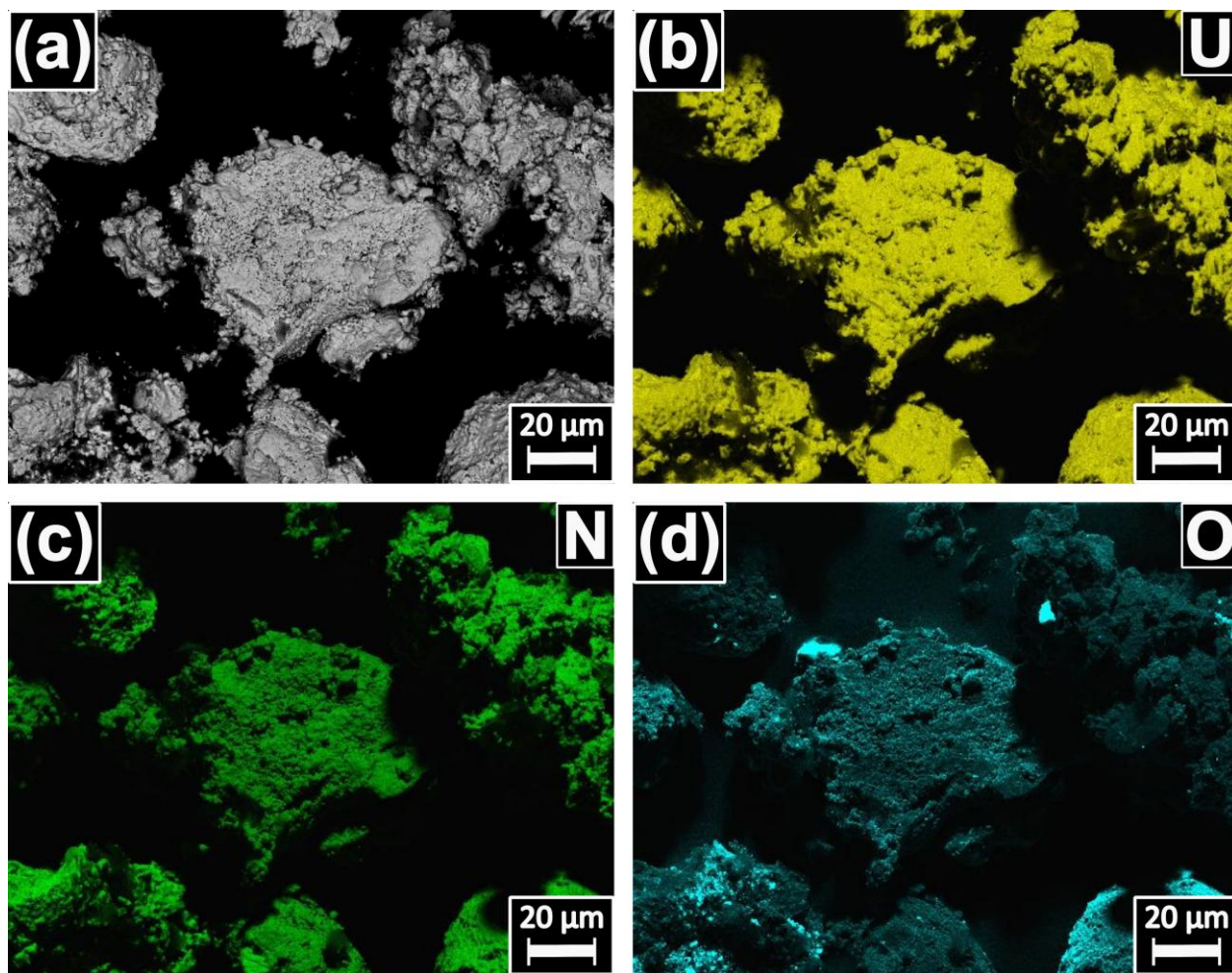
Figure 6. SEM-EDS elemental maps of oxidised UN a) BSE image b) U-M map c) N-K map d) and O-K map. High intensity O spots correlate with impurities (cross contamination), for further details check Supplementary Note 2, Figure S9 and Figure S10.
