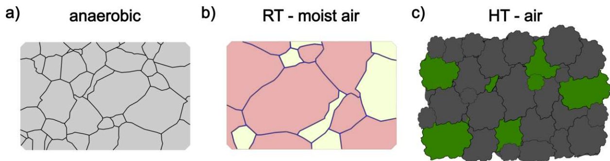
Figure 10. Graphical illustration of a) Ln -doped UN single phase microstructure expected to occur in irradiated UN fuel under anaerobic conditions, b) Ln -doped UN multiphase microstructure expected to occur when irradiated UN fuel is exposed to atmospheric conditions (RT) – wet oxidation; room temperature air and moisture, showing phase separation of \text{UO}_2 (red), \text{Ln}(\text{OH})_3 (yellow) and \text{U}_2\text{N}_3 (blue lines) and c) Ln -doped UN multiphase microstructure of irradiated UN fuel is exposed to high temperature (HT) oxidising conditions, showing formation of expanded particles of \text{U}_3\text{O}_8 (dark gray) and \text{Ln}_2\text{O}_3 (green).
