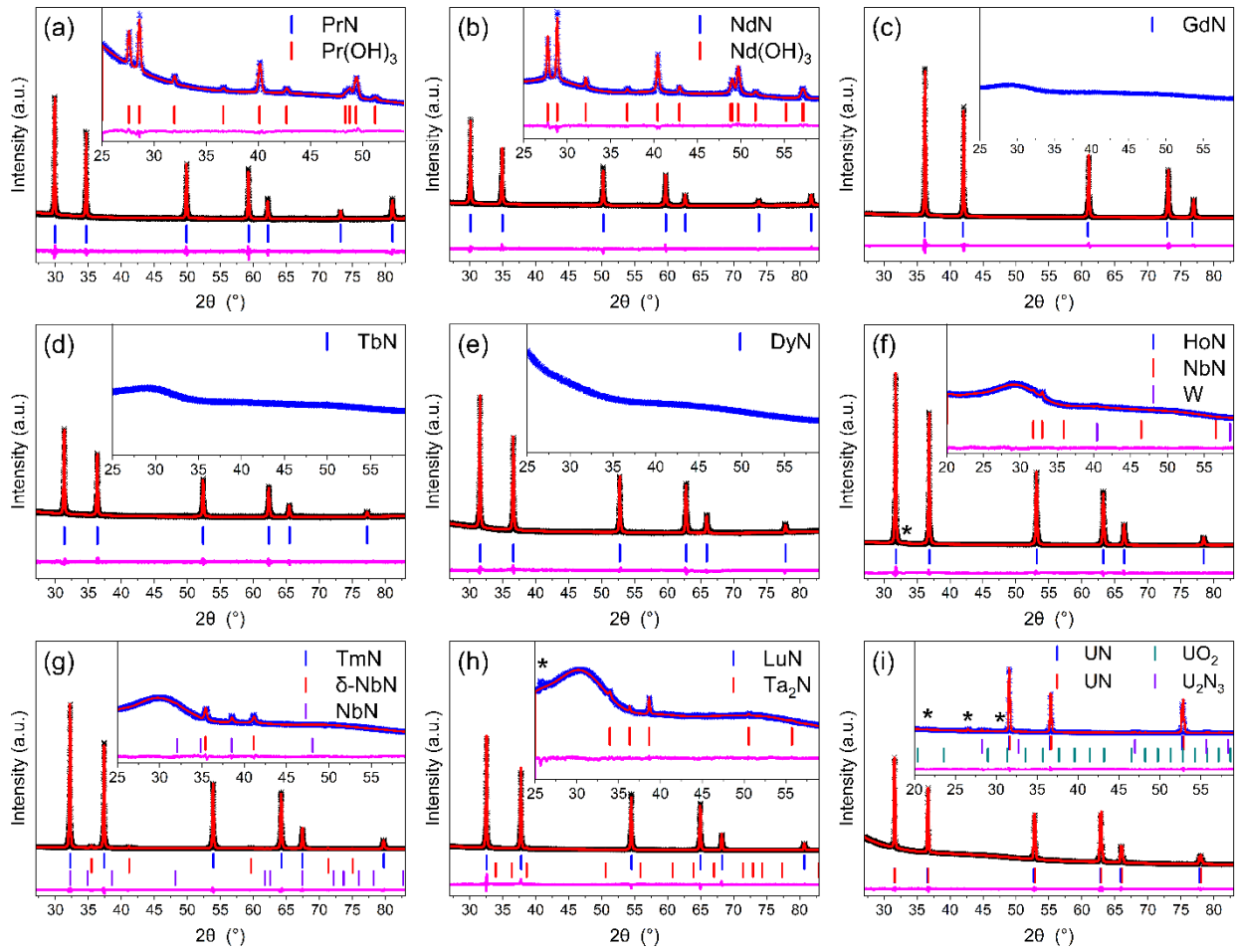
Figure 1: Rietveld profiles made against PXRD data of pristine LnN ( Ln = \text{Pr} (a), \text{Nd} (b), \text{Gd} (c), \text{Tb} (d), \text{Dy} (e), \text{Ho} (f), \text{Tm} (g), \text{Lu} (h)) and \text{UN} (i) phases. The insets provide corresponding Rietveld profiles for the same samples oxidised in air. The black and blue crosses correspond to
