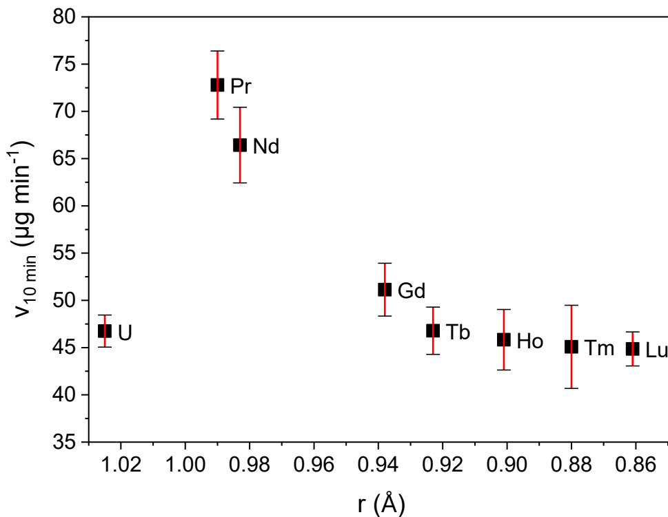
Figure 4. Oxidation rates of LnN ( Ln = \text{Pr, Nd, Gd, Tb, Ho, Tm, Lu} ) powders with < 100 \mu\text{m} particle size exposed to air for 10 minutes as function of their associated cation ionic radius, based on their reported ionic radii 30 when in a trivalent 6-fold coordination environment.
