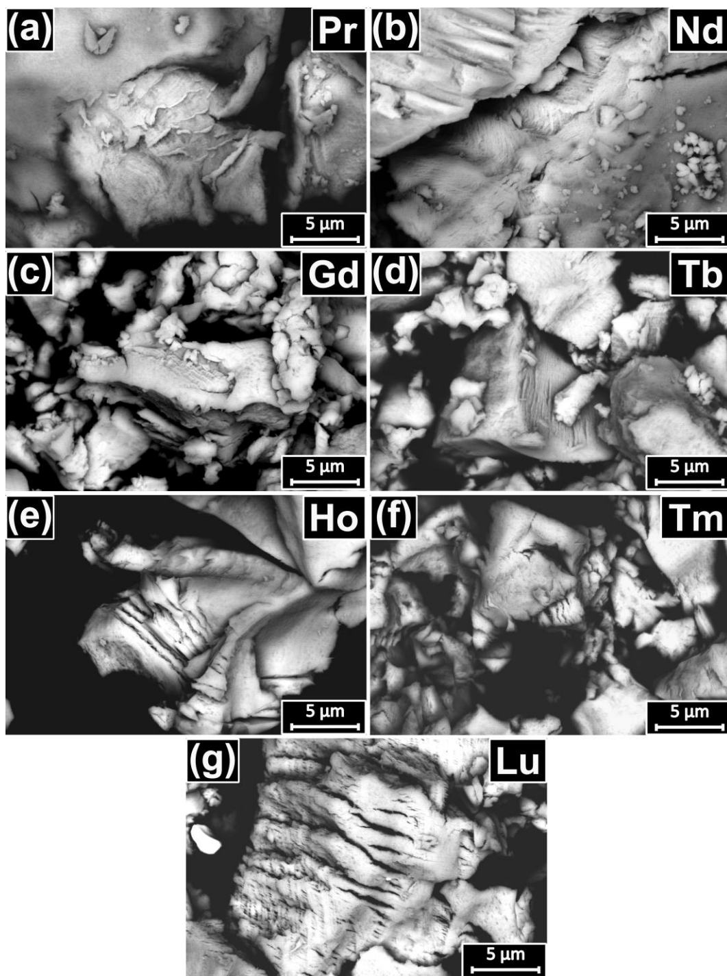
Figure 5. SEM-BSE images of Ln(OH)_3 ( Ln = \text{Pr} (a), \text{Nd} (b), \text{Gd} (c), \text{Tb} (d), \text{Ho} (e), \text{Tm} (f), \text{Lu} (g)) powders received by oxidation at ambient conditions of their respective LnN powders < 100 \mu\text{m} particle size in air, showing fibrous microstructures for all investigated powders.
