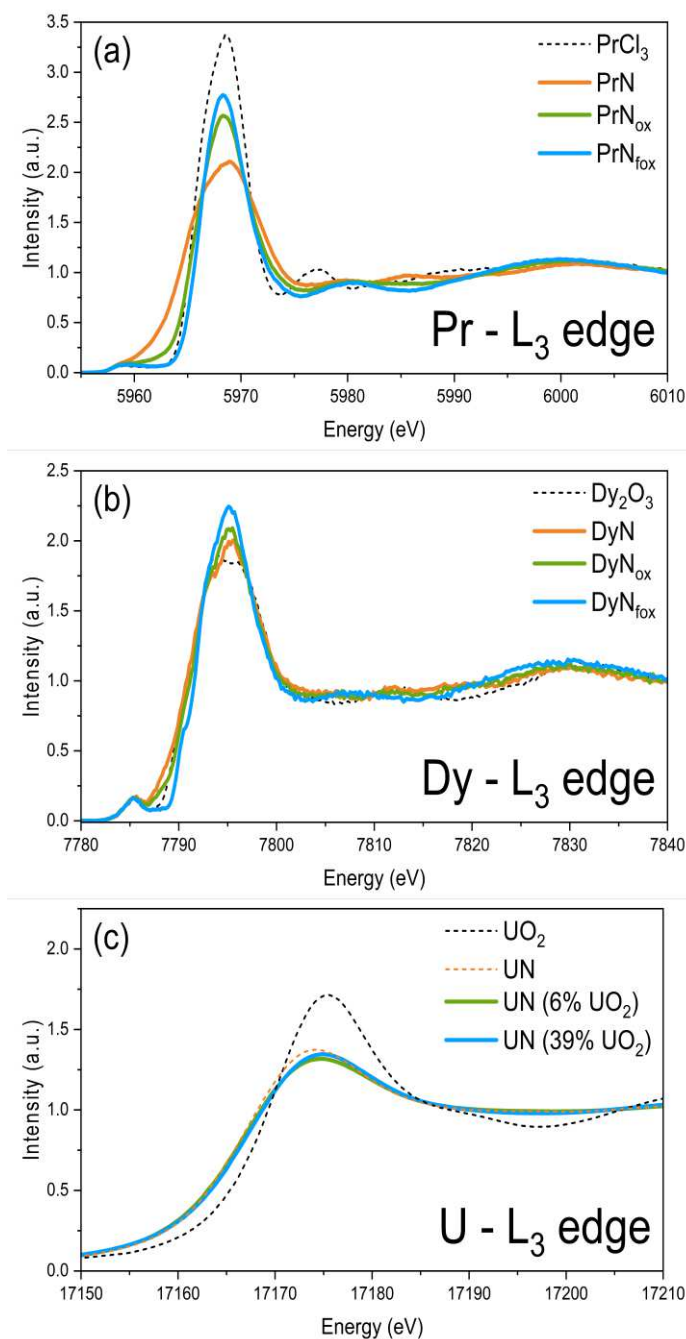
Figure 7. HR-XANES spectra (normalised to edge jump 1) of (a) at the Pr L 3 -edge for PrN, partially (ox) and full oxidised (fox) PrN samples with Pr +3 Cl 3 reference; (b) at the Dy L 3 -edge for DyN, partially (ox) and full oxidised (fox) DyN samples with Dy 2 +3 O 3 reference; (c) U L 3 -edge XANES spectra for UN samples containing 6.4 wt%/1.2 wt% and 38.8 wt%/1.5 wt% UO 2 /U 2 N 3 , and UO 2 and UN reference; respectively measured on the cation L 3 -edge.
