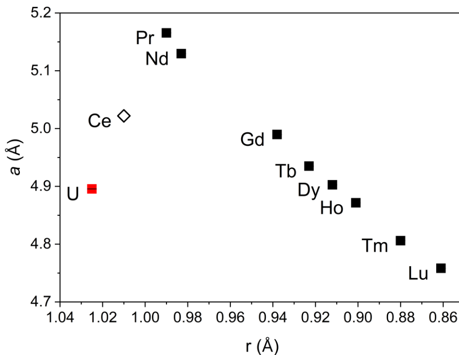
Figure 3. Lattice parameters as a function of ionic radii for the investigated UN and LnN compounds investigated based on their reported associated cation ionic radius 30,31 when in a trivalent 6-fold coordinated environment. Additionally CeN is plotted as reference from literature values. 32
