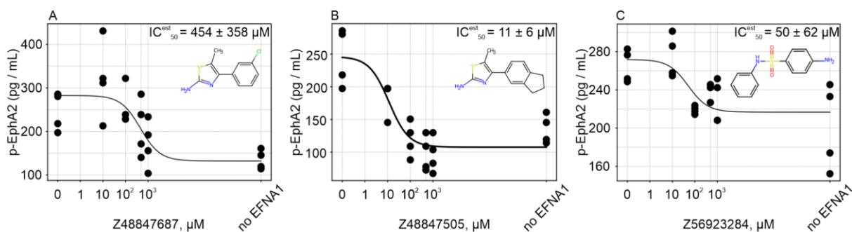
Figure S10. Quantitative analysis of the inhibitory activities of FBS hits and their derivatives. A, B, C) Dependencies of ELSA readout on ligand concentration in Figure 7 were approximated with eq (6) to determine the IC_{50} of the Z48847505, Z48847687, and Z56923284 compounds. (+) and (-) represent the positive (no inhibitor added) and negative (no ephrin A1 added) controls, respectively. The data is representative of 4 independent experiments ( n = 4 ).
