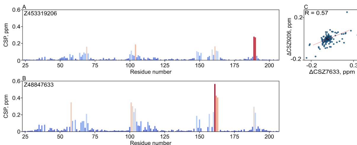
Figure S5. Binding modes of Z453319206 and Z48847633 according to the CSP data. A) ligand-induced CSPs in EphA2-LBD are plotted versus the residue number for the Z453319206 (A) and Z48847633 (B). Residues with high CSP have warm colors. C) Correlation between the CSPs induced by Z48847633 and by Z453319206. Pearson coefficient (R) is indicated.
