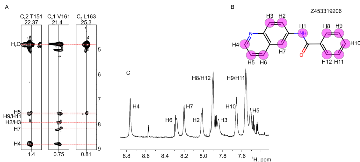
Figure S6. NMR data, reporting on the interaction between Z453319206 and EphA2 LBD. A) 2D strips of a 3D ^{15}\text{N}/^{13}\text{C} -filtered, ^{13}\text{C} -edited-NOESY-HSQC are indicated for the methyl group resonances of T151, V161, and L163. Assignments of the intermolecular cross-peaks are indicated. B) Structure of the compound with the chemical shift nomenclature. C) Fragment of a 1D ^{13}\text{C}/^{15}\text{N} -filtered-NOESY spectrum, containing the signals of Z453319206 with the indication of the assignments.
