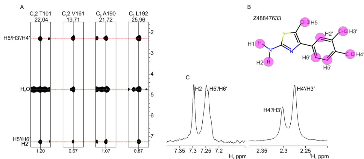
Figure S3. NMR data, characterizing the interaction between Z48847633 and EphA2 LBD. A) 2D slices of a 3D ^{15}\text{N}/^{13}\text{C} -filtered, ^{13}\text{C} -edited-NOESY-HSQC are indicated for the methyl group resonances of T101, V161, A190, and L192. Assignments of the intermolecular cross-peaks are indicated. B) Structure of the compound with the chemical shift nomenclature. C) Fragments of 1D ^{13}\text{C}/^{15}\text{N} -filtered-NOESY spectrum, containing the signals of Z48847633 with the indication of the assignments.
