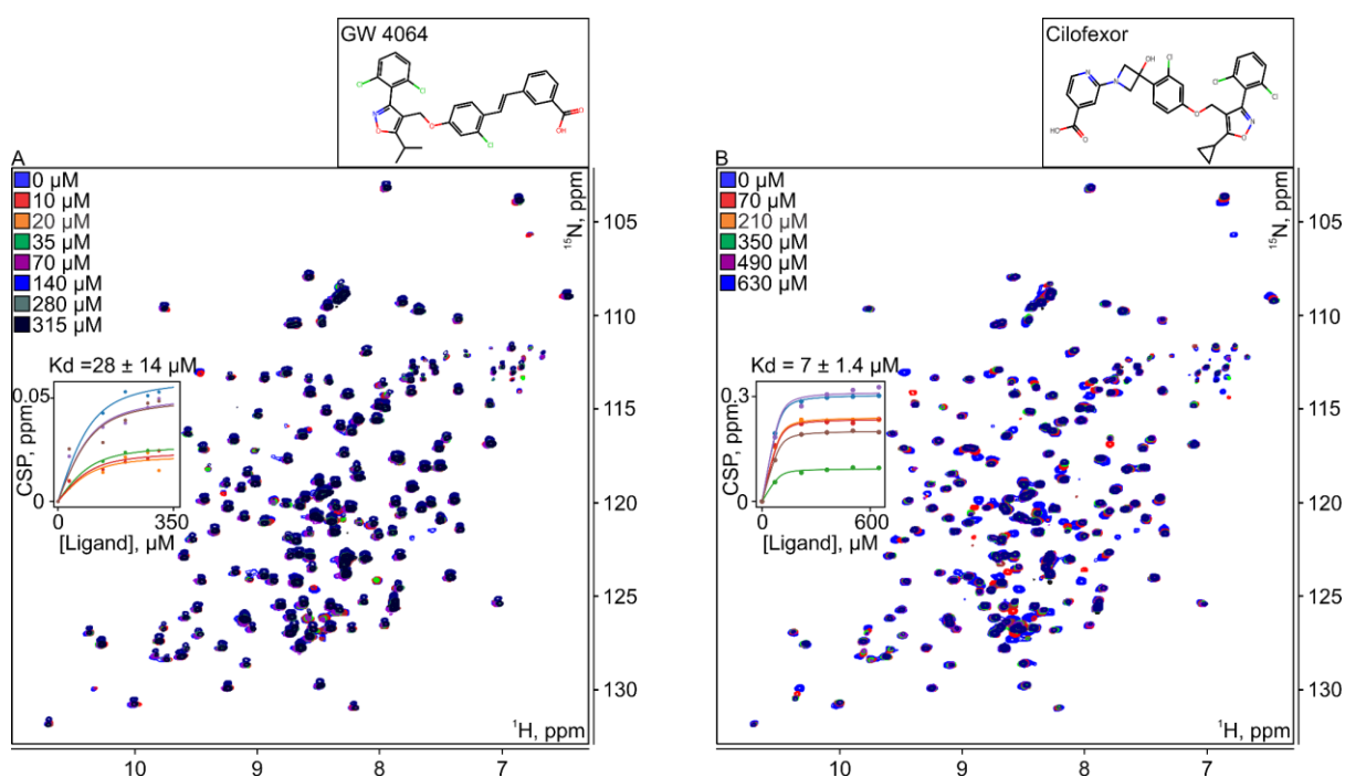
Figure S1. Binding of EphA2 LBD to the known ligands. A) Overlay of ^1\text{H} , ^{15}\text{N} -HSQC spectra of EphA2 LBD recorded in the presence of GW4064 at different concentrations: 0, 10, 20, 35, 70, 140, 280, 315 \mu\text{M} . The structure of GW 4064 is shown on the top of the panel. B) Overlay of ^1\text{H} , ^{15}\text{N} -HSQC spectra of EphA2 LBD recorded in the presence of Cilofexor at different concentrations: 0, 70, 210, 350, 490, 630 \mu\text{M} . The structures of GW 4064 and cilofexor are shown on the top of the panels. The CSP dependence on the ligand concentration is shown for 6 residues to estimate the K_D in A and B . Solid lines show the result of approximation of experimental data with the theoretical dependence (eq. (4))
