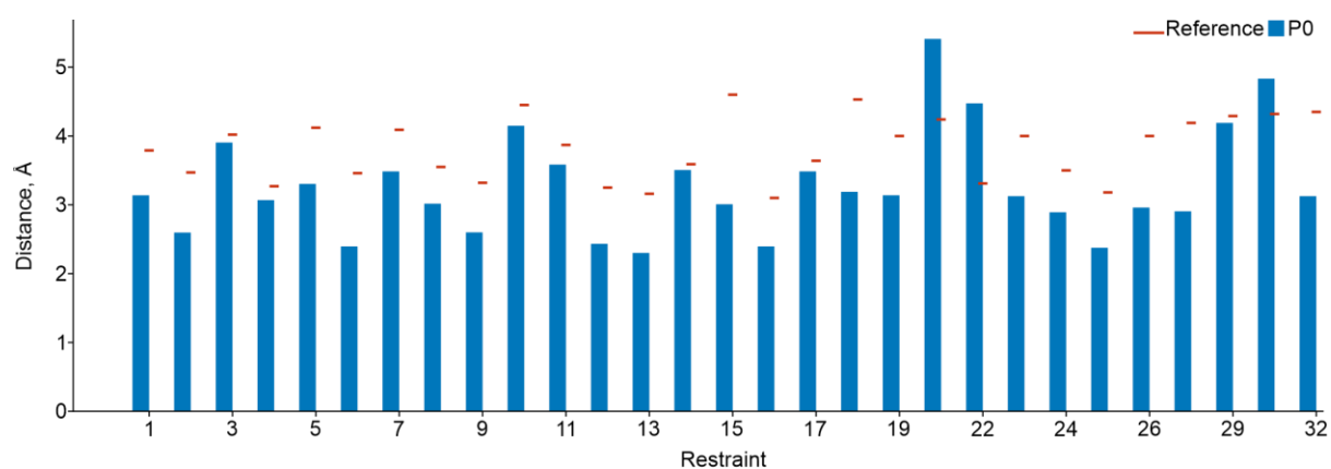
Figure S8. Comparison of MD simulation distances with the NMR restraints. Bars indicate the distances, corresponding to the each of the 32 peaks observed in the 3D ^{15}\text{N} , ^{13}\text{C} -filtered-NOESY-HSQC spectrum of Z48847633/EphA2 LBD complex. The distances were averaged over all MD trajectories. Red lines denote the NMR-derived distances for the peaks. Ambiguity of assignment is taken into account by averaging the sum of 1/r^6 of possible distances that can contribute to the respective NOE peak.
