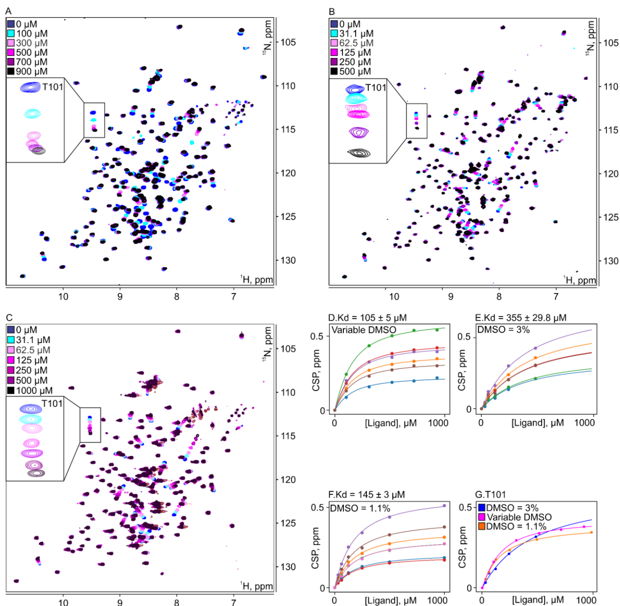
Figure S11. Effect of DMSO concentration on the affinity of Z48847633. A, B, C) Overlay of 2D ^1\text{H} , ^{15}\text{N} -HSQC spectra of EphA2 LBD recorded in the presence of Z48847633 at variable ( A ), 3% ( B ), 1.1% DMSO concentration ( D ). The concentrations of Z48847633 are indicated. The spectra were obtained at 100 \mu\text{M} of the protein in A and 50 \mu\text{M} in B and C , 298 K, pH 6.7. The close-up view of the T101 cross-peak is shown in a rectangle. D, E, F) The CSP dependence on the ligand concentration is shown for 6 residues to estimate the K_D in A , B , and C , respectively. Solid lines show the result of the approximation of experimental data with the theoretical dependence (eq. (4)). G) The overlay of CSP dependencies on the ligand concentration is shown for T101 in three different set-ups.
