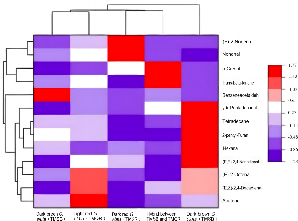
Supplementary figure 6. Cluster analysis of 13 volatile compounds detected by gas chromatography-mass spectrometry (GC-MS) in various germplasms of Gastrodia elata . The x-axis is the Gastrodia elata sample, and the y-axis is the name of the volatile compound. The label on the right indicates the relative content of each volatile compound, with blue representing low relative content and red representing high relative content.
