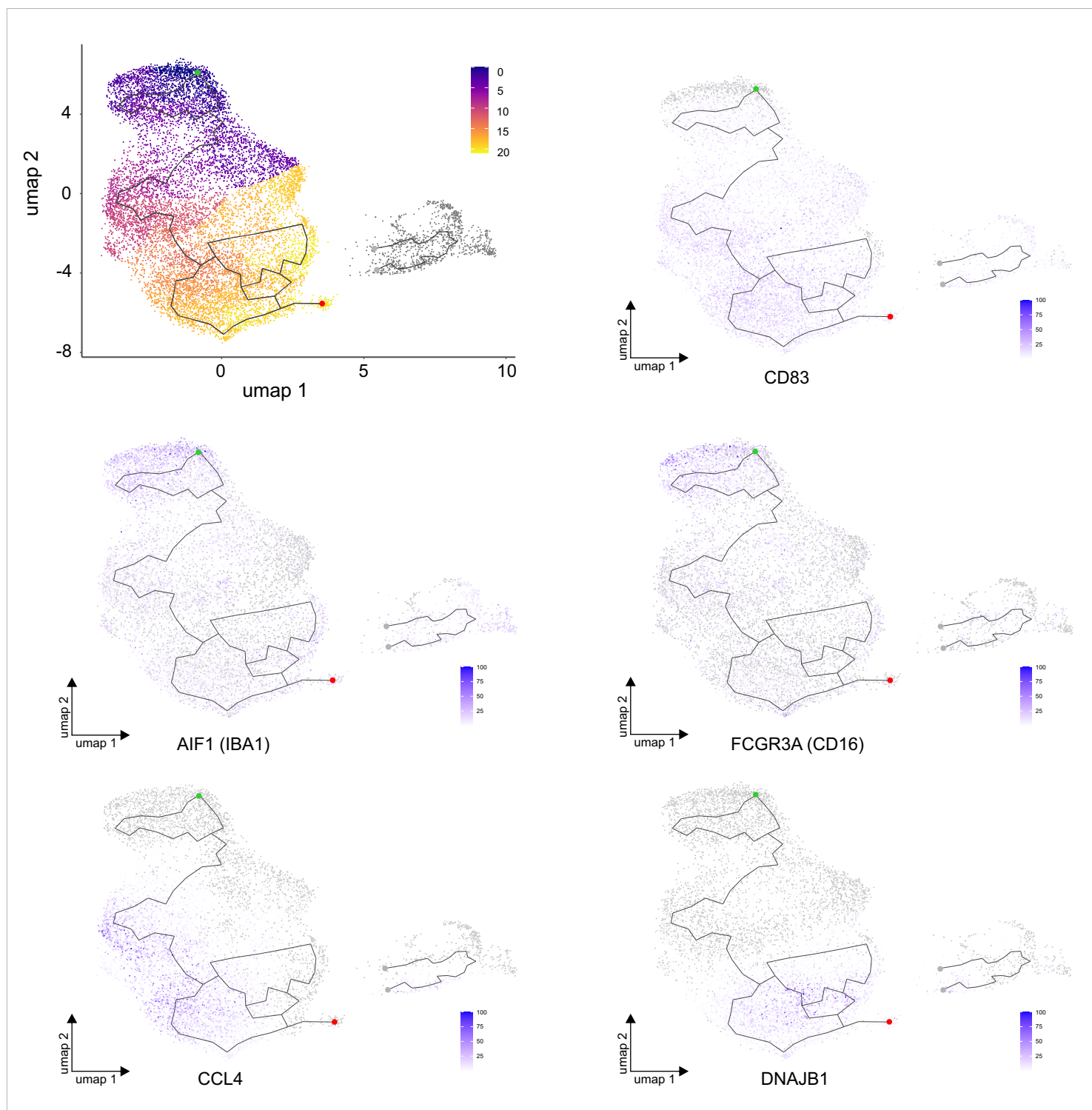
Fig. S10: Trajectory analysis to show the potential connectedness of microglia clusters. Feature plots show the normalized expression (expressed as a percentage) of genes that best define different transitional subpopulations (see also Fig. 6F).
