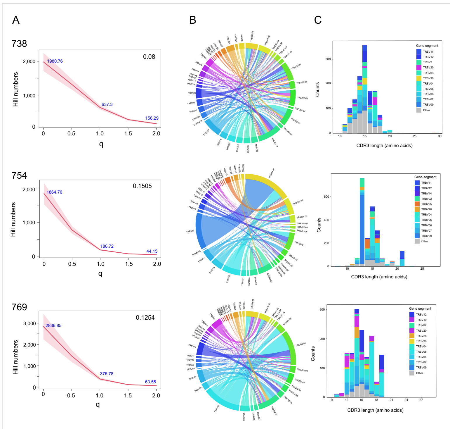
Fig. S8: (A) Hill plots showing that the diversity of T cell clonotypes in the brain surgical specimens is lowest in patient 754 and highest in patient 738 reflecting a higher clonality in patient 754 compared with patient 738 (clonality score in the top right corner of each graph). (B) Chord plots show TRBV and TRBJ gene usage is demonstrably skewed in the surgical specimens from patient 754 and patient 769. (C) Frequency histograms of Vbeta chain CDR3 lengths color coded for the proportion of frequent TRBV genes confirms the expansion of specific clonotypes (see also Table S1).
