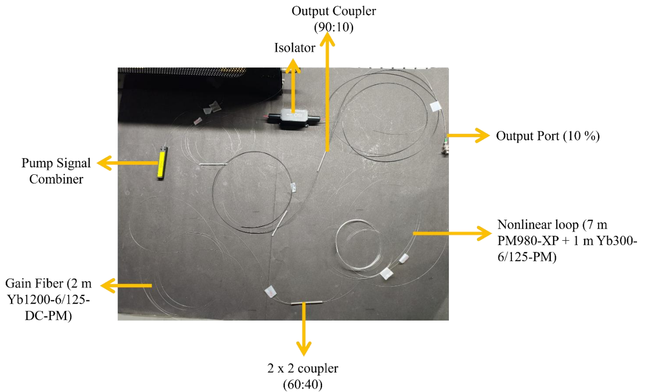
Figure 1: Setup of NAbLM based Figure of 8 Laser Oscillator (when pump is OFF)
