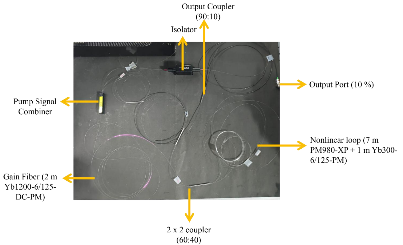
Figure 2: Setup of NAbLM based Figure of 8 Laser Oscillator (when pump is ON)
