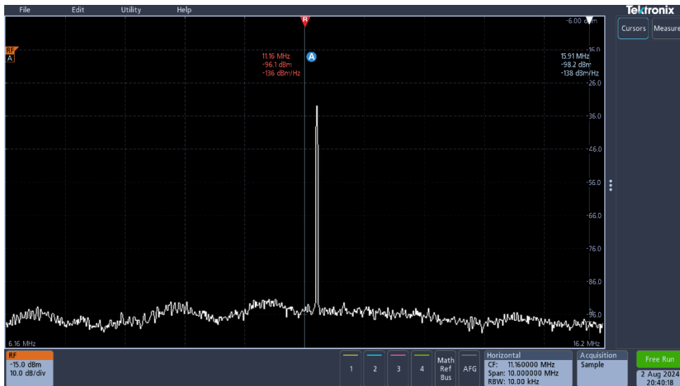
Figure 4: RF Spectrum of the output
