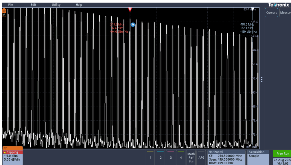
Figure 5: RF Spectrum of the output for 500 MHz span
