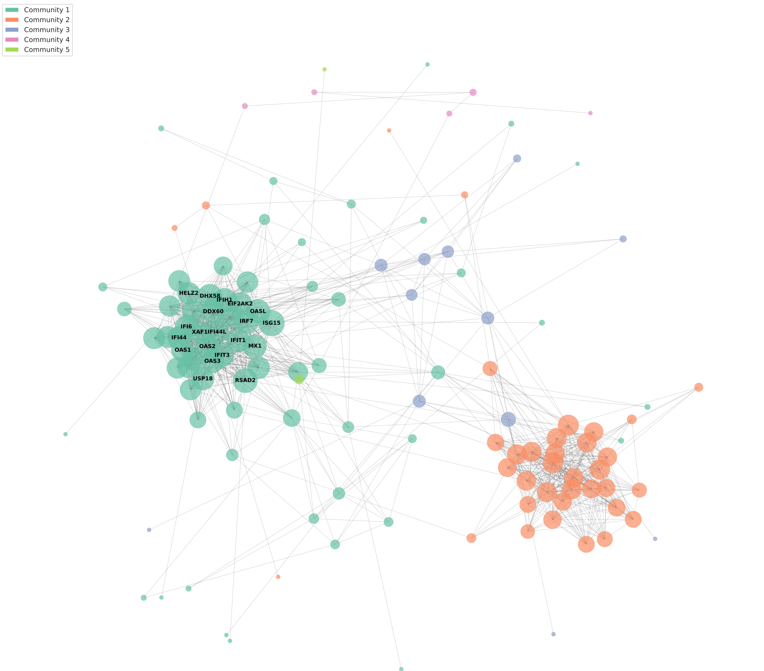
PPI Network of Top 200 DEGs in COVID-19 Colored by Community, Sized by Degree Centrality
